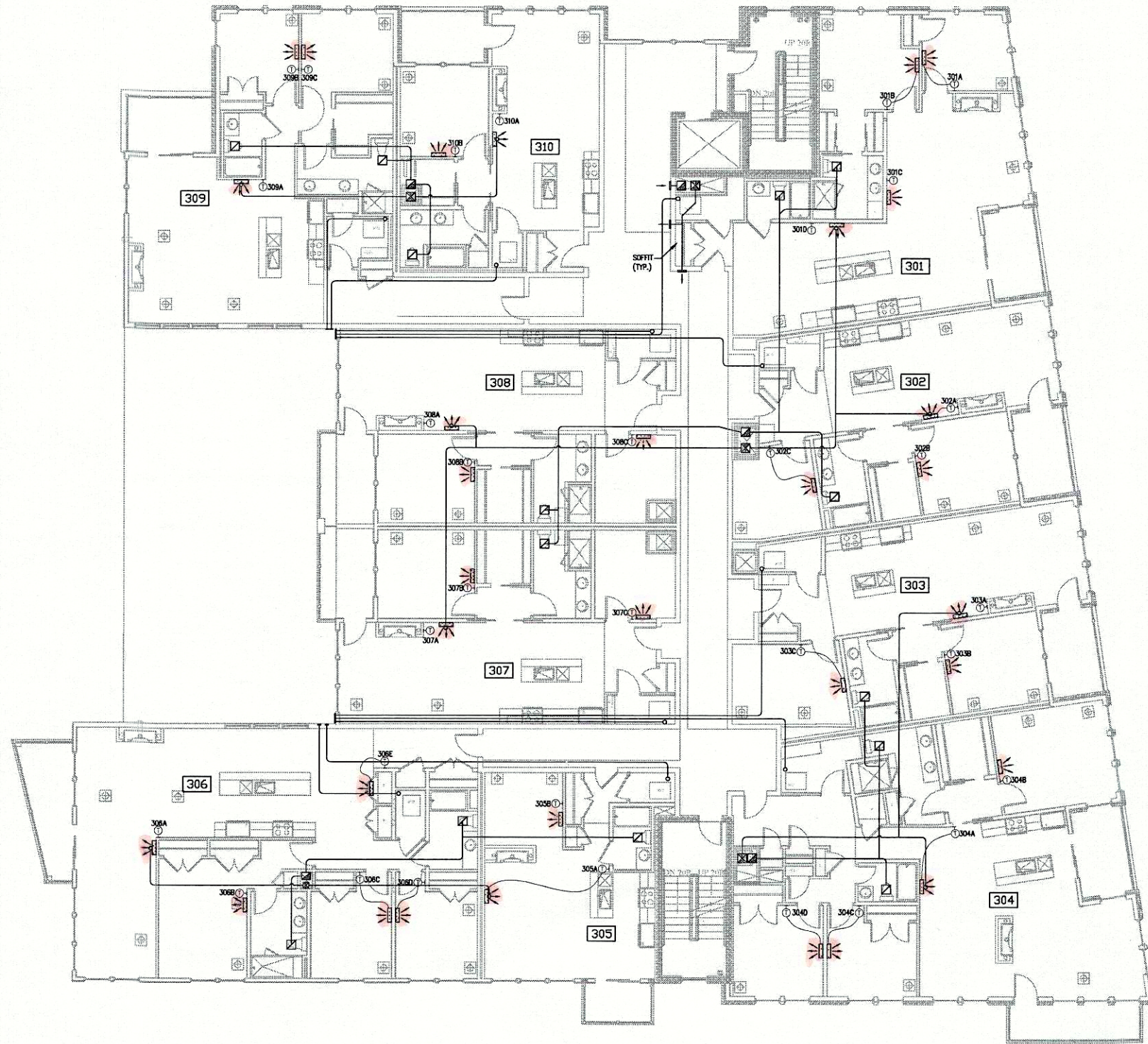
THIRD FLOOR - DUCTWORK SCALE: 1/8"=1'-0"
