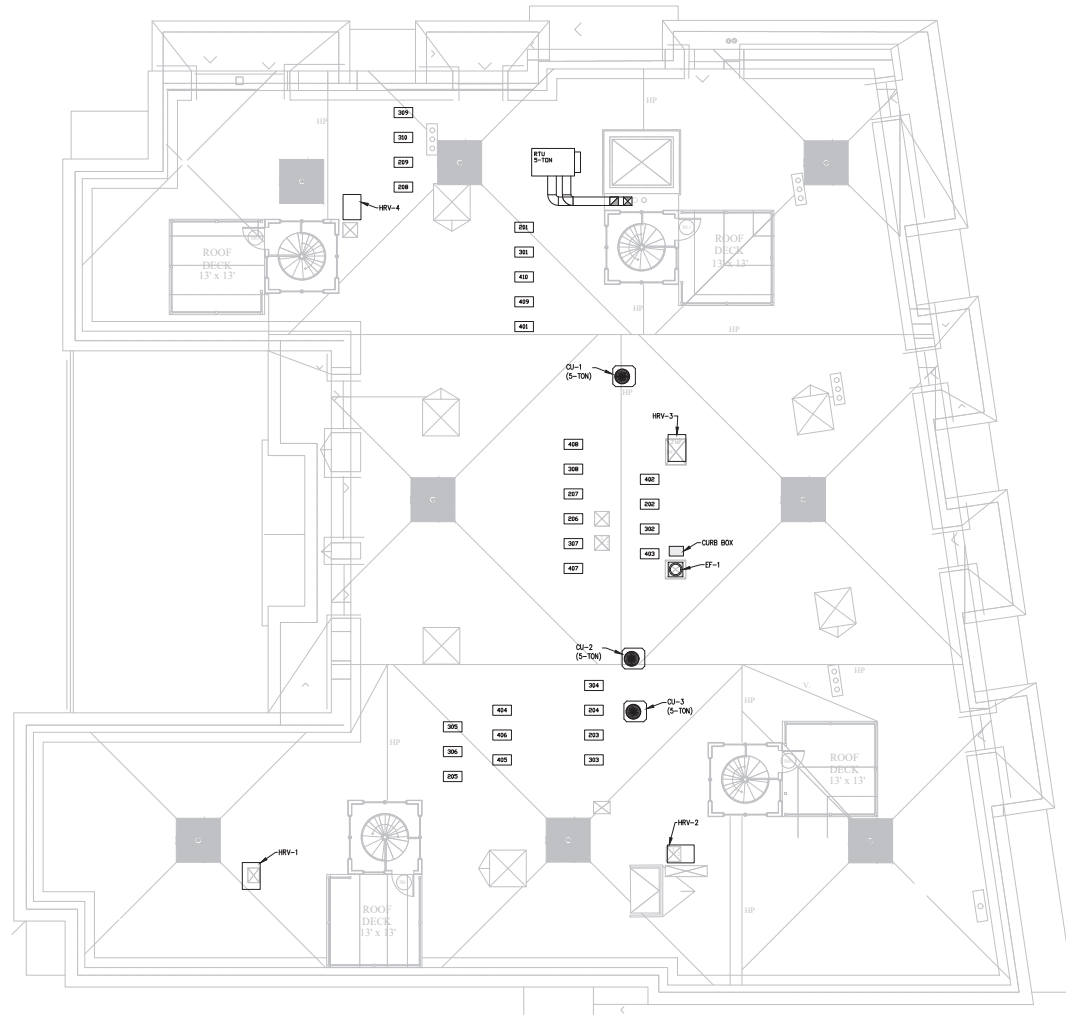
ROOF — DUCTWORK SCALE: 1/8"=1'-0"
