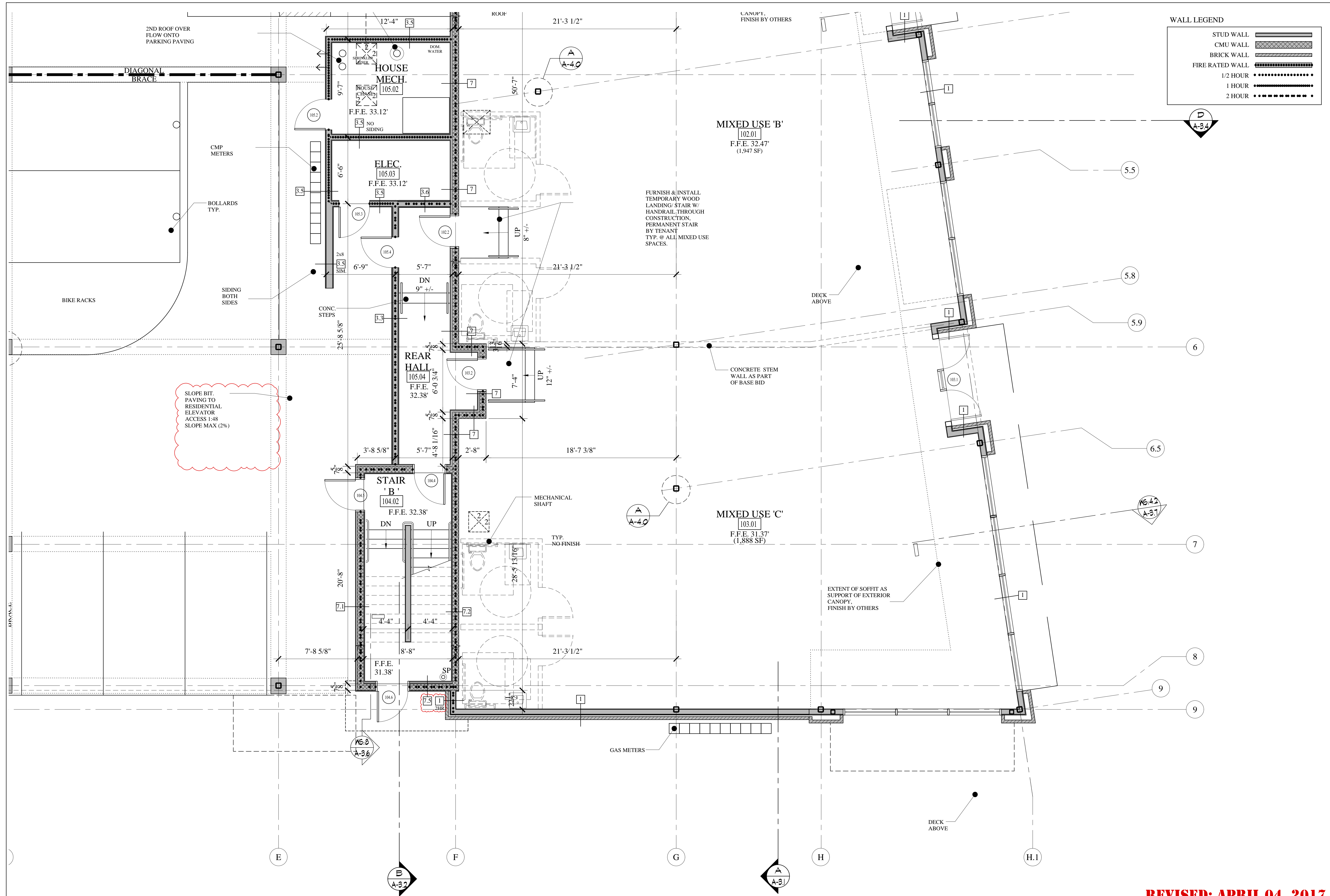
PARTIAL FIRST FLOOR PLAN 'B' SCALE: 1/4"=1'-0"
