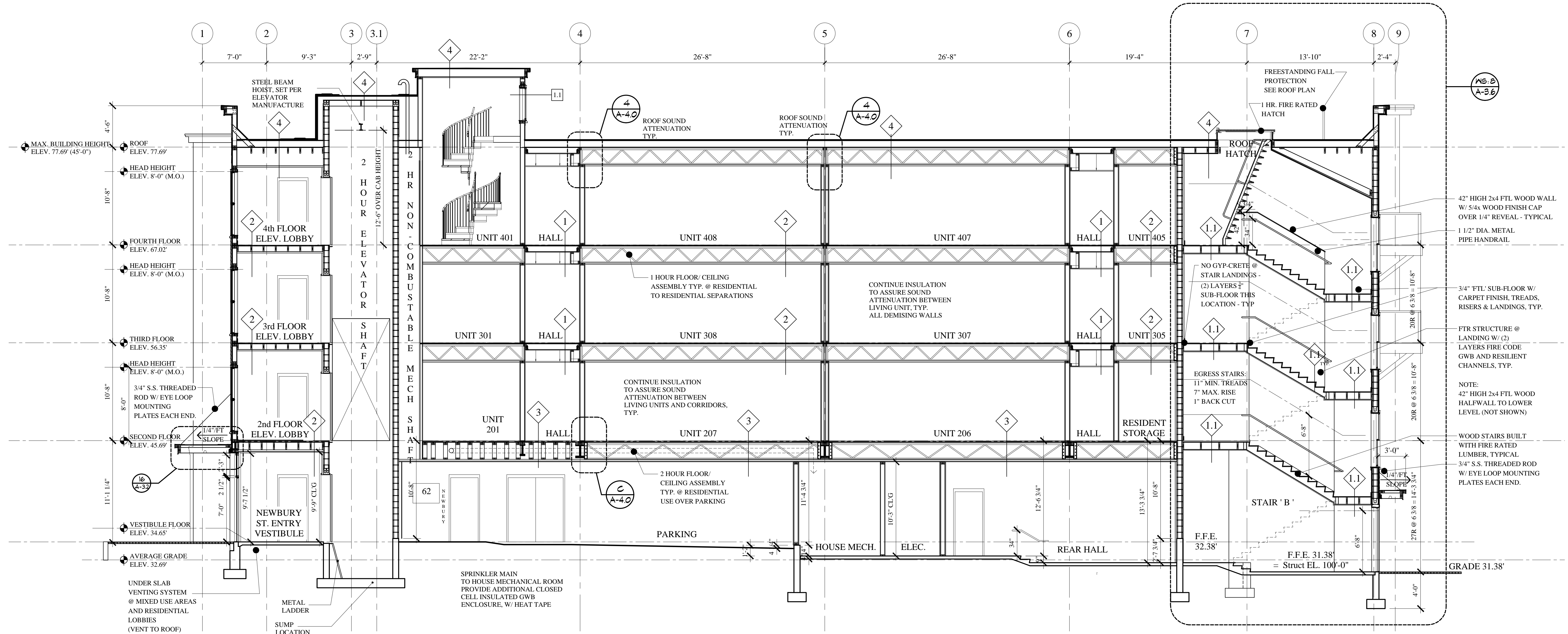
B BUILDING SECTION A-1.3 SCALE: 3/16" = 1'-0"
