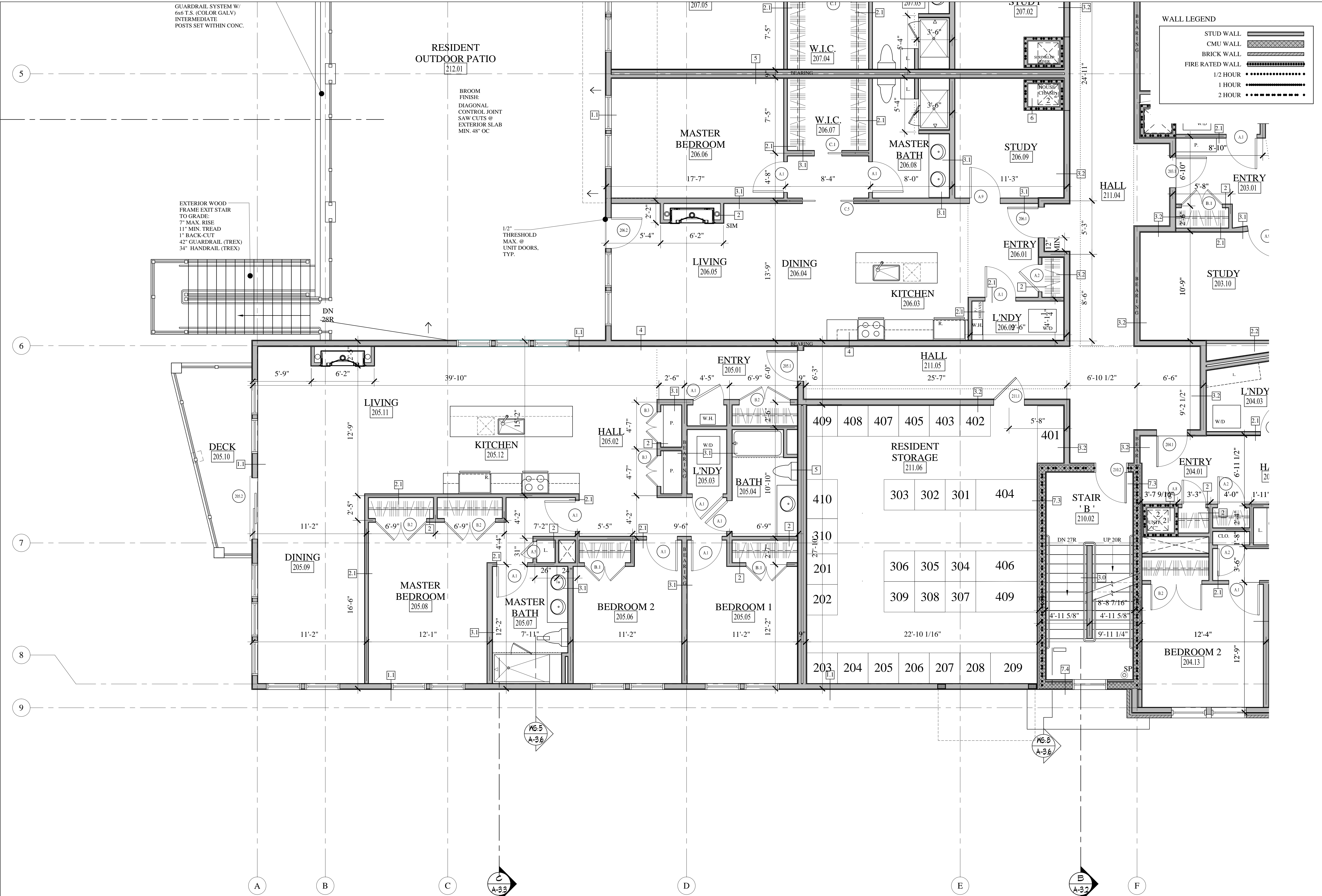
PARTIAL SECOND FLOOR PLAN 'C' SCALE: 1/4"=1'-0"
