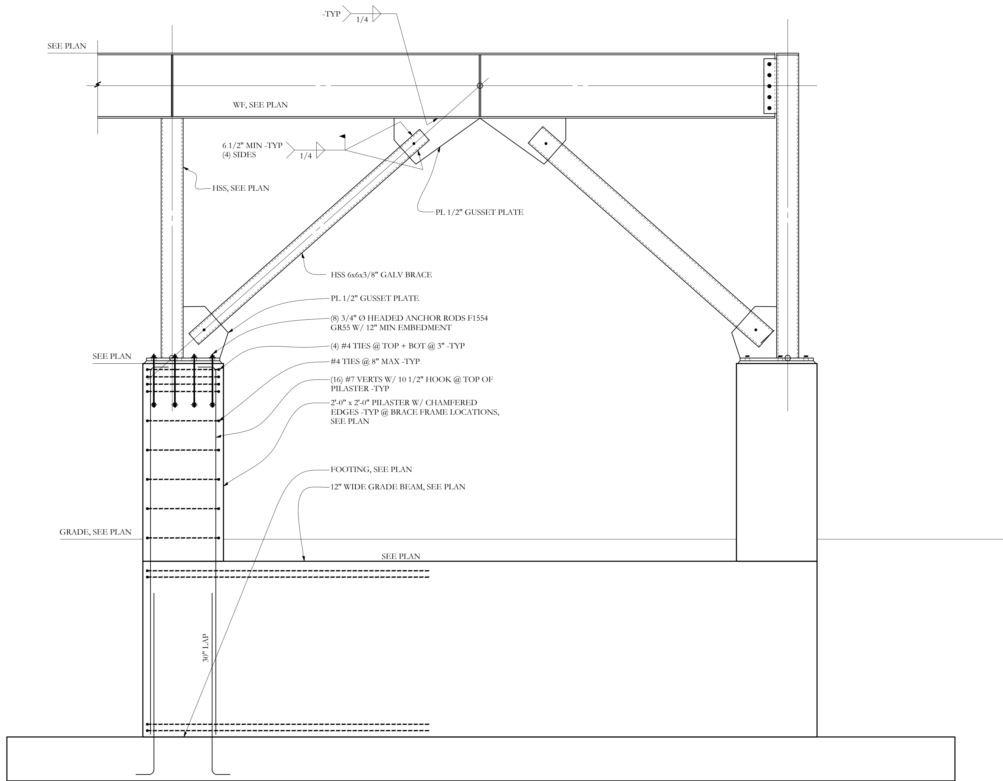
SECTION MM S-2.4 3/4"=1'-0
