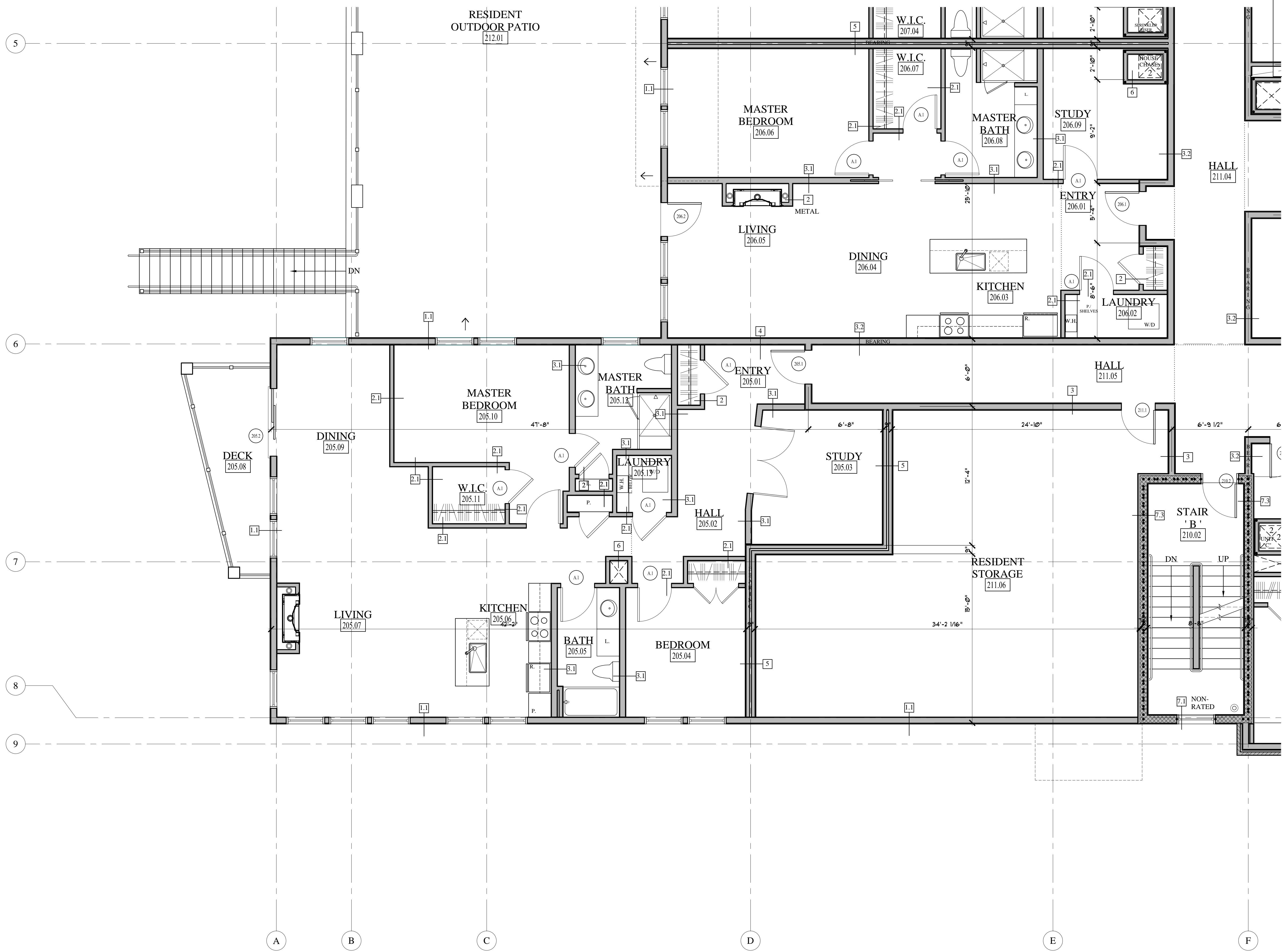
PARTIAL SECOND FLOOR PLAN ' B ' SCALE: 1/4"=1'-0"
