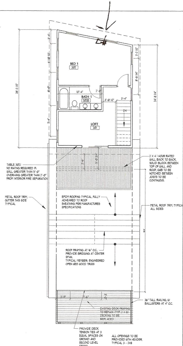
1 2 3 3RD LEVEL SCALE: 1/4" = 1'-0"
