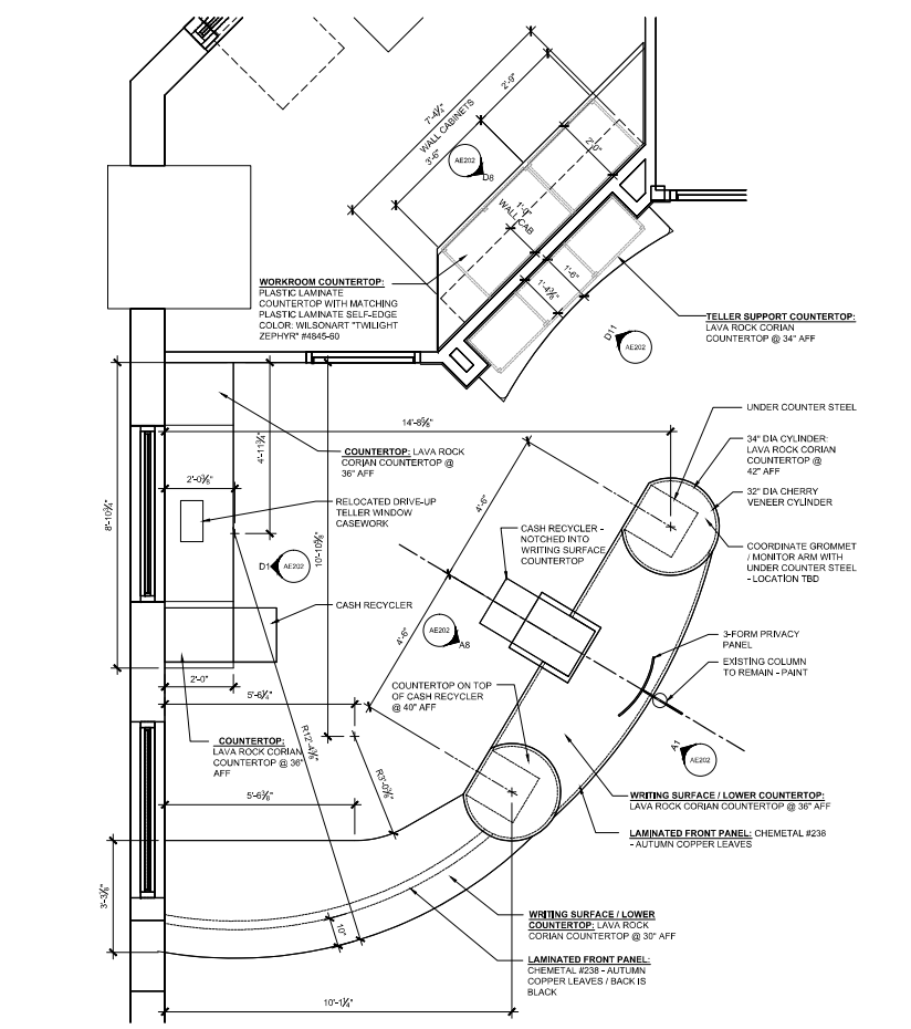
A4 ENLARGED TELLER CASEWORK PLAN 1/2" = 1'-0"
