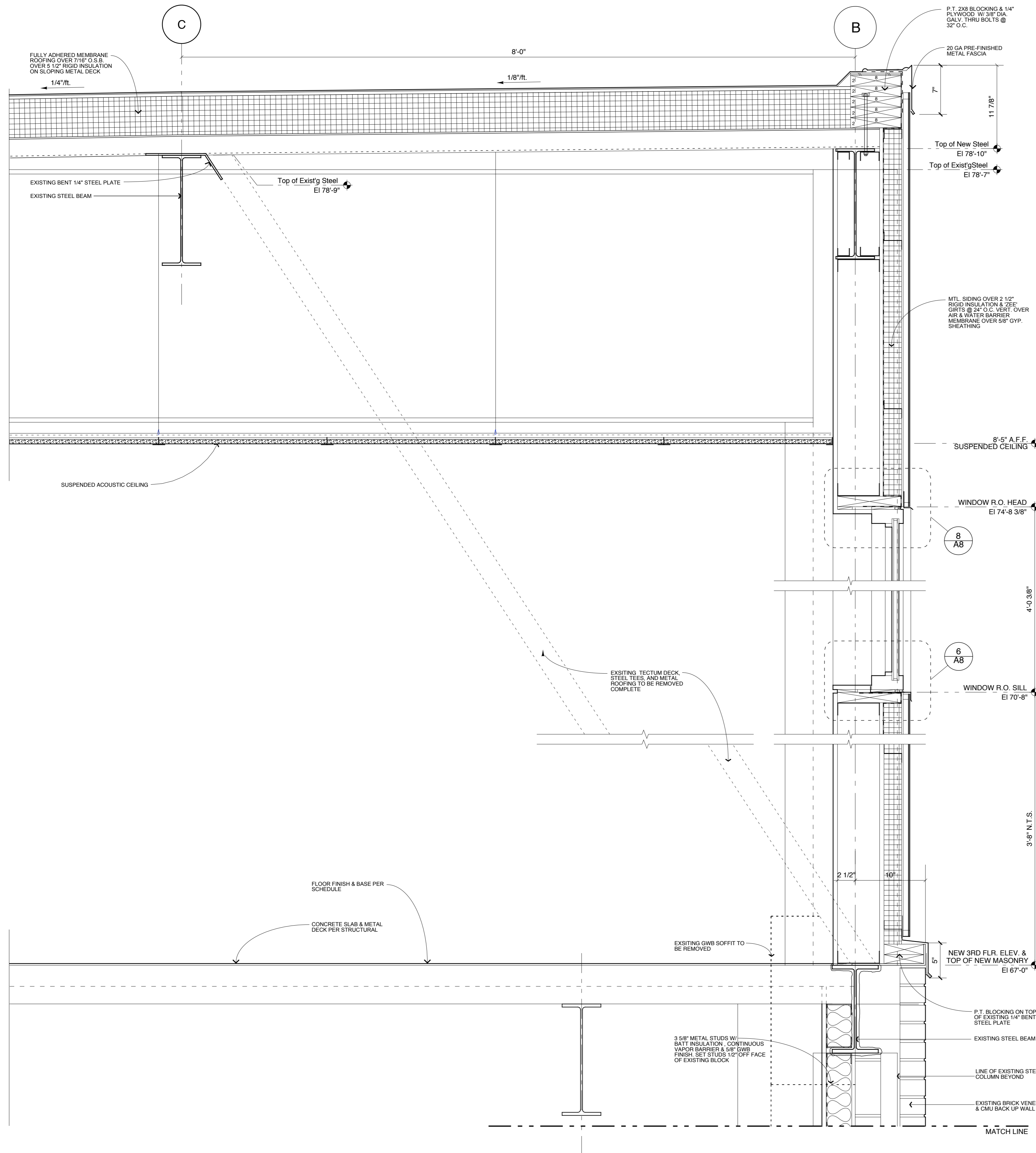
4 WALL SECTION AT 'B' LINE 1/2" = 1'-0"
