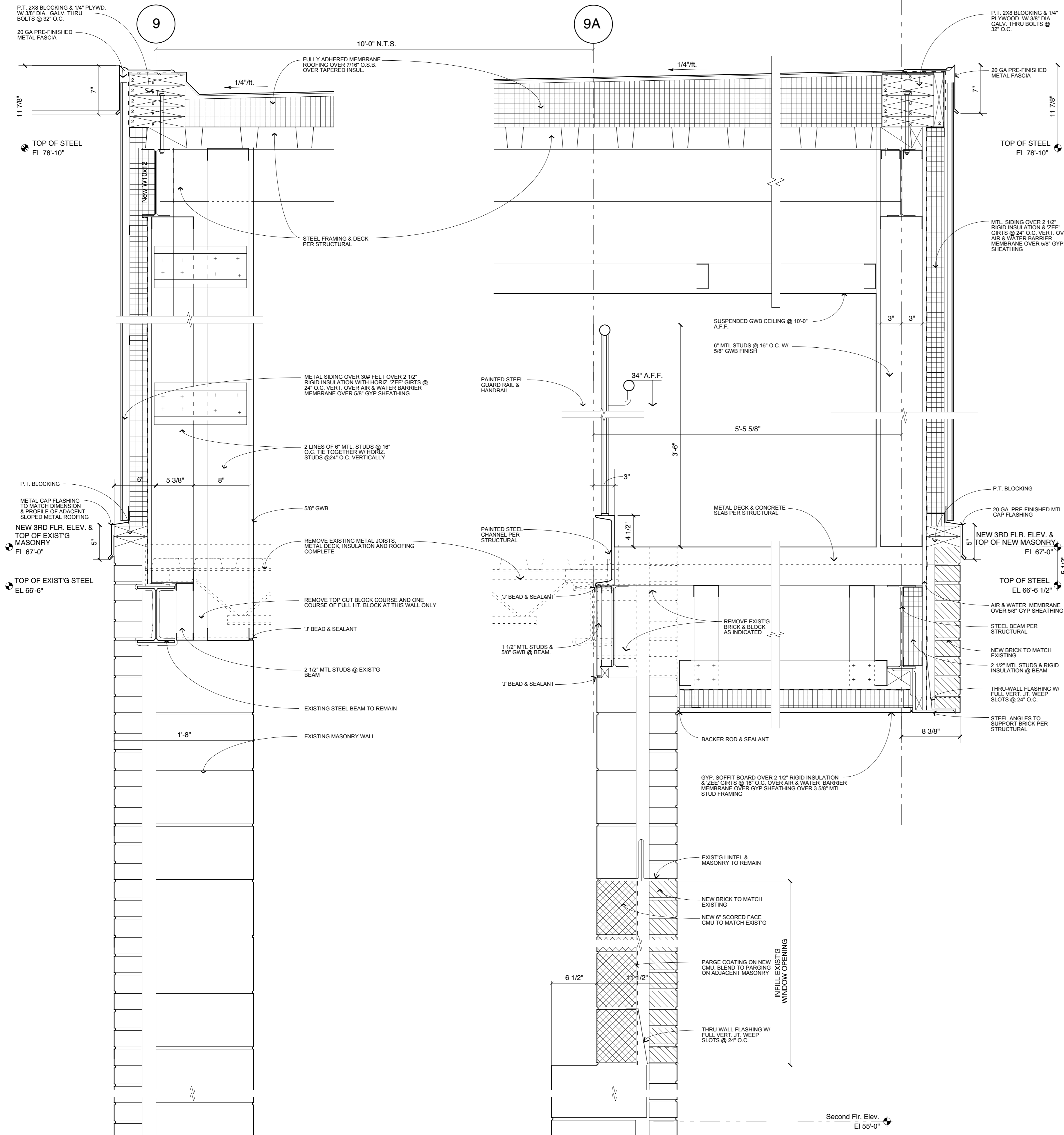
1 WALL SECTION AT STAIR 1 1/2" = 1'-0"
