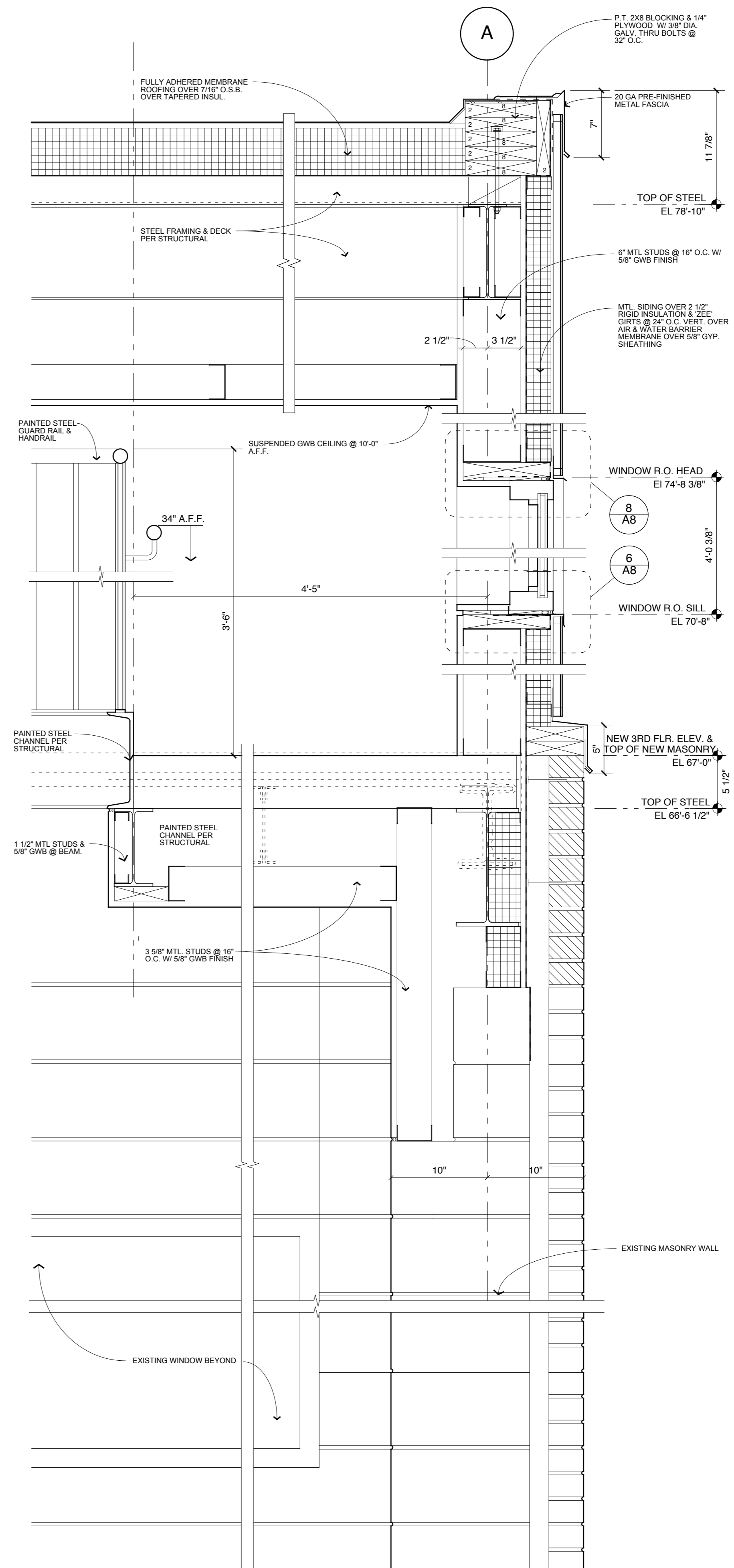
3 WALL SECTION AT STAIR 1 1/2" = 1'-0"
