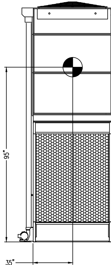
Air Inlet Side
