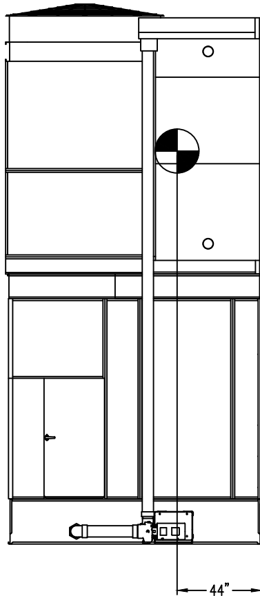
Connection End
