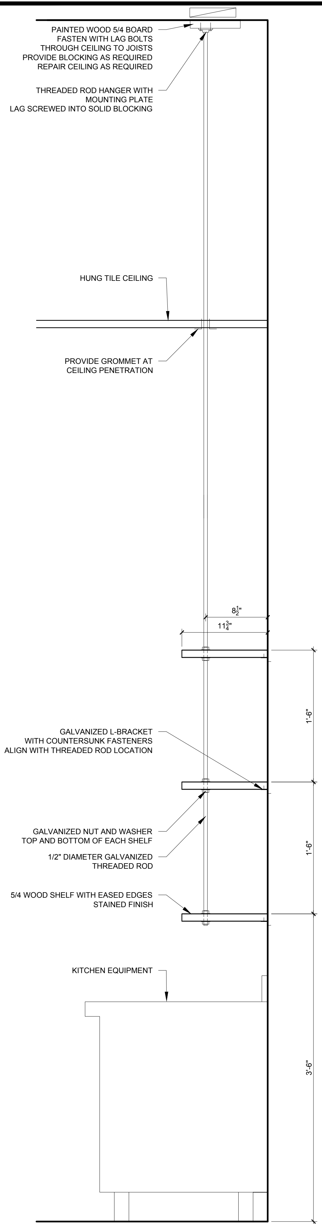
2 BACK BAR SHELVING SECTION DETAIL 1/12" = 1'-0"
