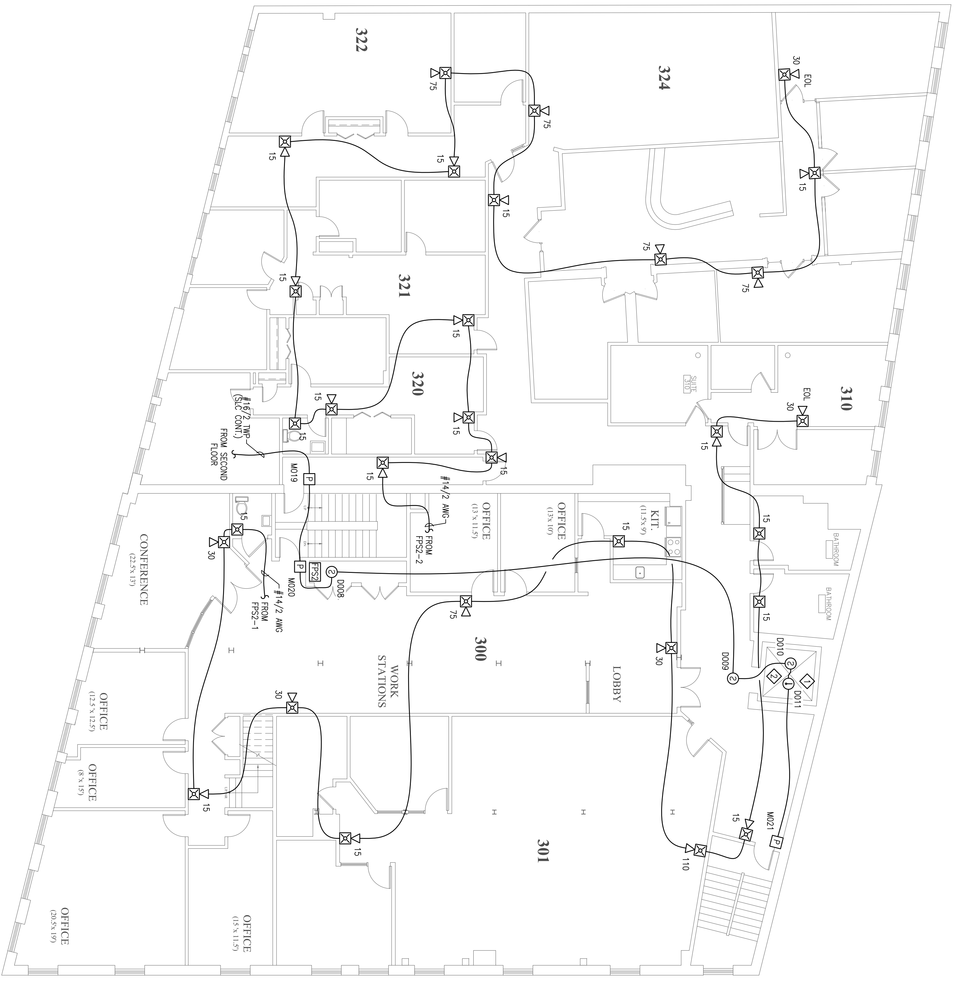
THIRD FLOOR FIRE ALARM PLAN SCALE: 1/8"=1'-0"
