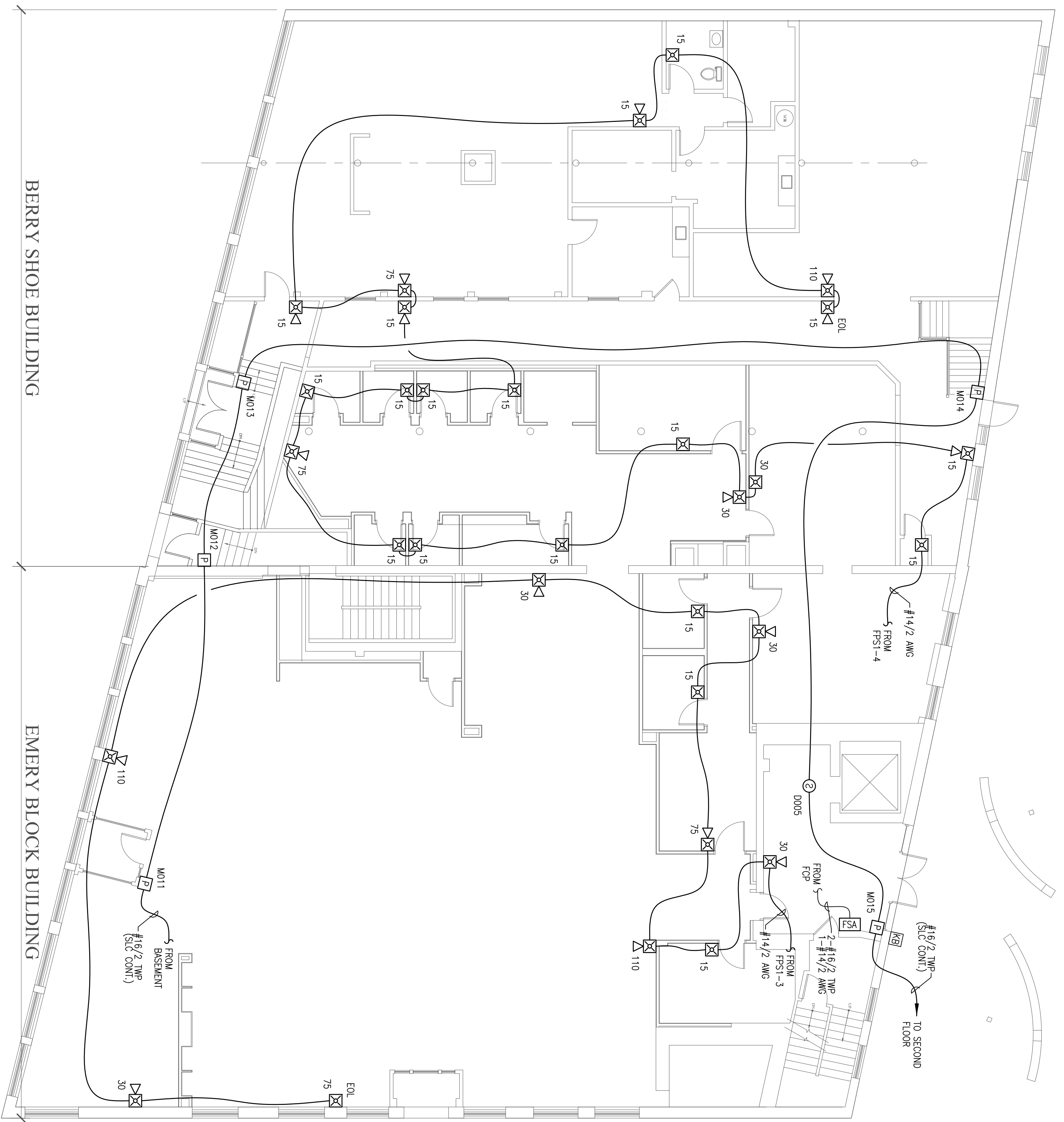
FIRST FLOOR FIRE ALARM PLAN SCALE: 1/8"=1'-0"
