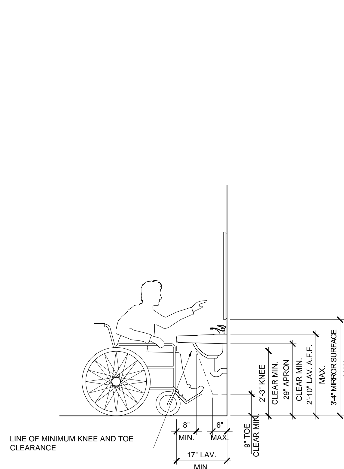
10 TYPICAL ADA CLEARANCES
