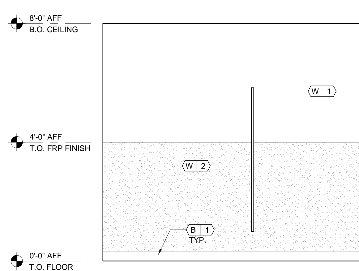
2 INTR ELEVATION - WOMEN'S TOILET ROOM
