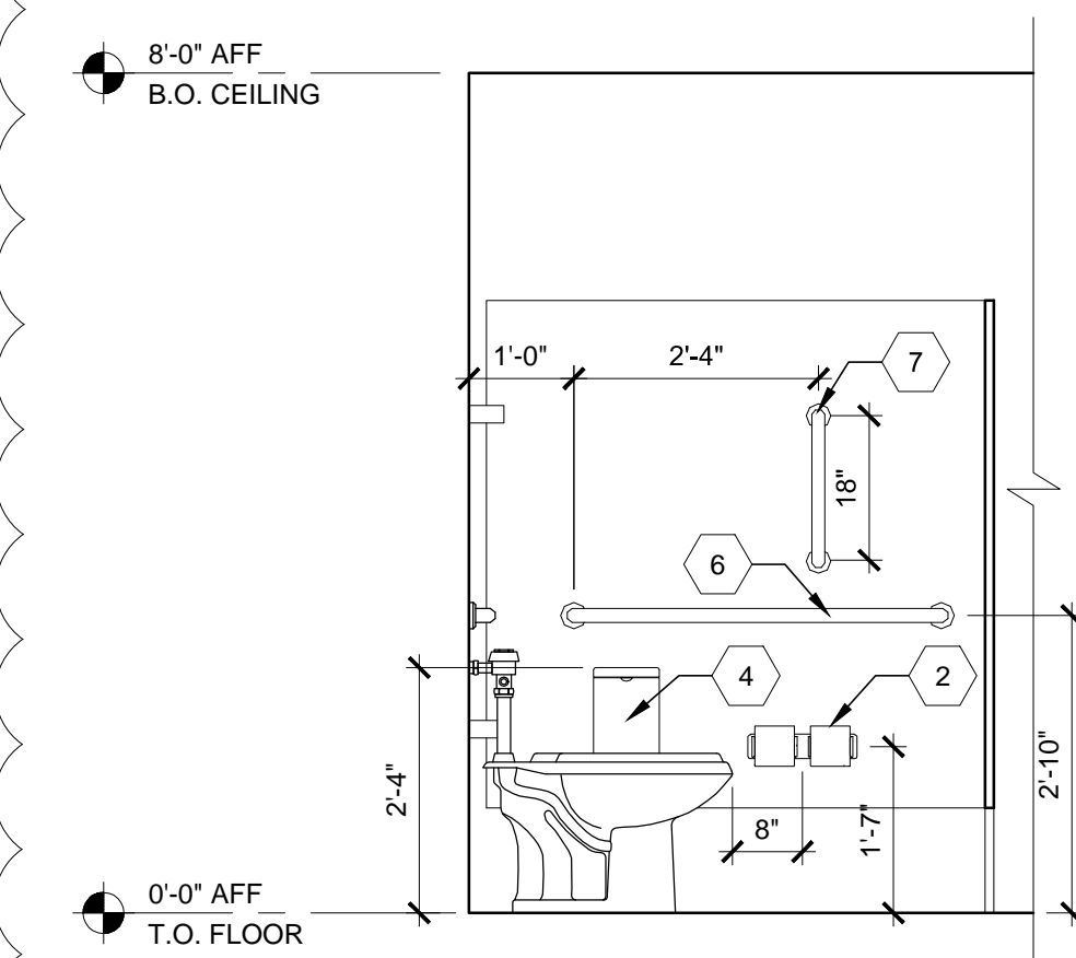
10 INTR ELEVATION - MEN'S TOILET ROOM
