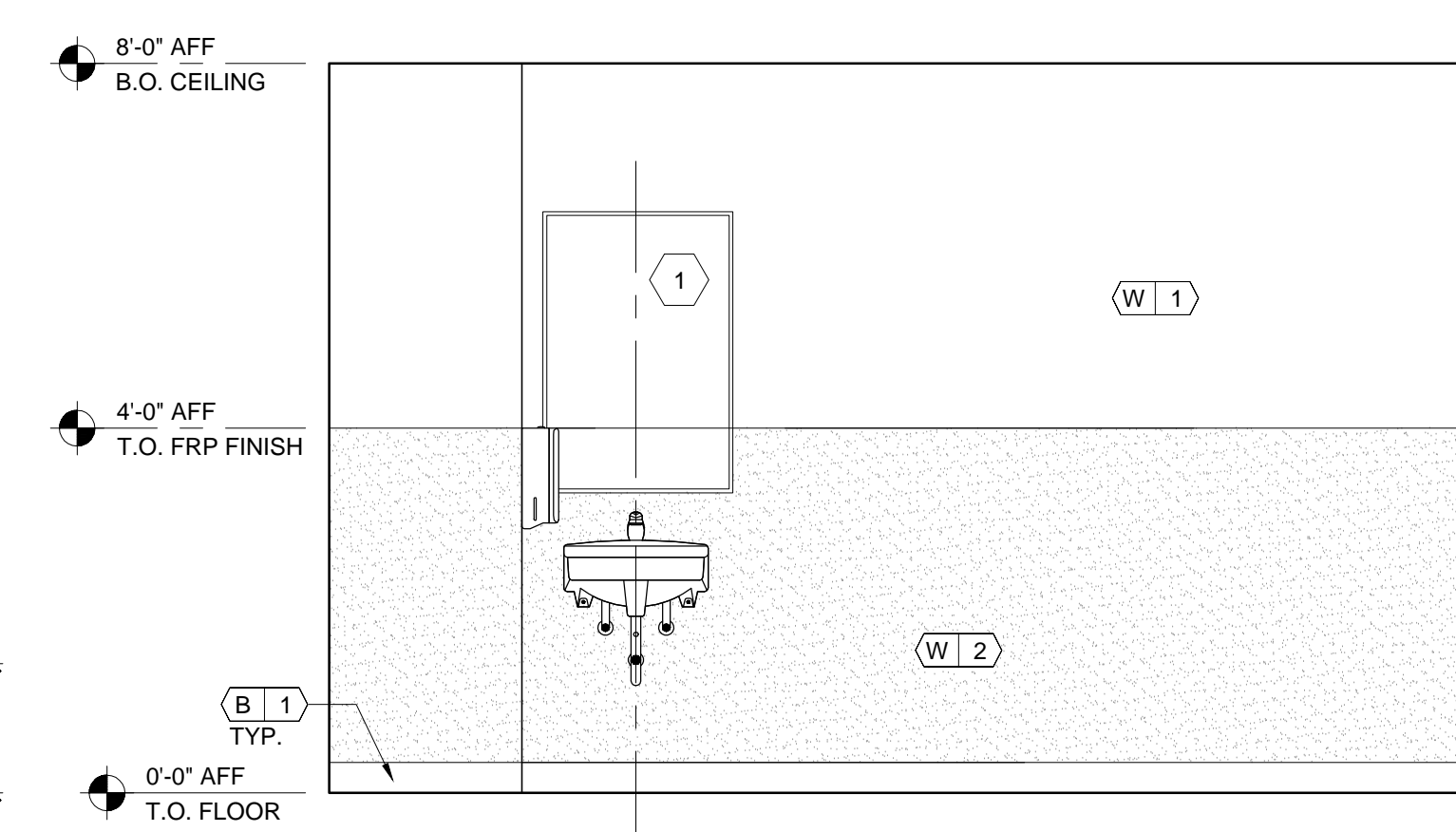
7 INTR ELEVATION - MEN'S TOILET ROOM
