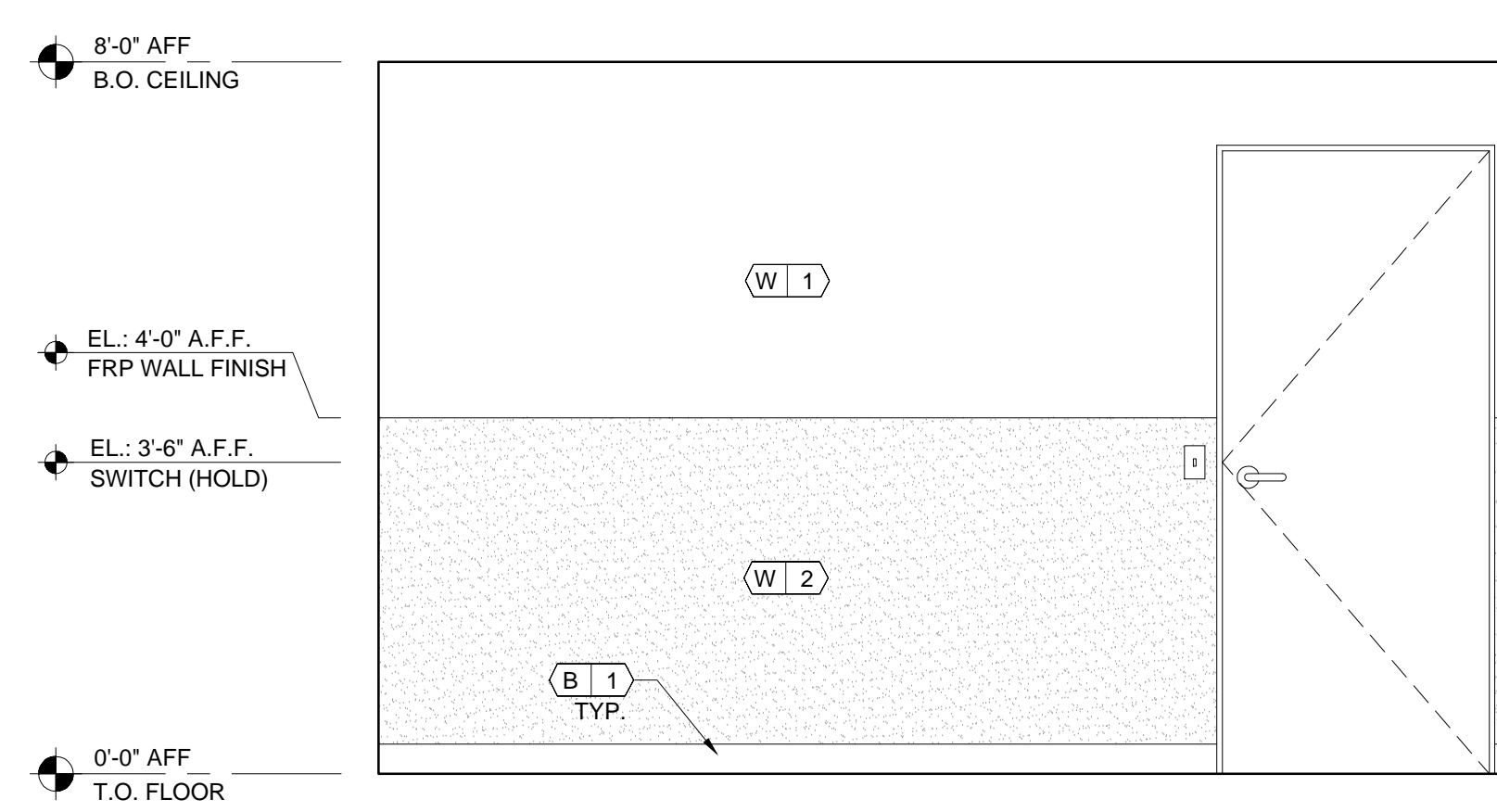
9 INTR ELEVATION - MEN'S TOILET ROOM
