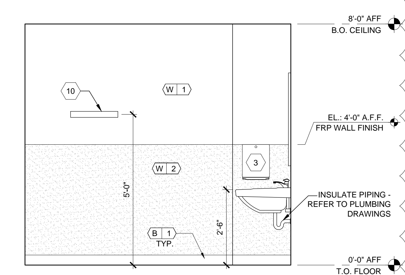
6 INTR ELEVATION - MEN'S TOILET ROOM
