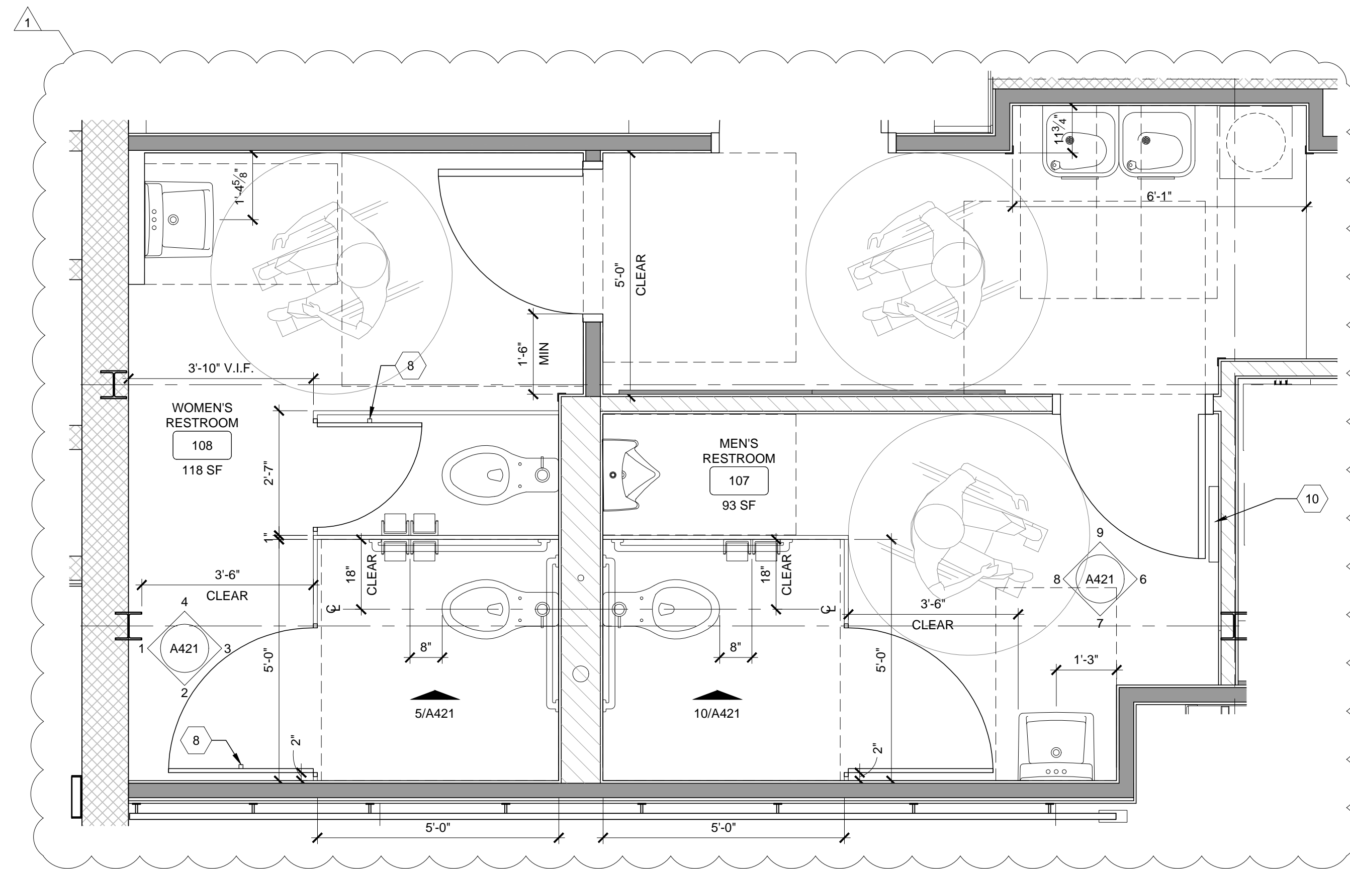
9 ENLARGED TOILET ROOM PLANS
