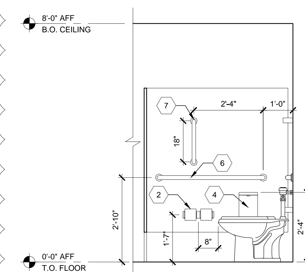
5 INTR ELEVATION - WOMEN'S TOILET ROOM
