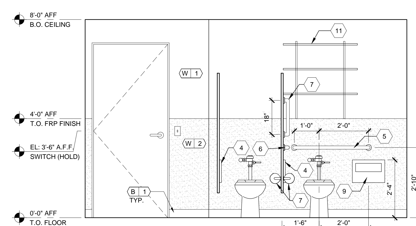
3 INTR ELEVATION - WOMEN'S TOILET ROOM
