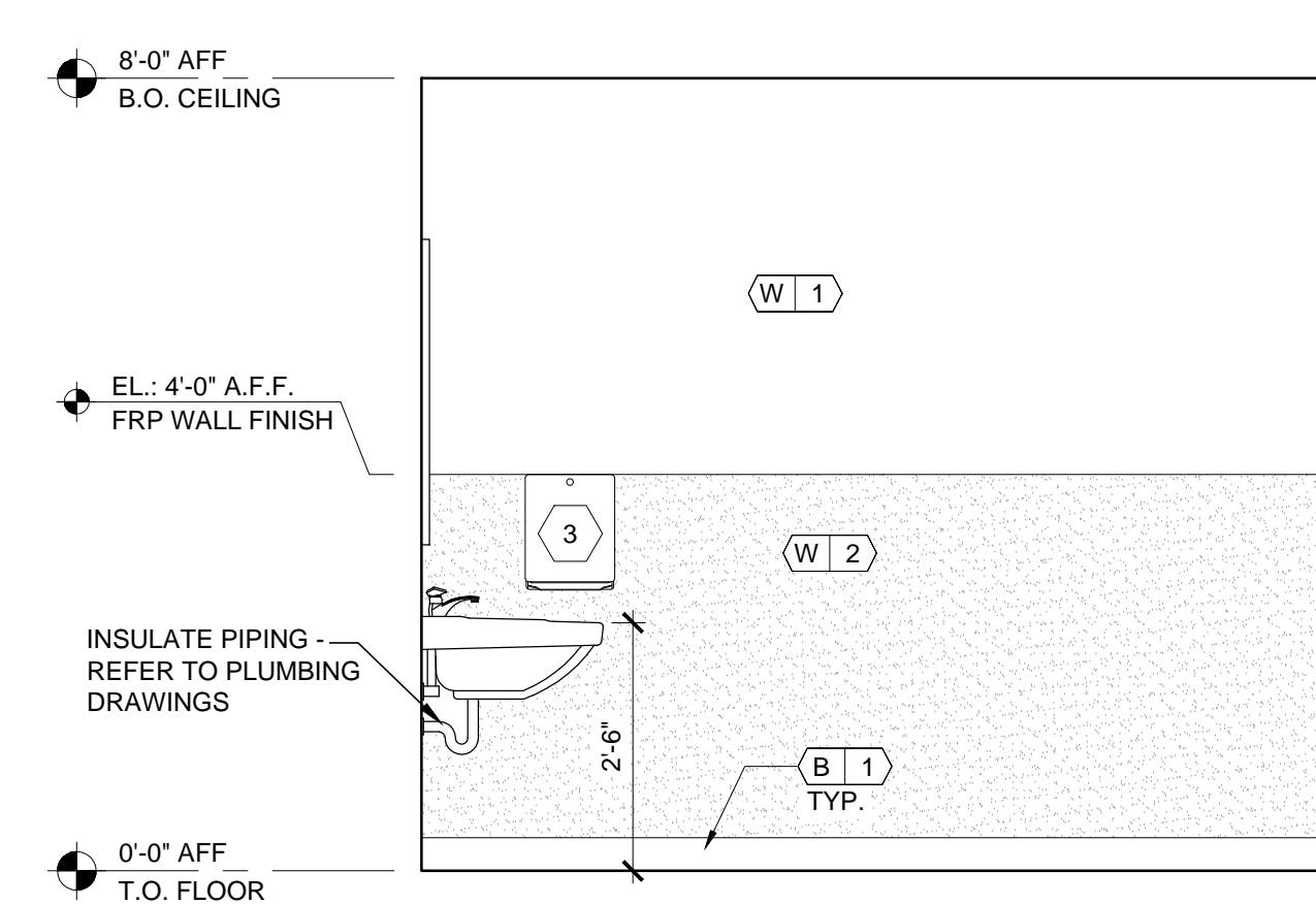
4 INTR ELEVATION - WOMEN'S TOILET ROOM
