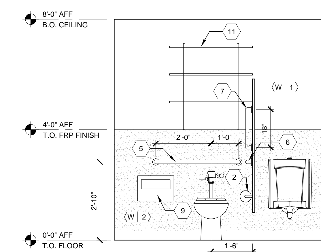
8 INTR ELEVATION - MEN'S TOILET ROOM
