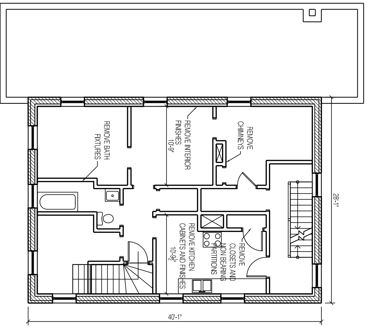
02 DEMO PLAN 1/8" = 1'-0"
