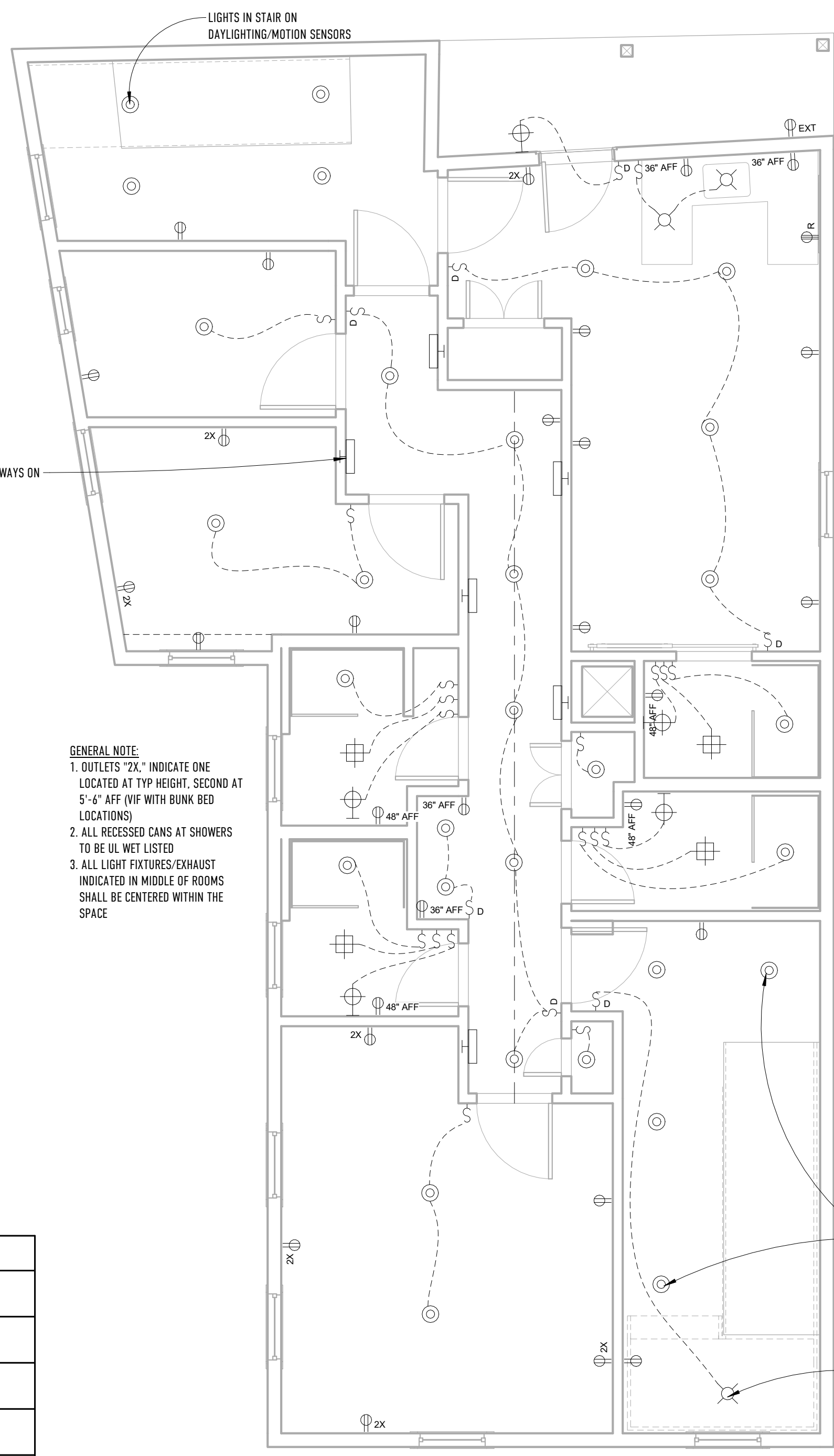
1 THIRD FLOOR 1/4" = 1'-0"
