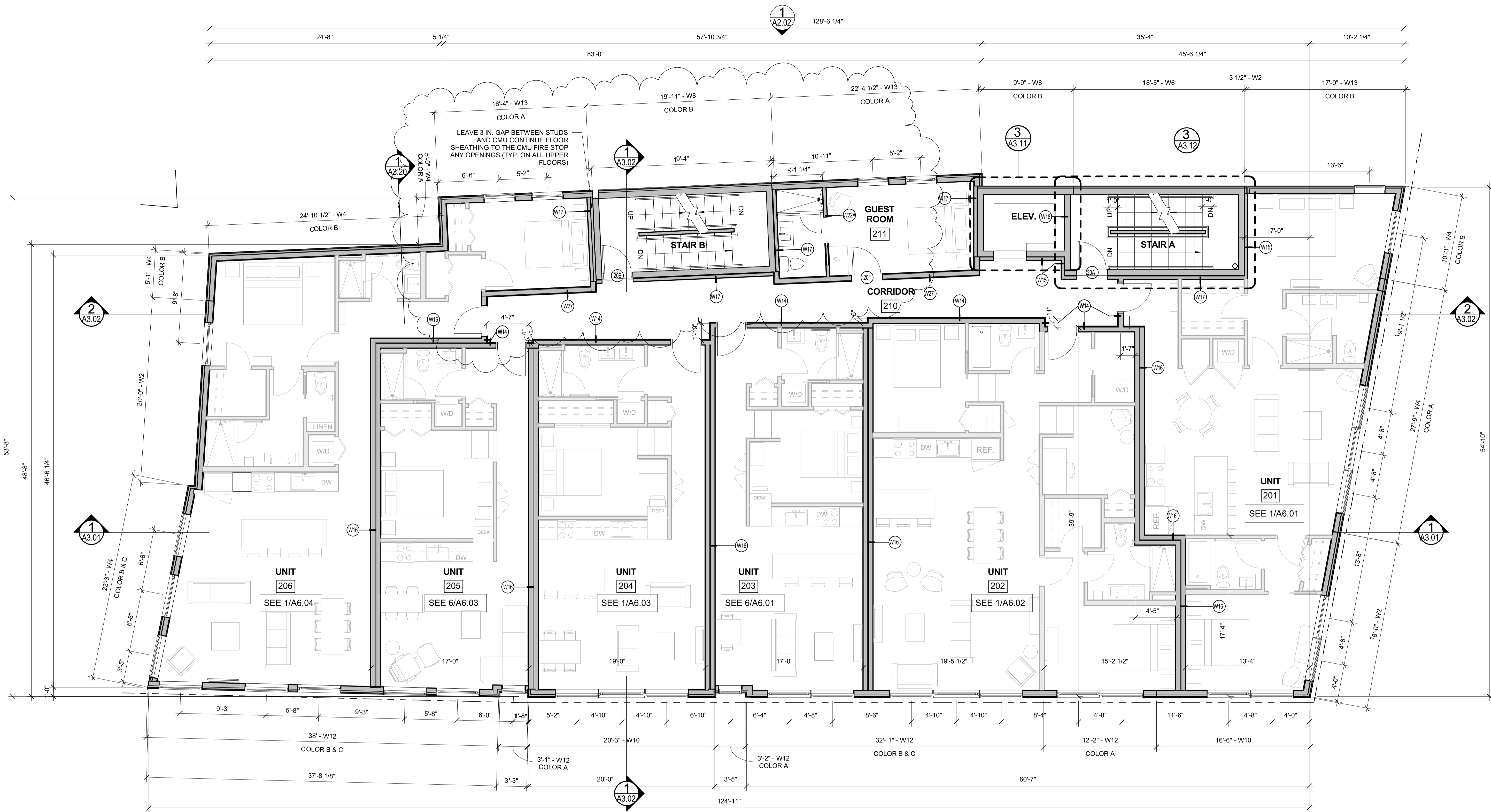
1 | 2ND FLOOR 3/16" = 1'-0"
