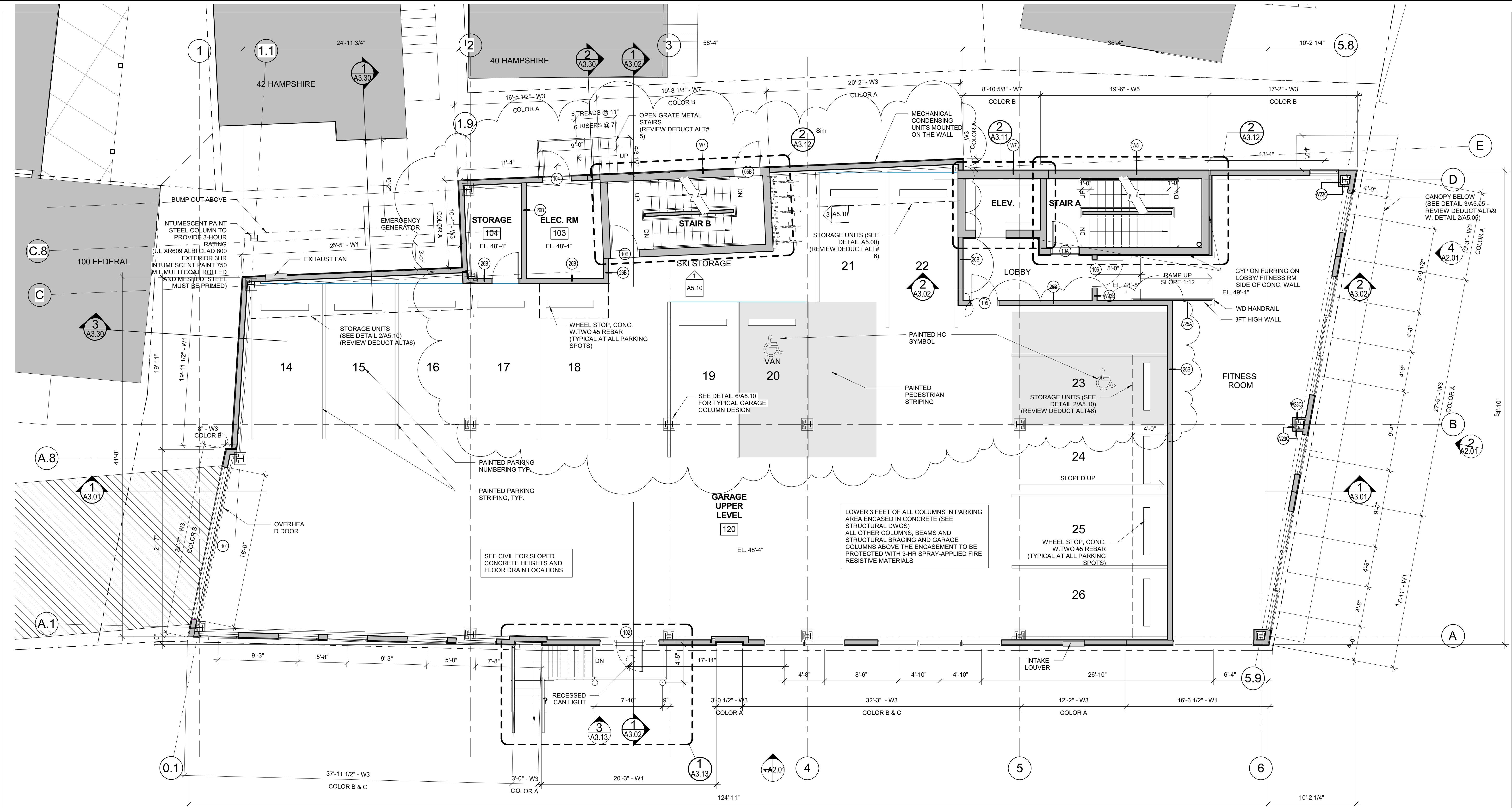
1 | 1ST FLOOR 3/16" = 1'-0" 0 2'-0" 4'-0" 8'-0" 16'-0"
