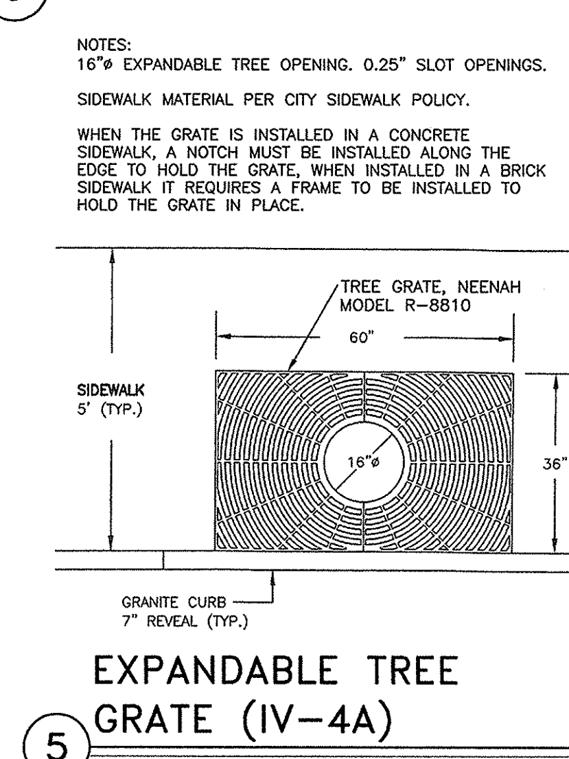
5 EXPANDABLE TREE GRATE (IV-4A) NOT TO SCALE
