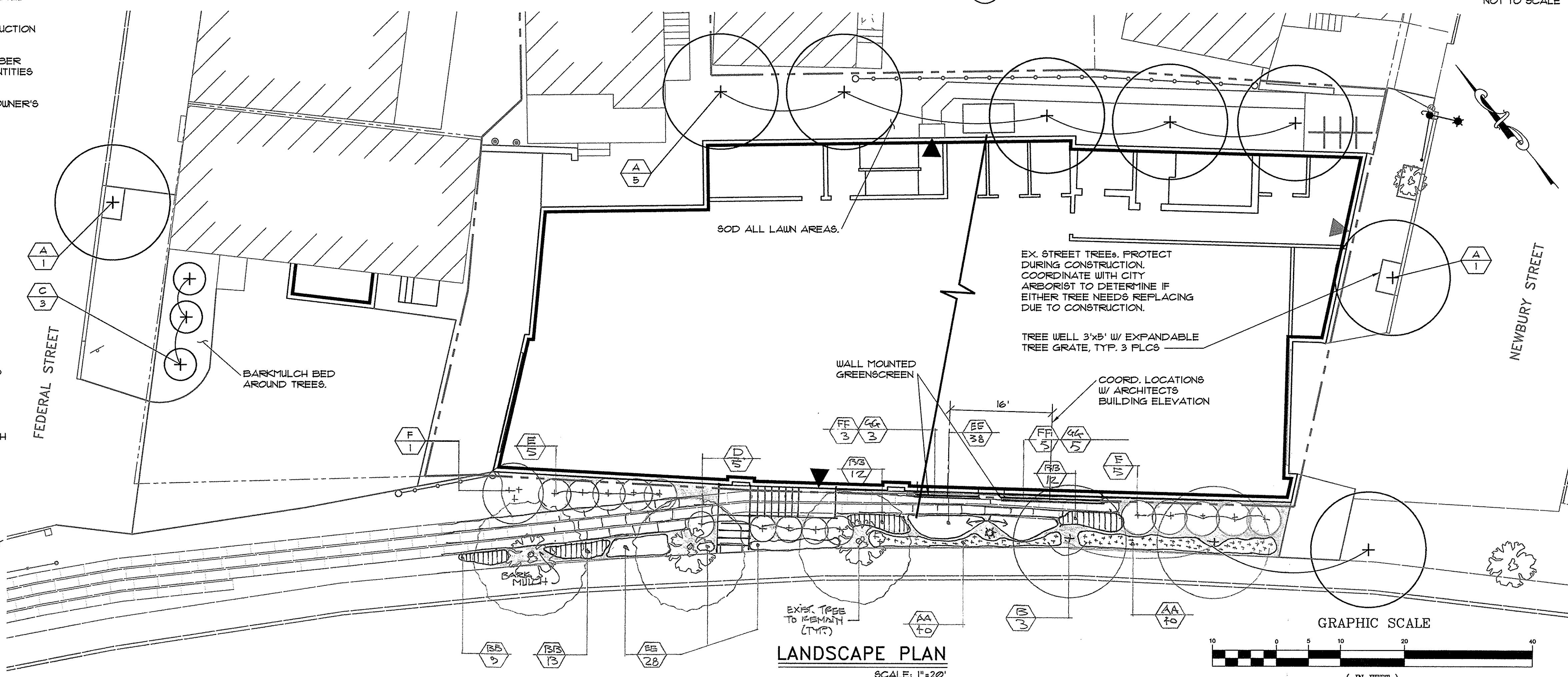
LANDSCAPE PLAN SCALE: 1"=20' FOR LEGEND SEE SHEET C1.4
