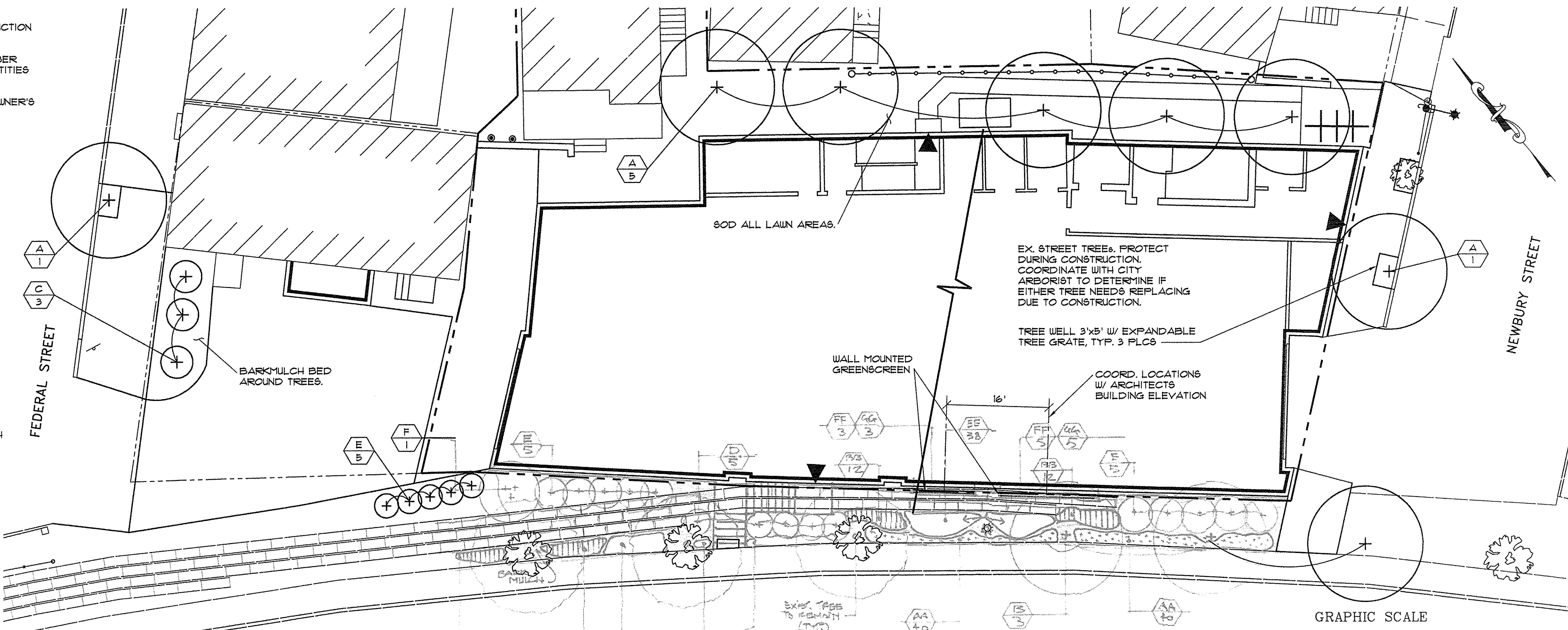
LANDSCAPE PLAN SCALE: 1"=20' FOR LEGEND SEE SHEET C1.4
