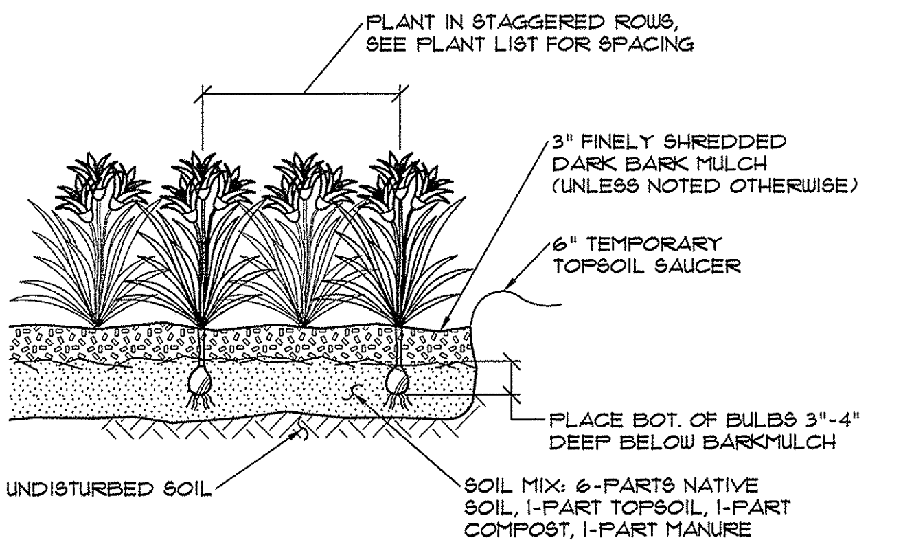
2 DAYLILY PLANTING DETAIL NOT TO SCALE
