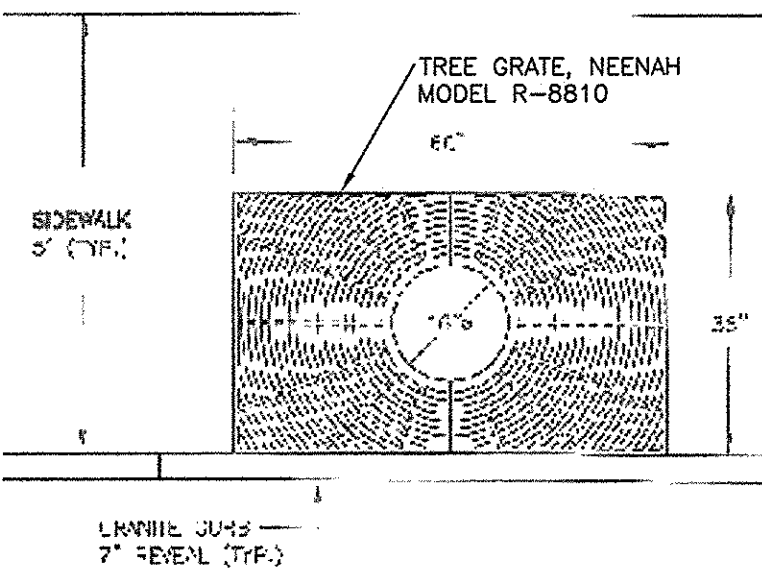
5 EXPANDABLE TREE GRATE (IV-4A) NOT TO SCALE
