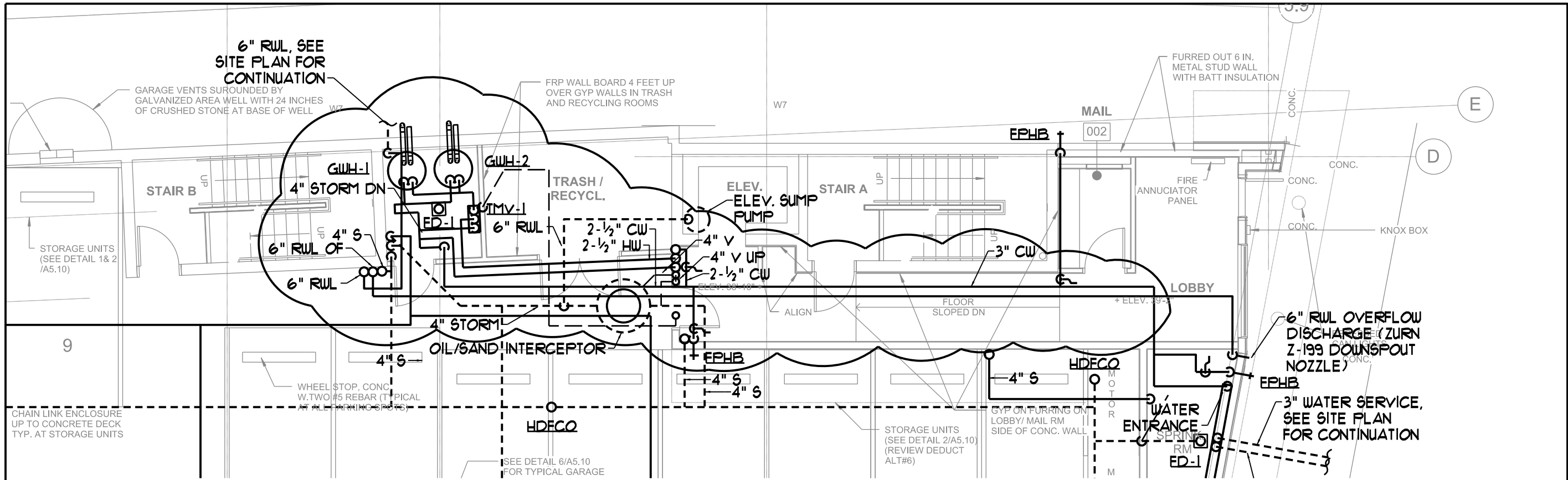
FIRST FLOOR PARTIAL PLUMBING PLAN
