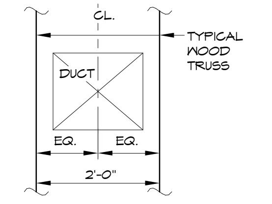
TYPICAL TRUSS LAYOUT @ MECHANICAL UNITS
