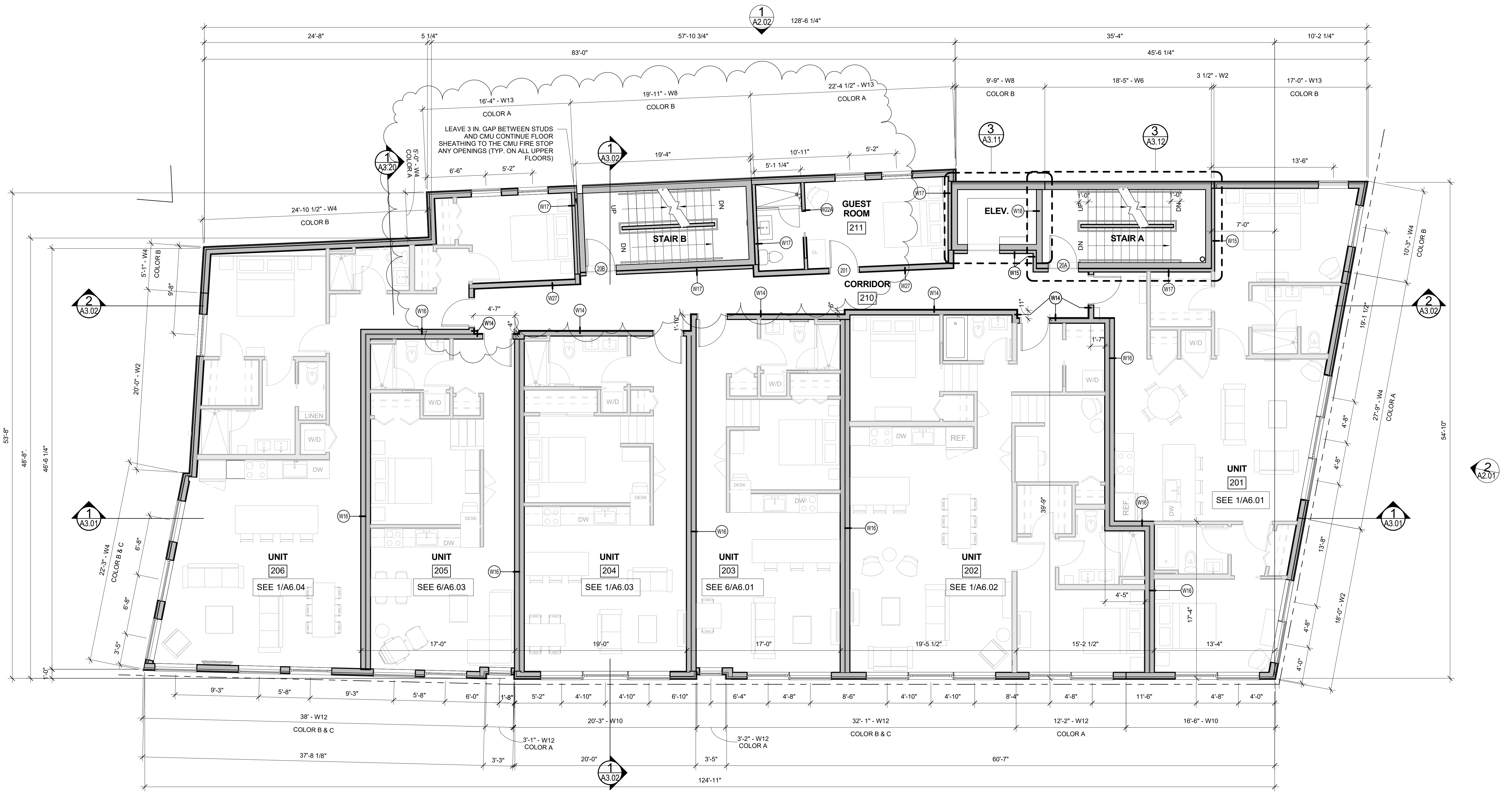
1 | 2ND FLOOR 3/16" = 1'-0"
