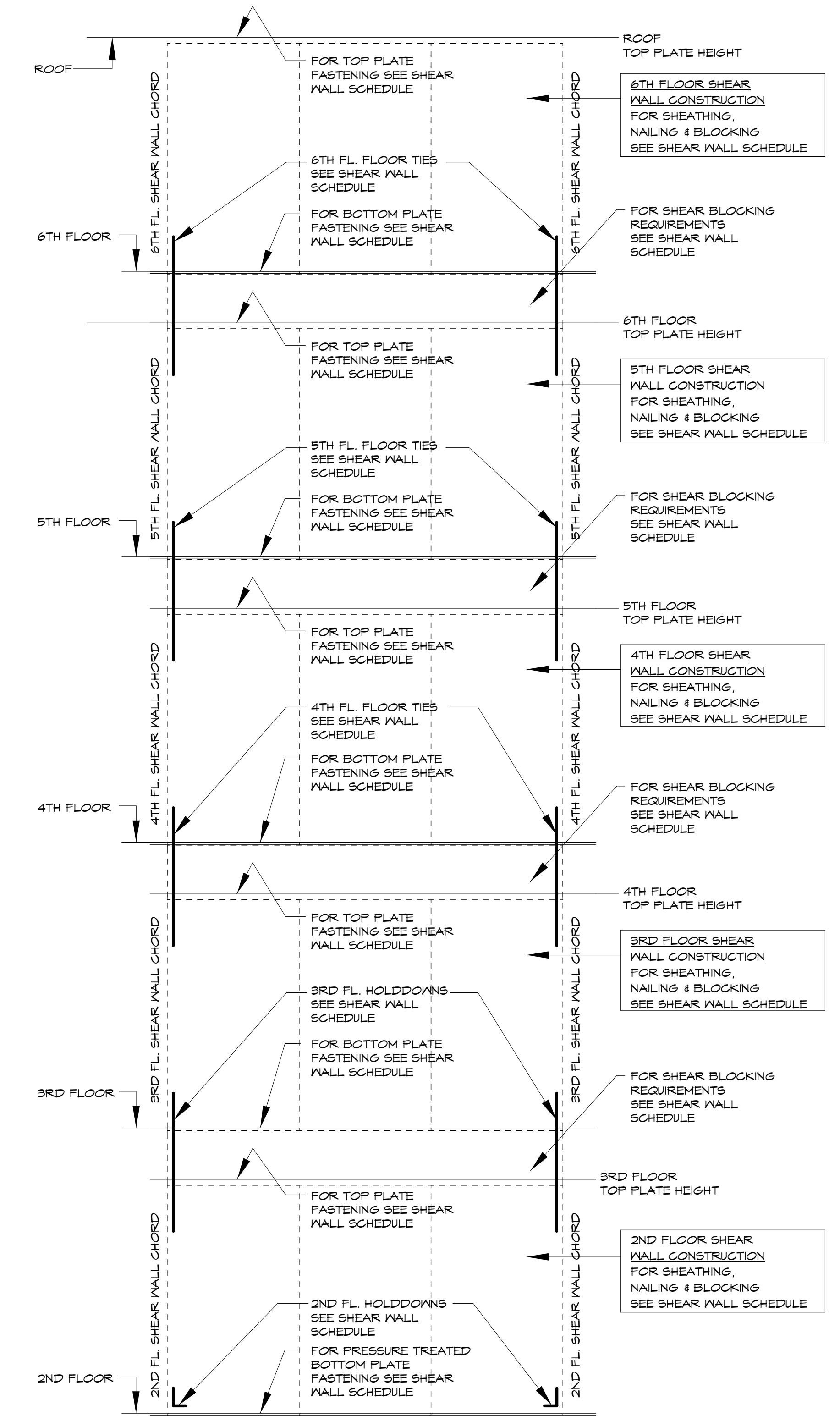
1 3/4" = 1'-0" SHEAR WALL ELEVATION
