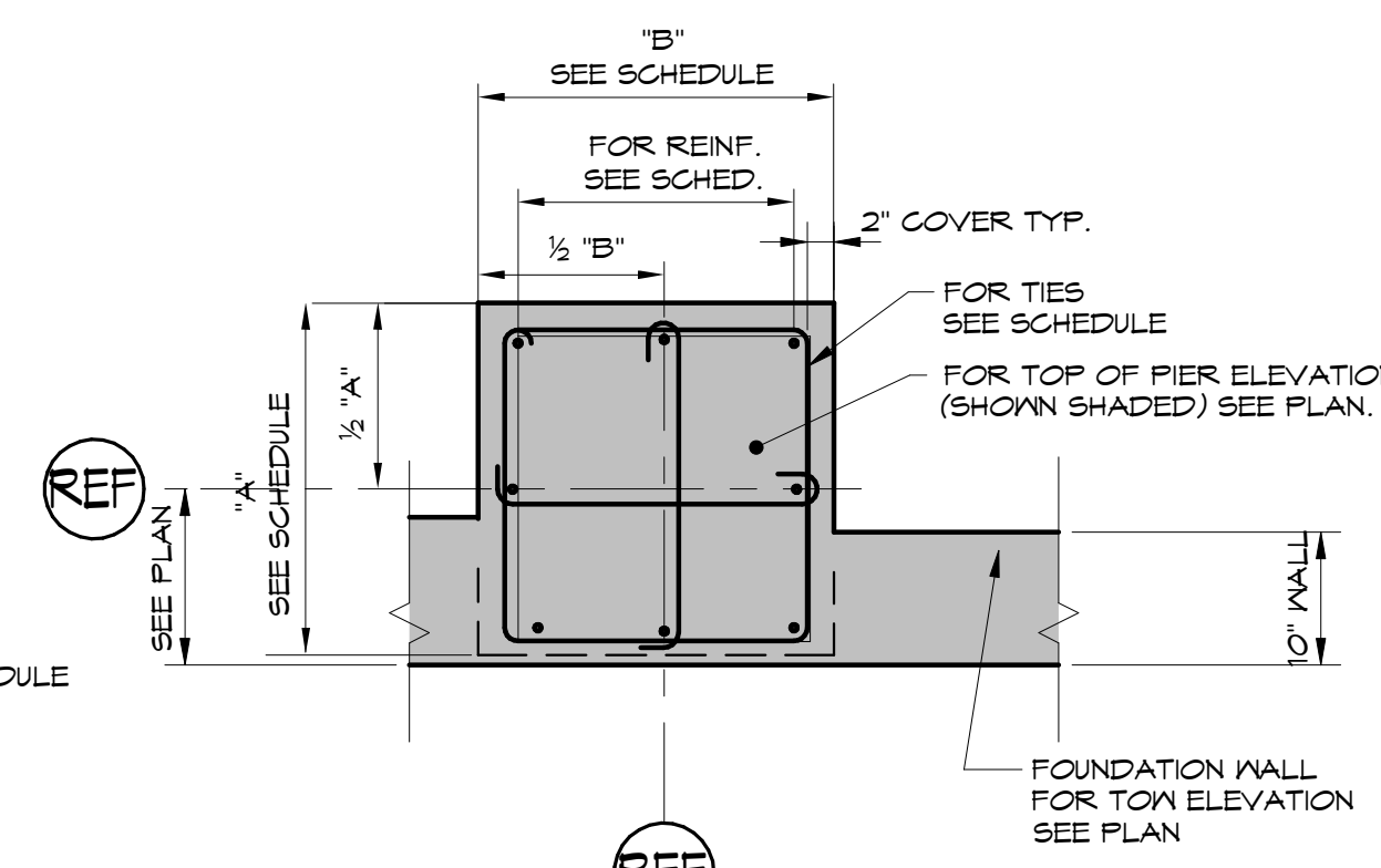
PIER DETAIL TYPE - B
