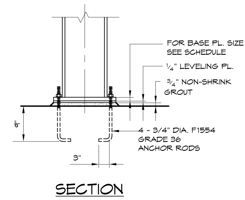
BASE PLATE - TYPE "A"
