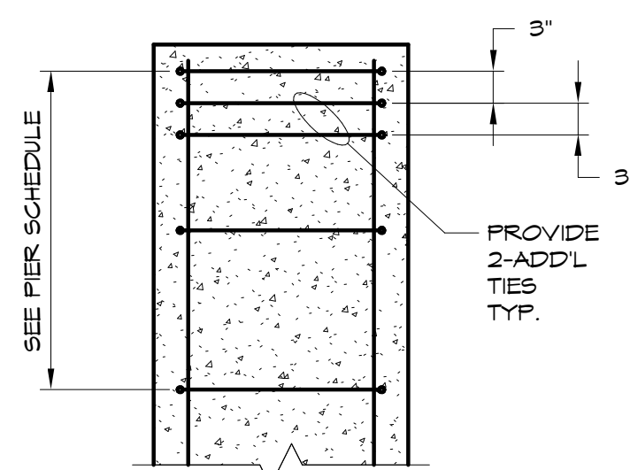
SECTION AT TYPICAL PIER 3/4"=1'-0"
