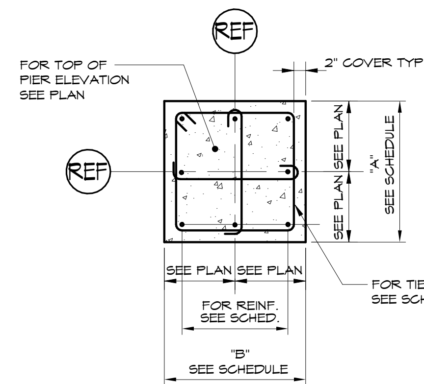
PIER DETAIL TYPE - A
