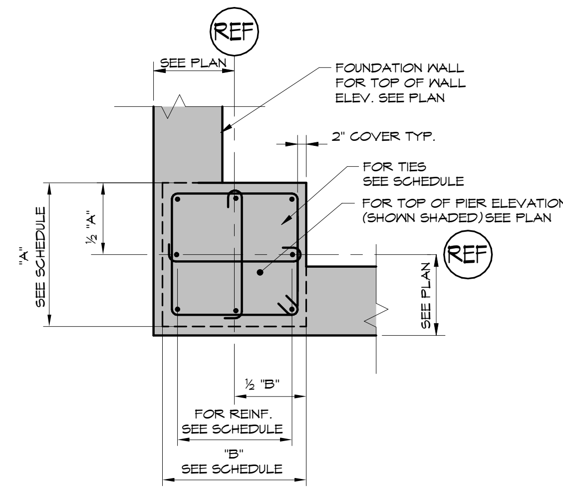
PIER DETAIL TYPE - C
