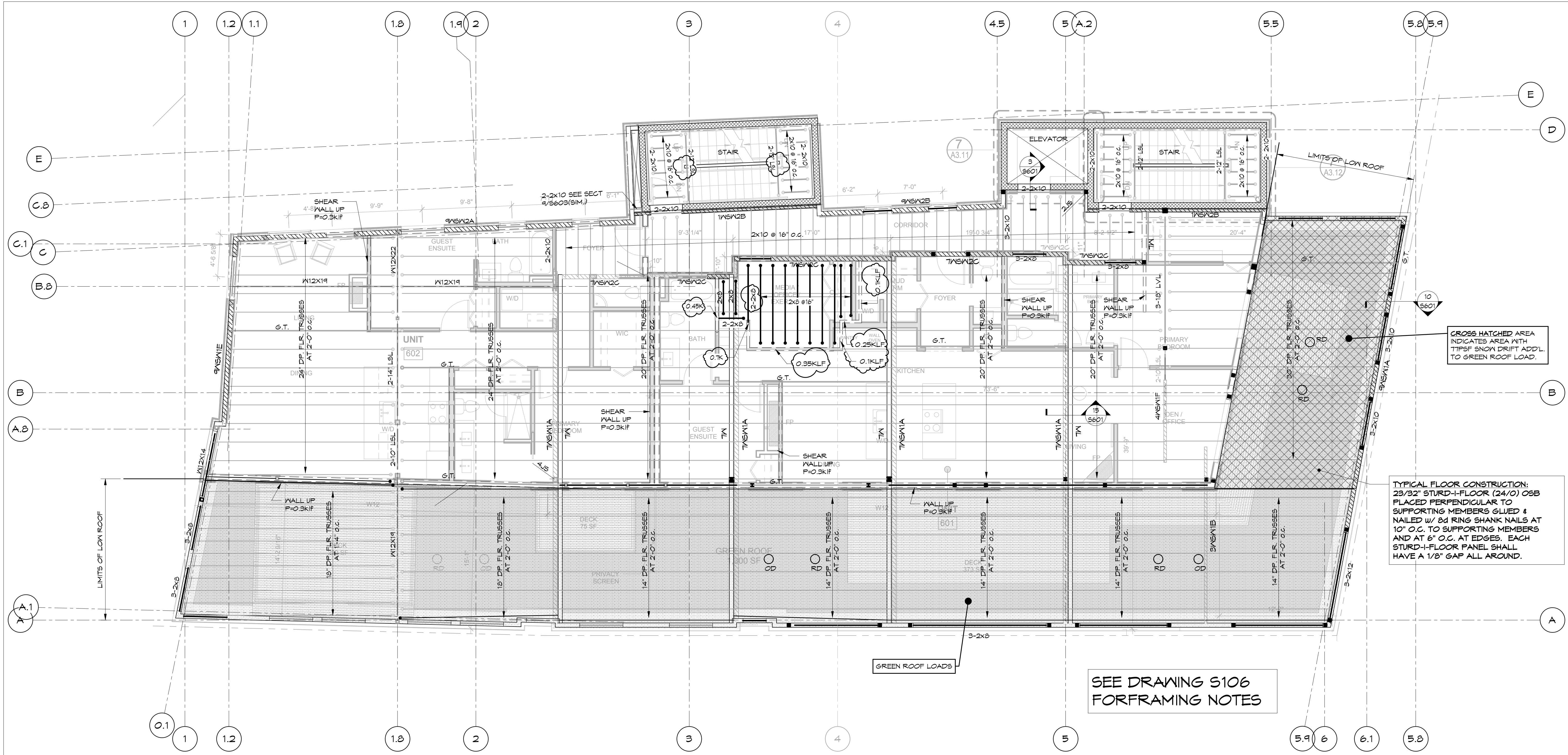
1 SIXTH FLOOR PLATFORM FRAMING PLAN 3/16" = 1'-0"
