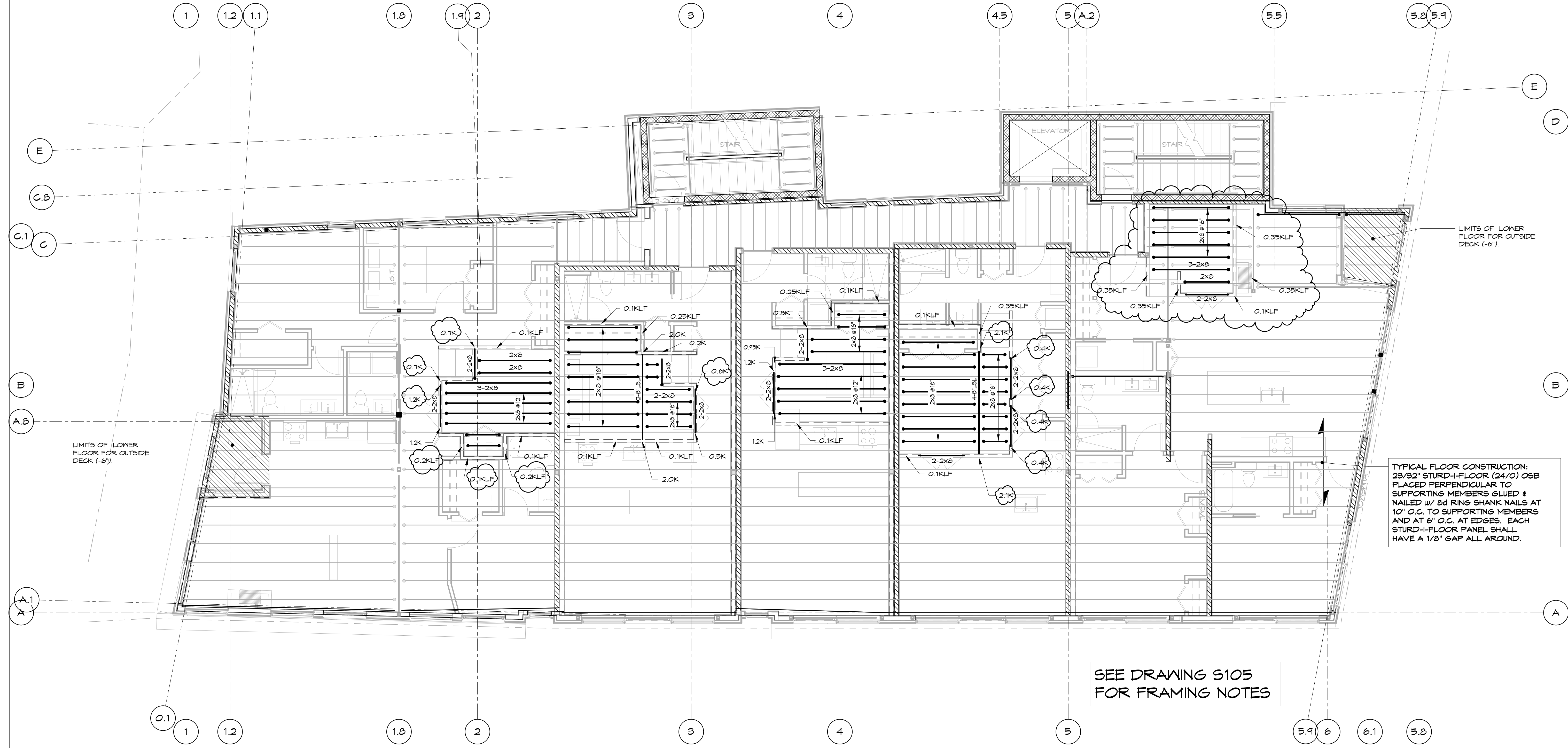
1 FIFTH FLOOR PLATFORM FRAMING PLAN 3/16" = 1'-0"
