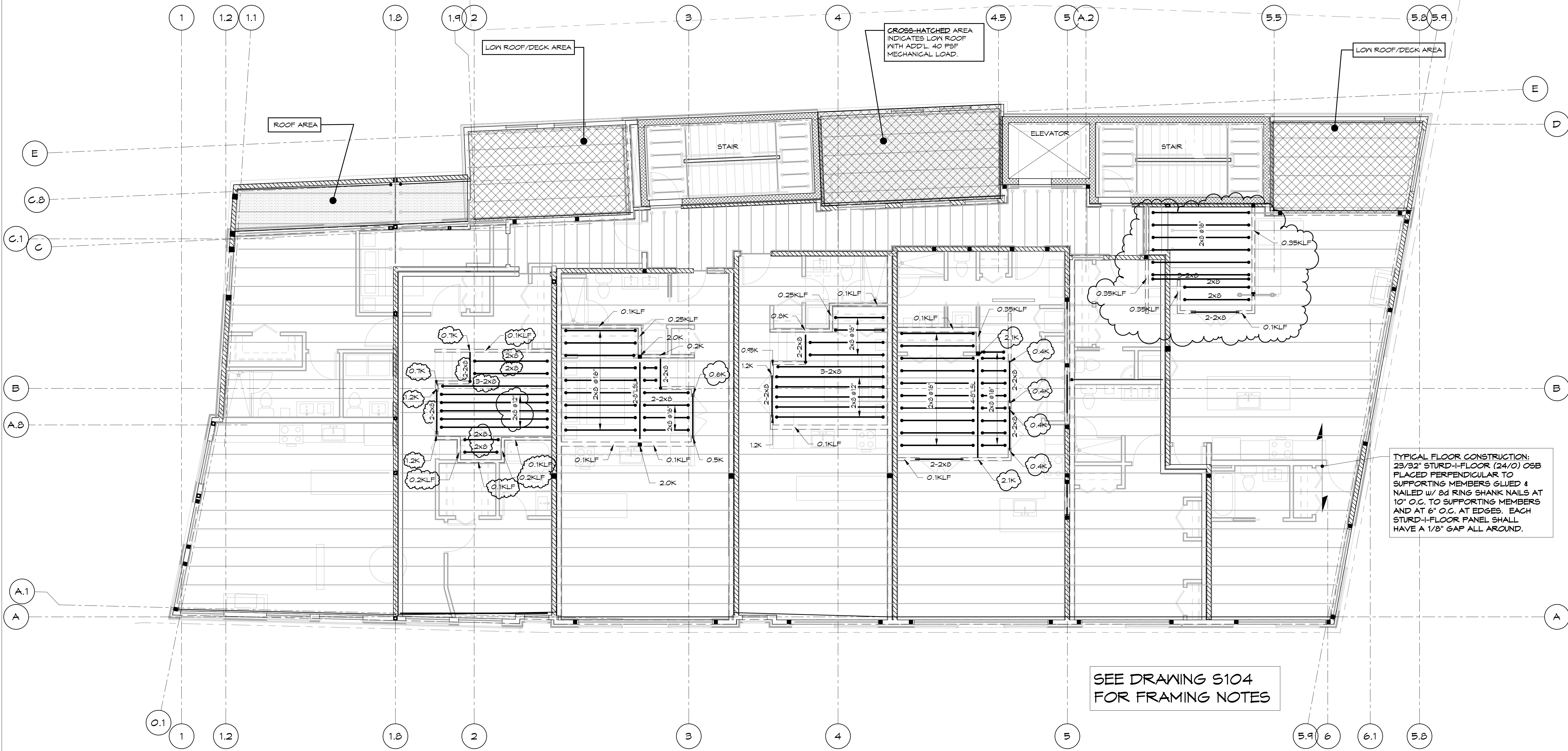
1 FOURTH FLOOR PLATFORM FRAMING PLAN 3/16" = 1'-0"
