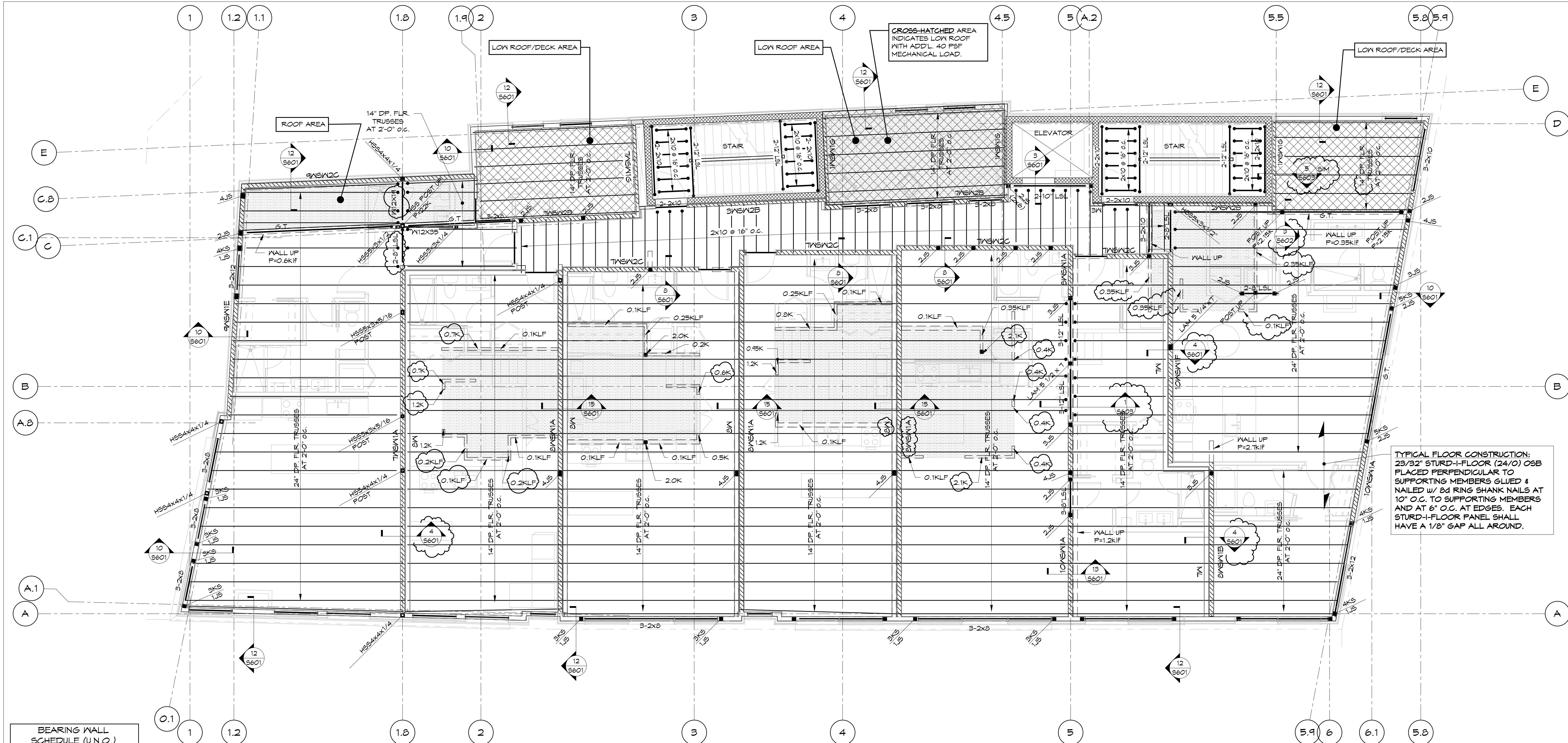
1 FOURTH FLOOR FRAMING PLAN 3/16" = 1'-0"
