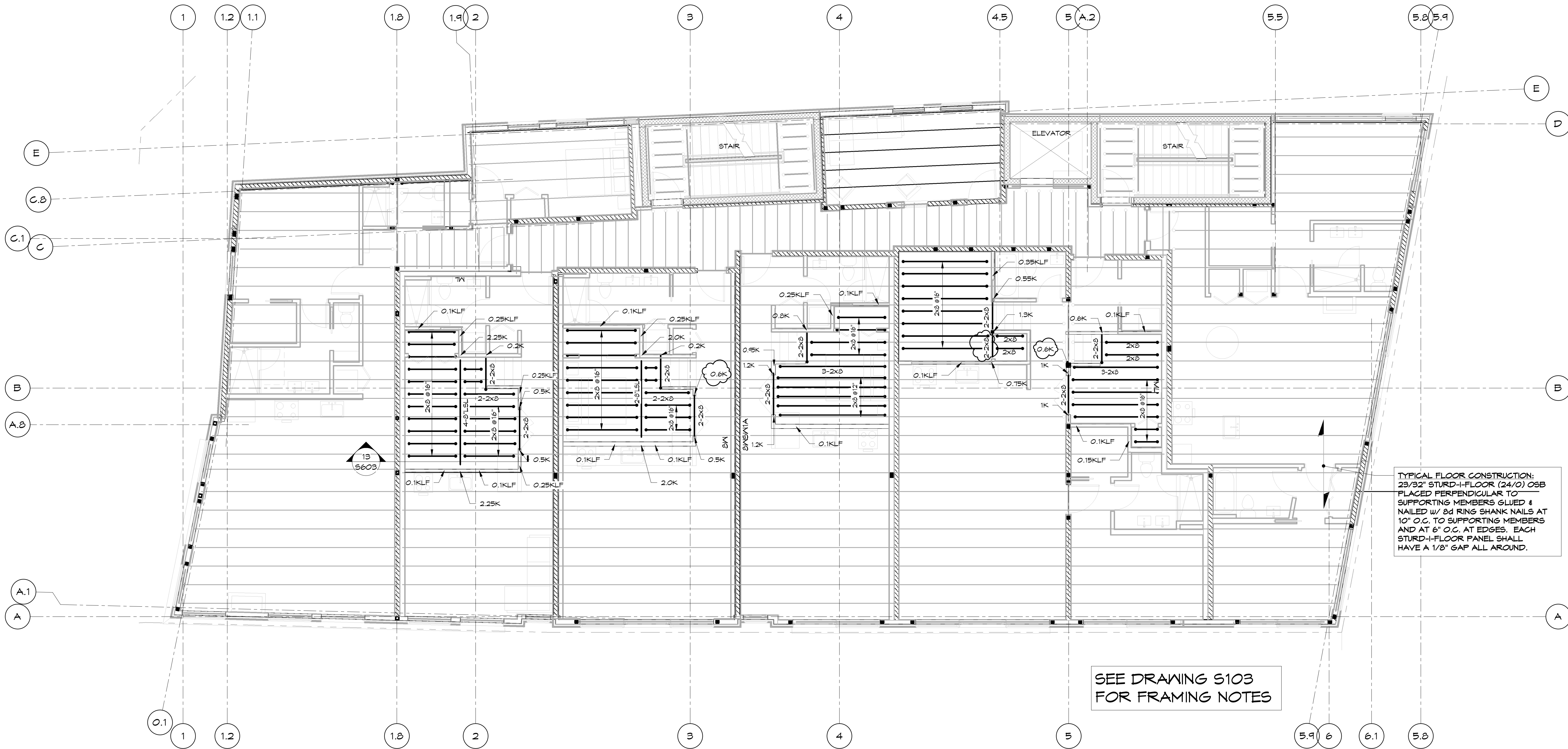
1 THIRD FLOOR PLATFORM FRAMING PLAN 3/16" = 1'-0"
