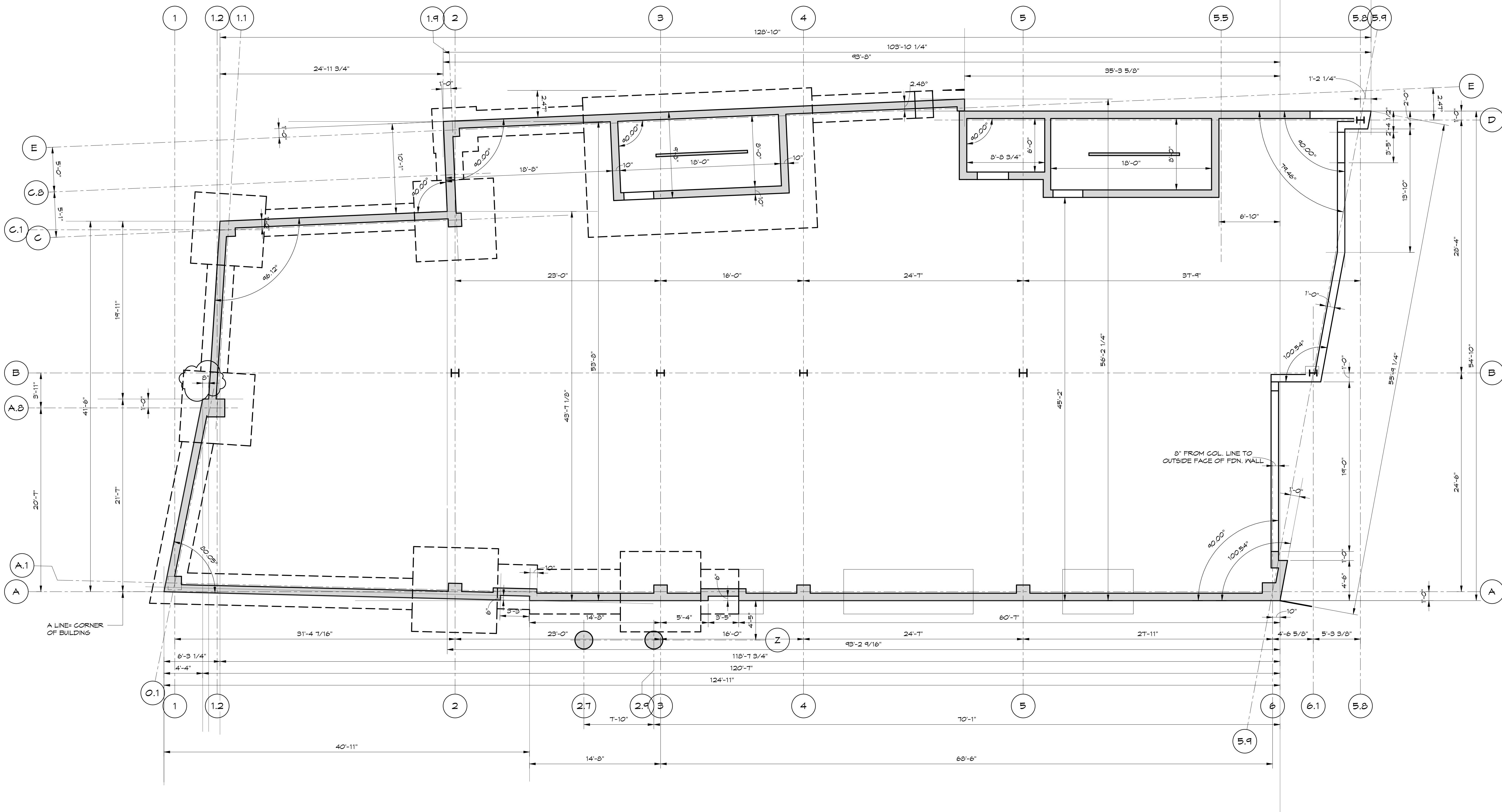
1 FOUNDATION WALL DIMENSION PLAN (BASEMENT LEVEL) 3/16" = 1'-0"
