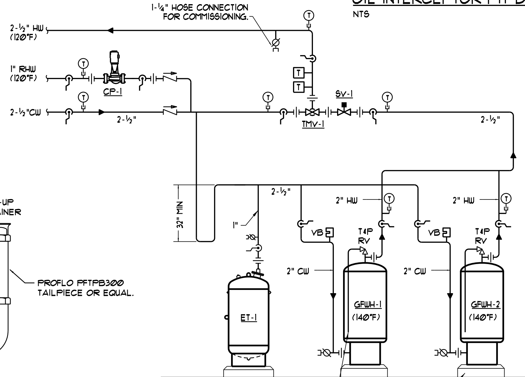
DOMESTIC HOT WATER PIPING SCHEMATIC NTS
