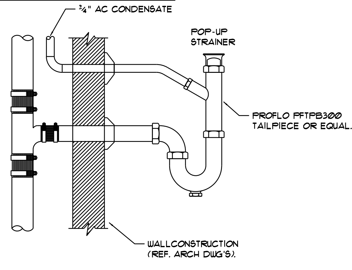
TYPICAL LAVATORY WITH 3/4" AC CONDENSATE CONNECTION DETAIL NTS
