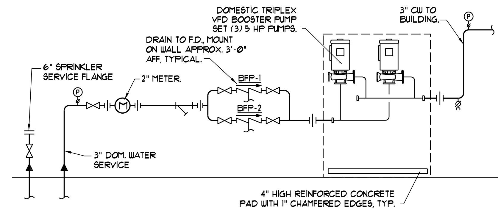
WATER ENTRANCE DETAIL NTS
