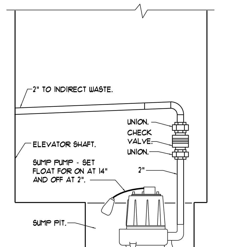
ELEVATOR SUMP PUMP PIPING DETAIL NTS
