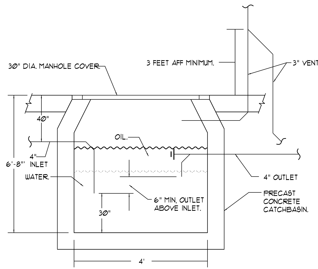
OIL INTERCEPTOR PIT DETAIL NTS
