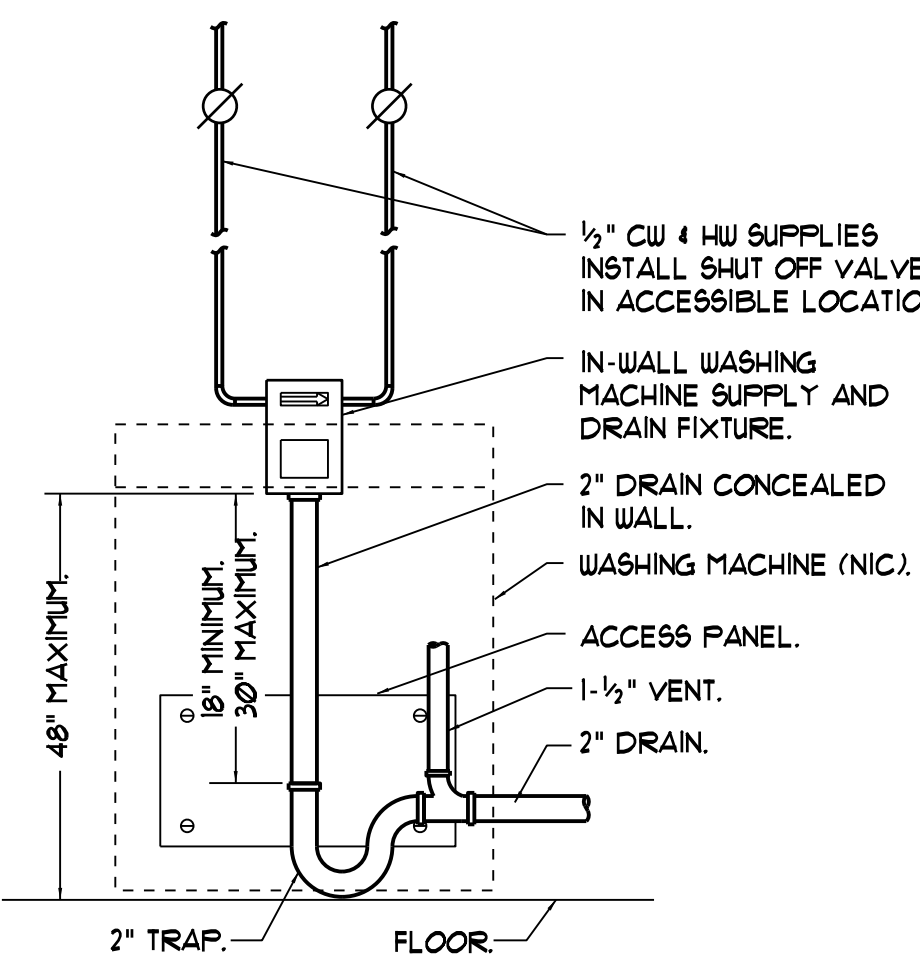
WASHING MACHINE HOOK-UP DETAIL NTS
