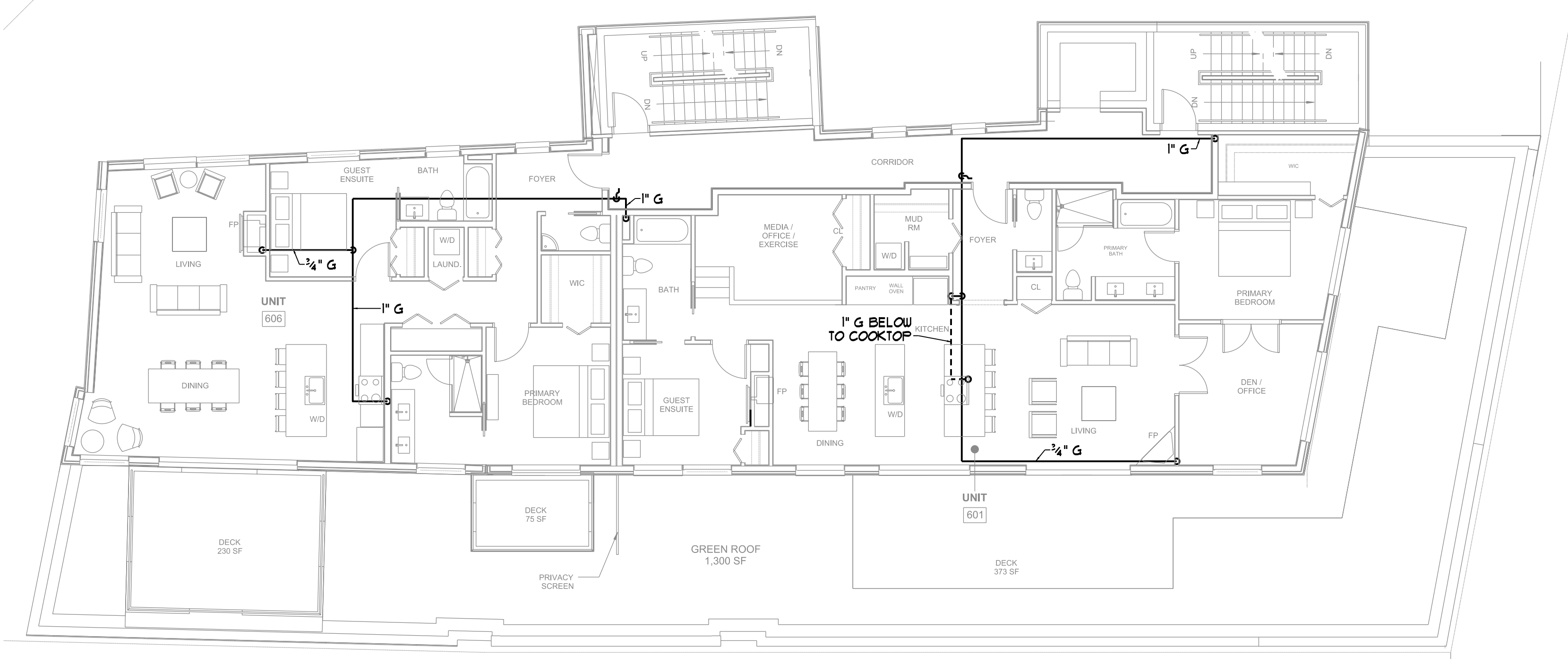
SIXTH FLOOR GAS PIPING PLAN SCALE - 1/8" = 1'-0"
