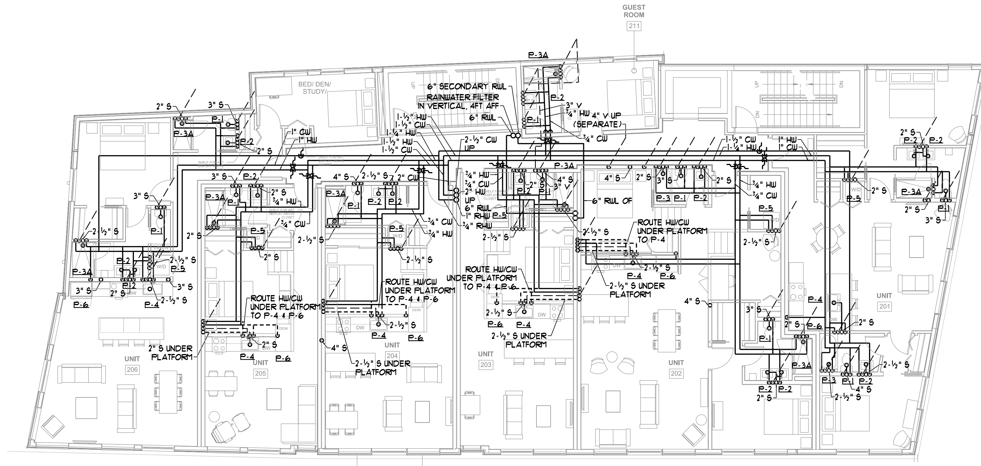
SECOND FLOOR PLUMBING PLAN SCALE - 1/8" = 1'-0"
