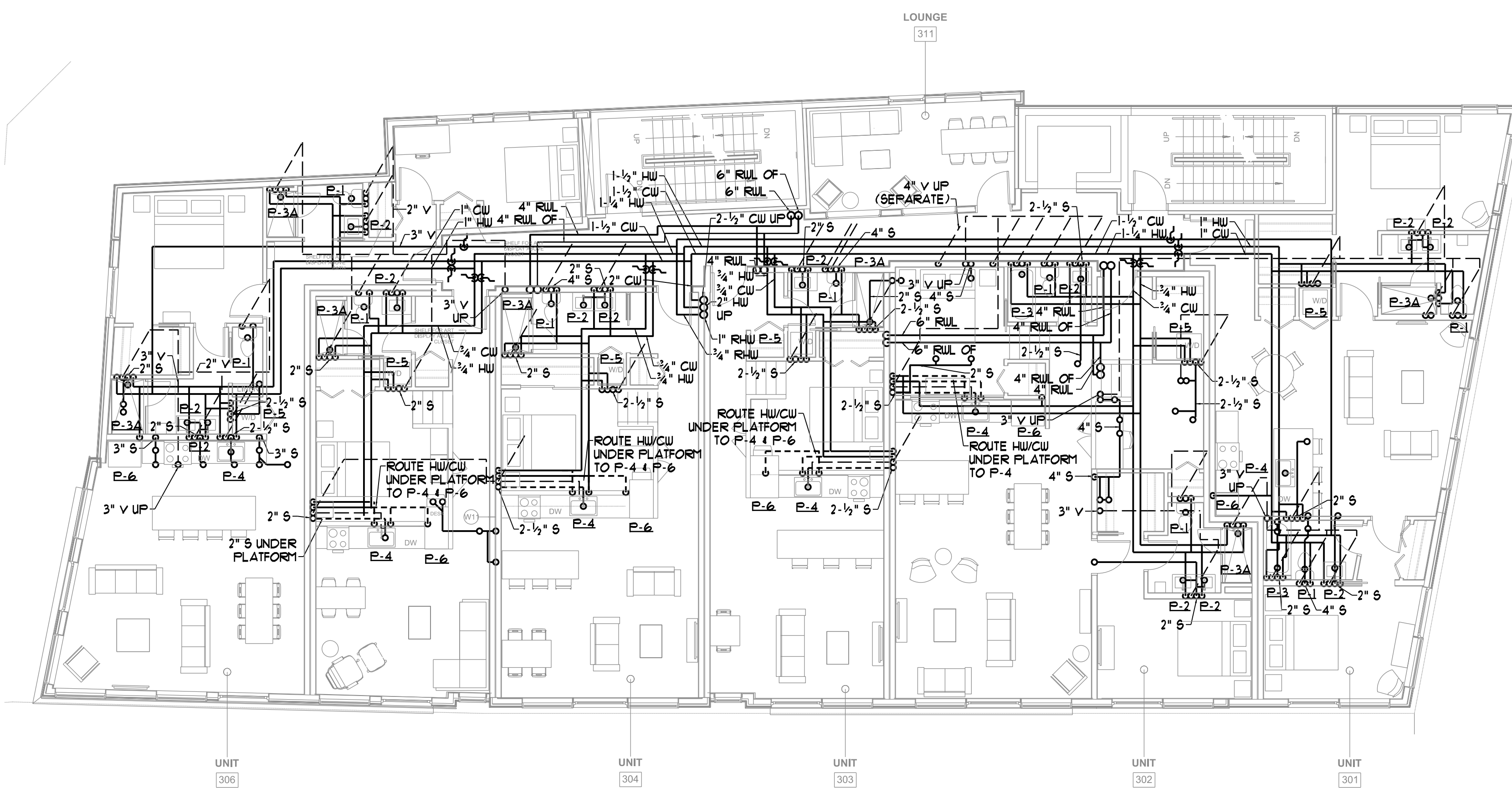
THIRD FLOOR PLUMBING PLAN SCALE - 1/8" = 1'-0"
