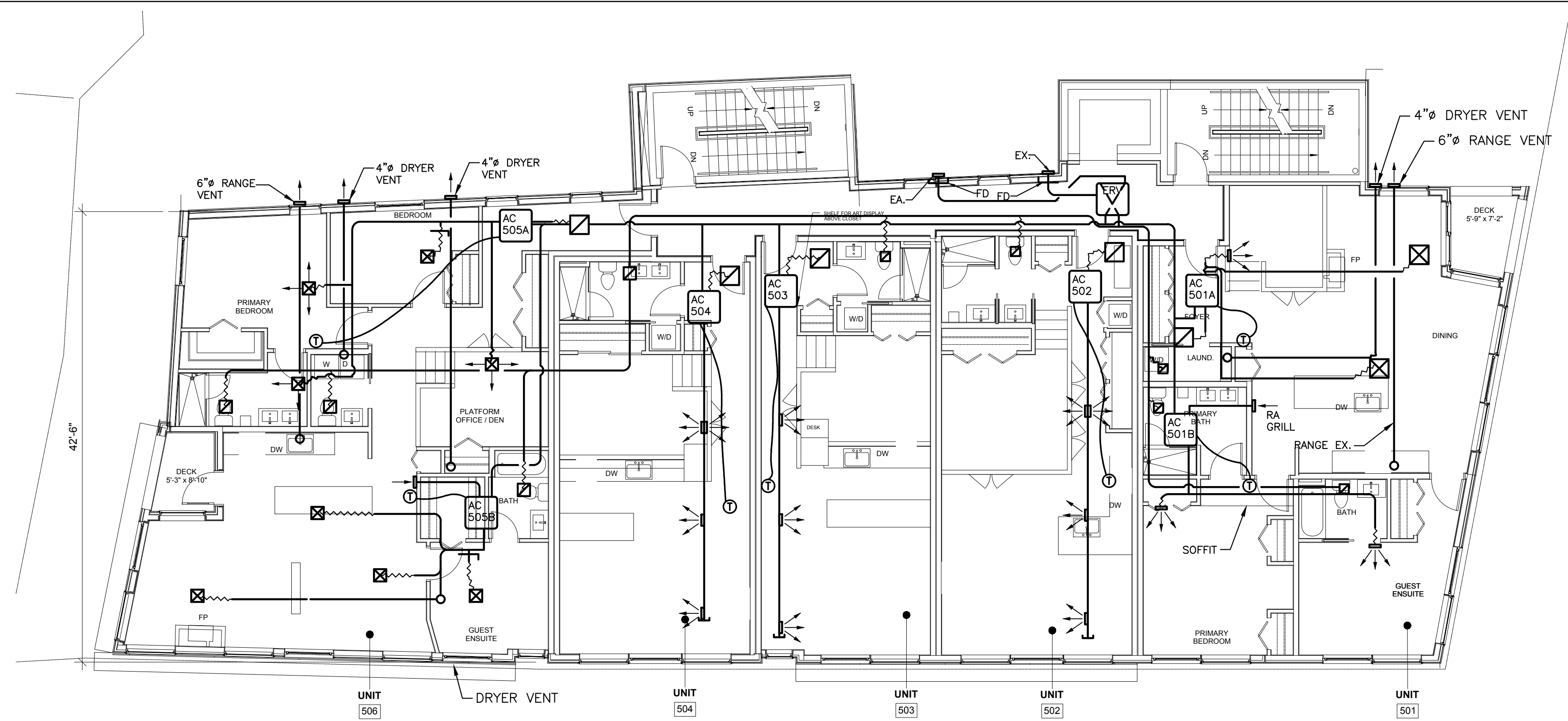
5TH FLOOR – DUCTWORK SCALE: 1/8"=1'-0"
