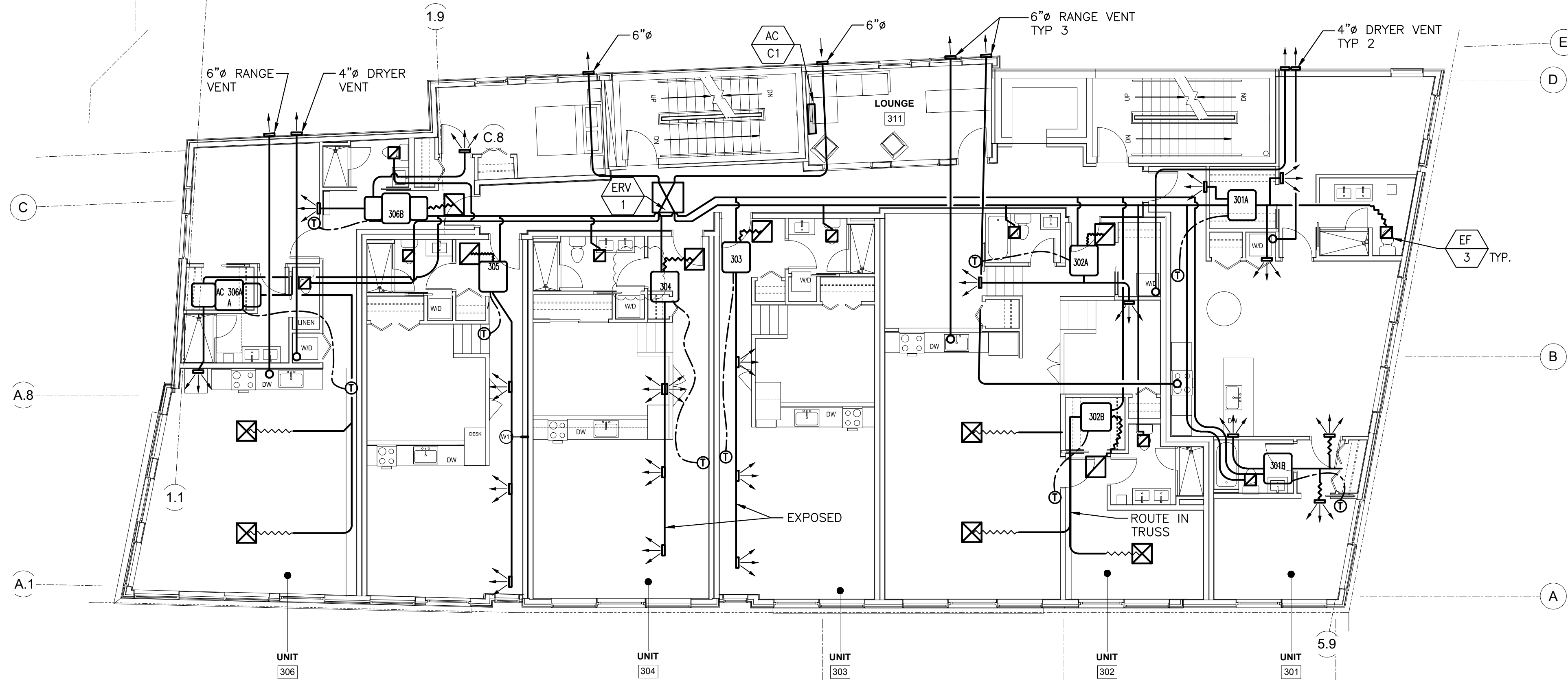
3RD FLOOR – DUCTWORK SCALE: 1/8"=1'-0"
