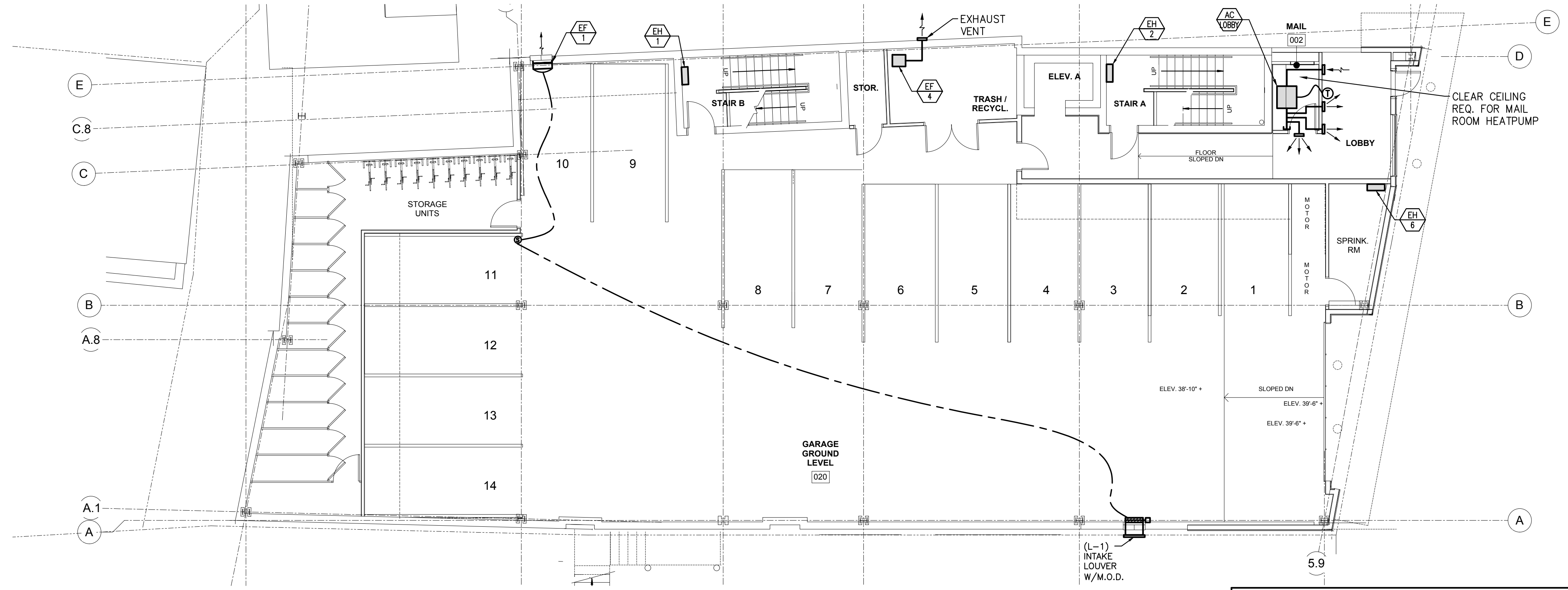
BASEMENT FLOOR - DUCTWORK SCALE: 1/8"=1'-0"
