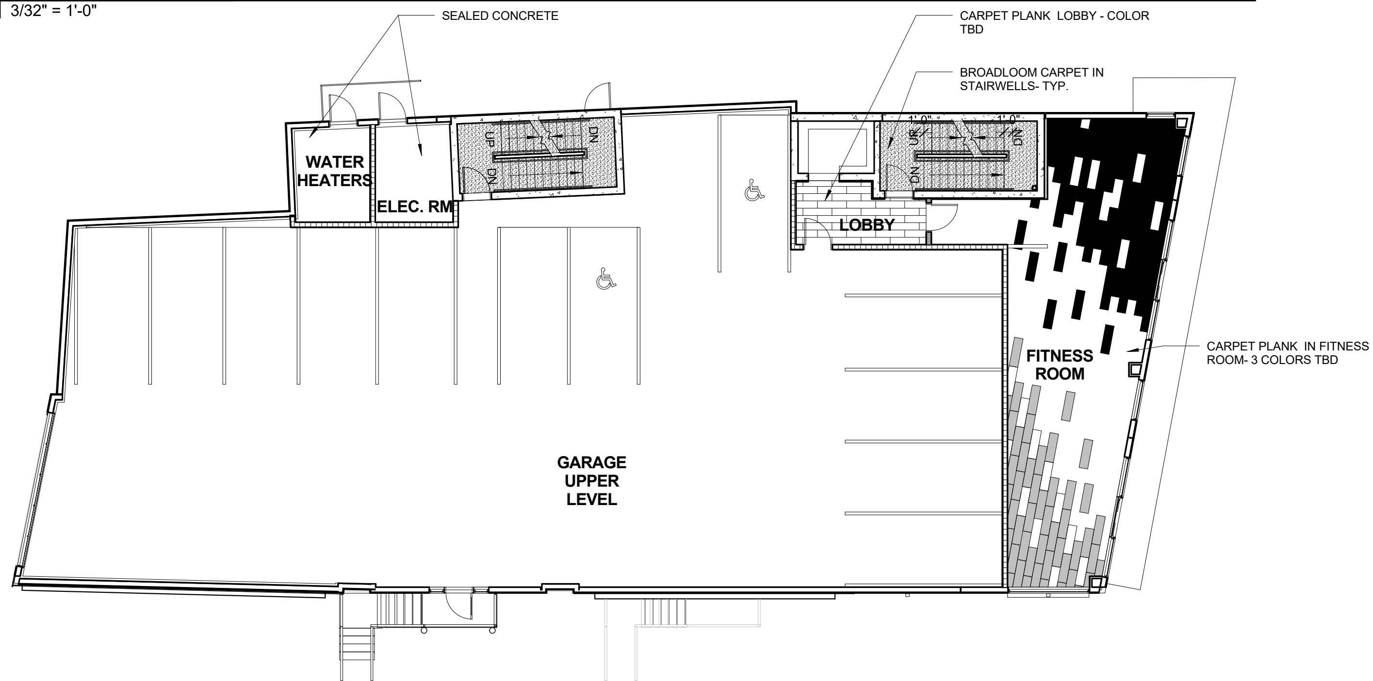
2 FINISH PLAN - 1ST FLOOR 3/32" = 1'-0"
