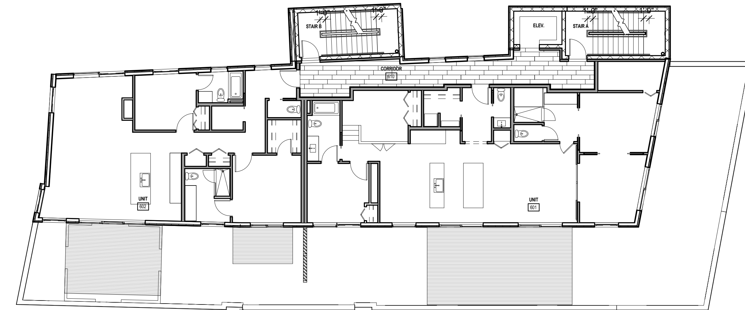
5 FINISH PLAN - 6TH FLOOR 3/32" = 1'-0"
