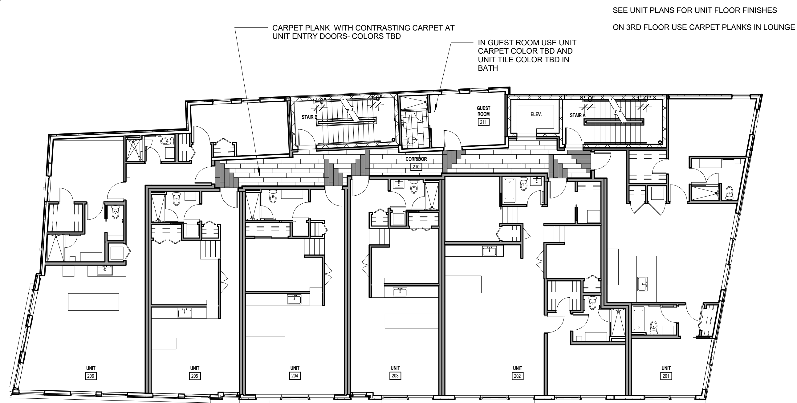
3 FINISH PLAN - 2ND & 3RD FLOOR 3/32" = 1'-0"
