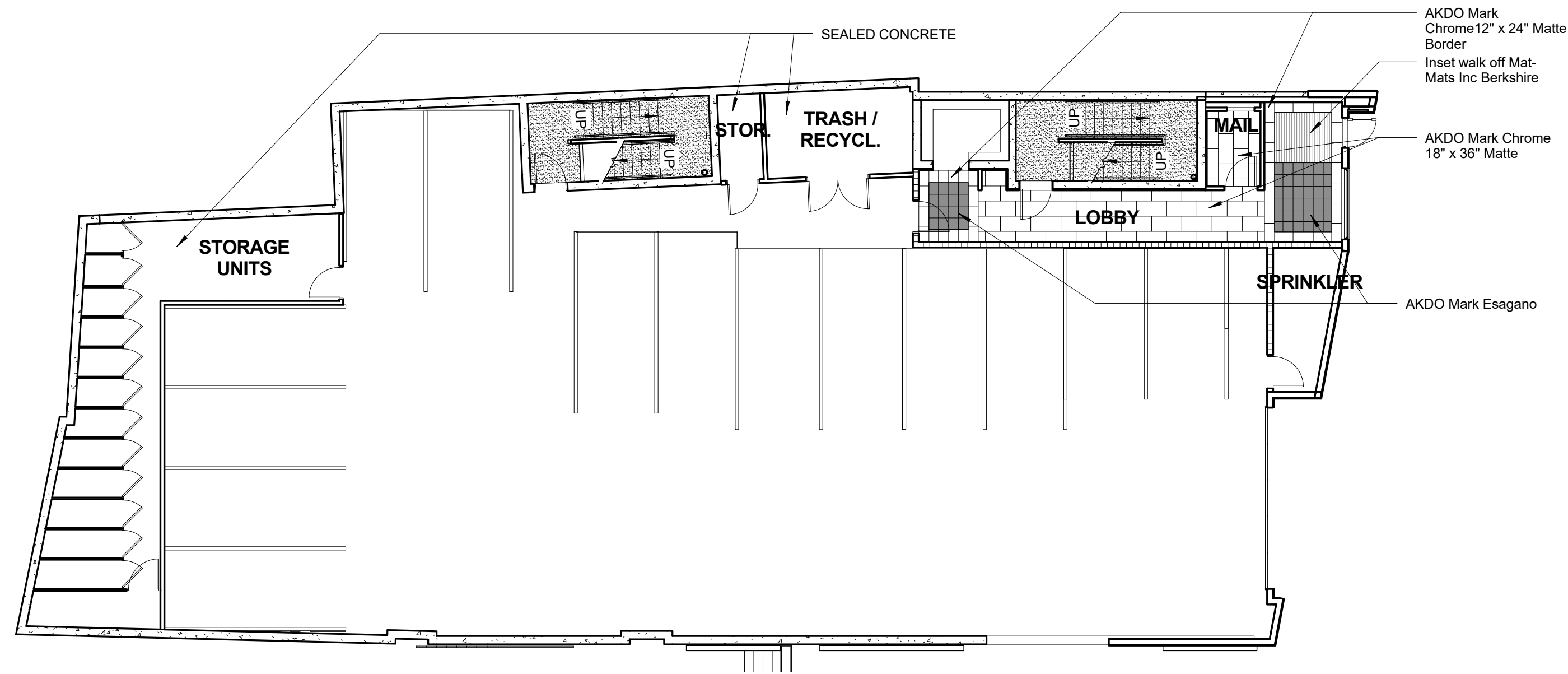
1 FINISH PLAN - BASEMENT 3/32" = 1'-0"
