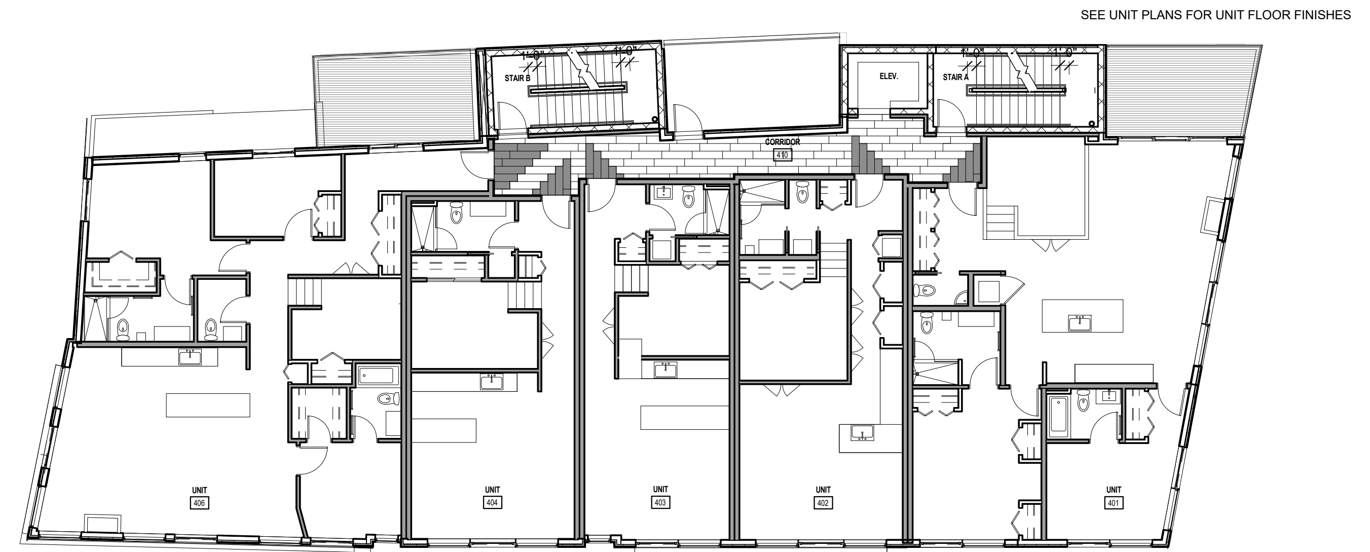
4 FINISH PLAN- 4TH & 5TH FLOOR 3/32" = 1'-0"
