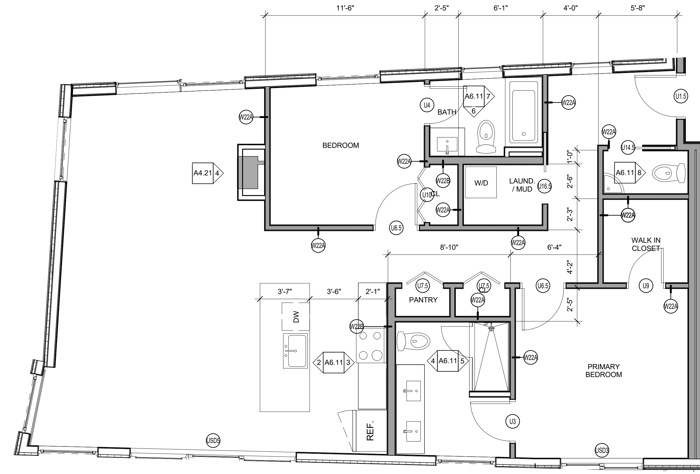
1 | ENLARGED PLAN - UNIT 602 1/4" = 1'-0" 0 1'-0" 2'-0" 4'-0" 8'-0"
