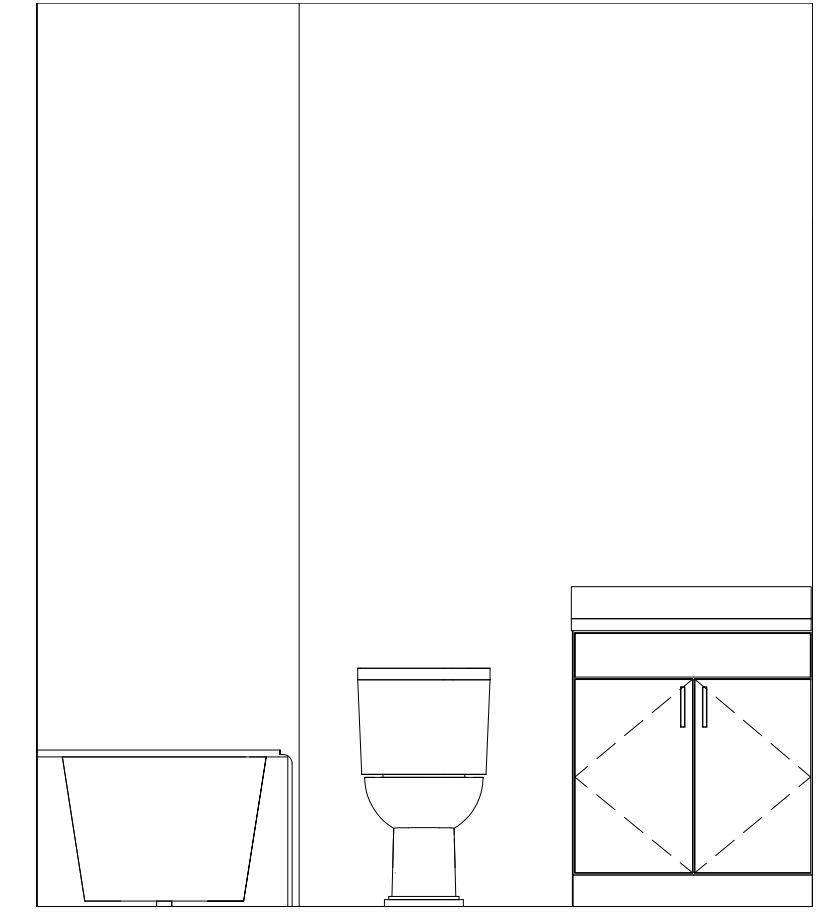
6 | UNIT 606 BATH 2 ELEV. A 1/2" = 1'-0" 0 0'-8" 1'-0" 2'-0" 4'-0"
