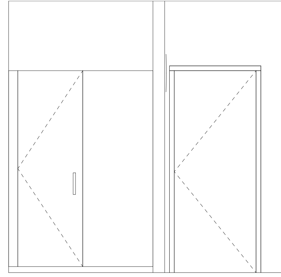
5 | UNIT 606 BATH ELEV. B 1/2" = 1'-0" 0 0'-8" 1'-0" 2'-0" 4'-0"
