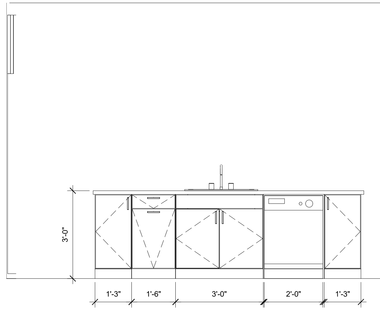
2 | UNIT 606 KITCHEN ELEV. A 1/2" = 1'-0" 0 0'-8" 1'-0" 2'-0" 4'-0"
