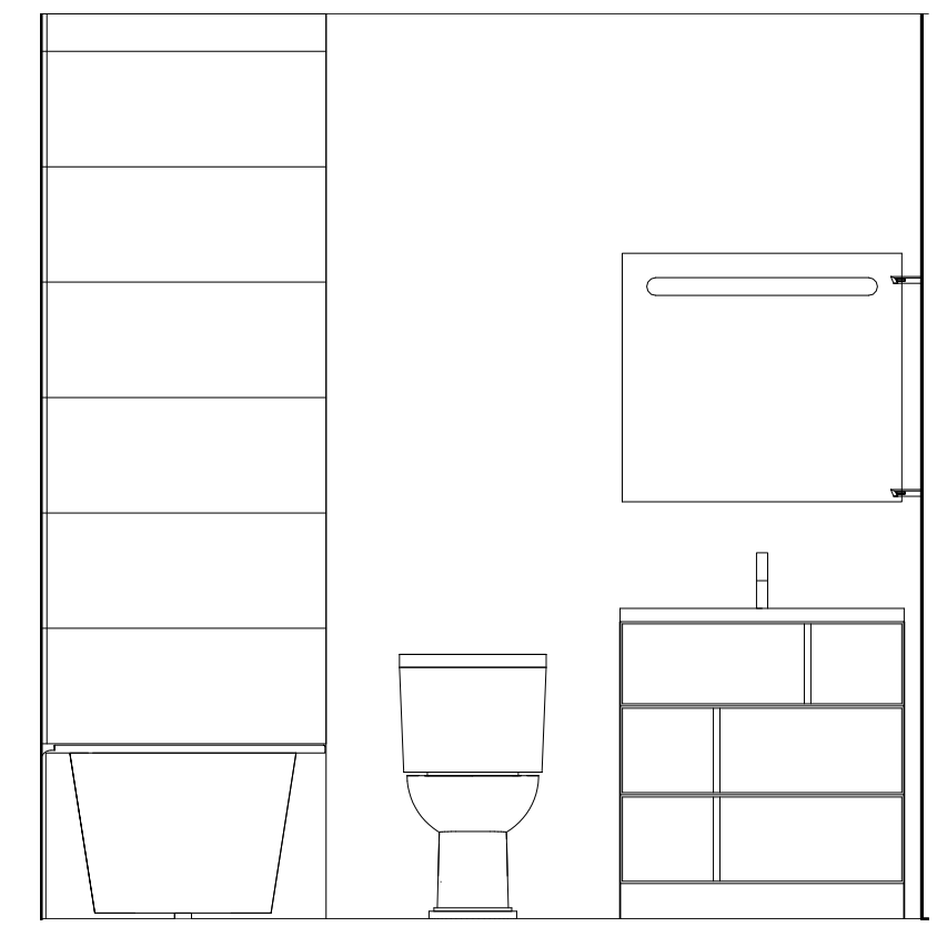
4 UNIT 401 BATH ELEV. A 1/2" = 1'-0"
