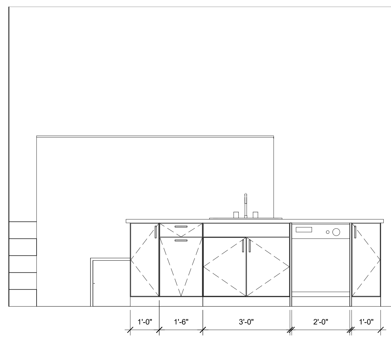
2 UNIT 401 KITCHEN ELEV. A 1/2" = 1'-0"
