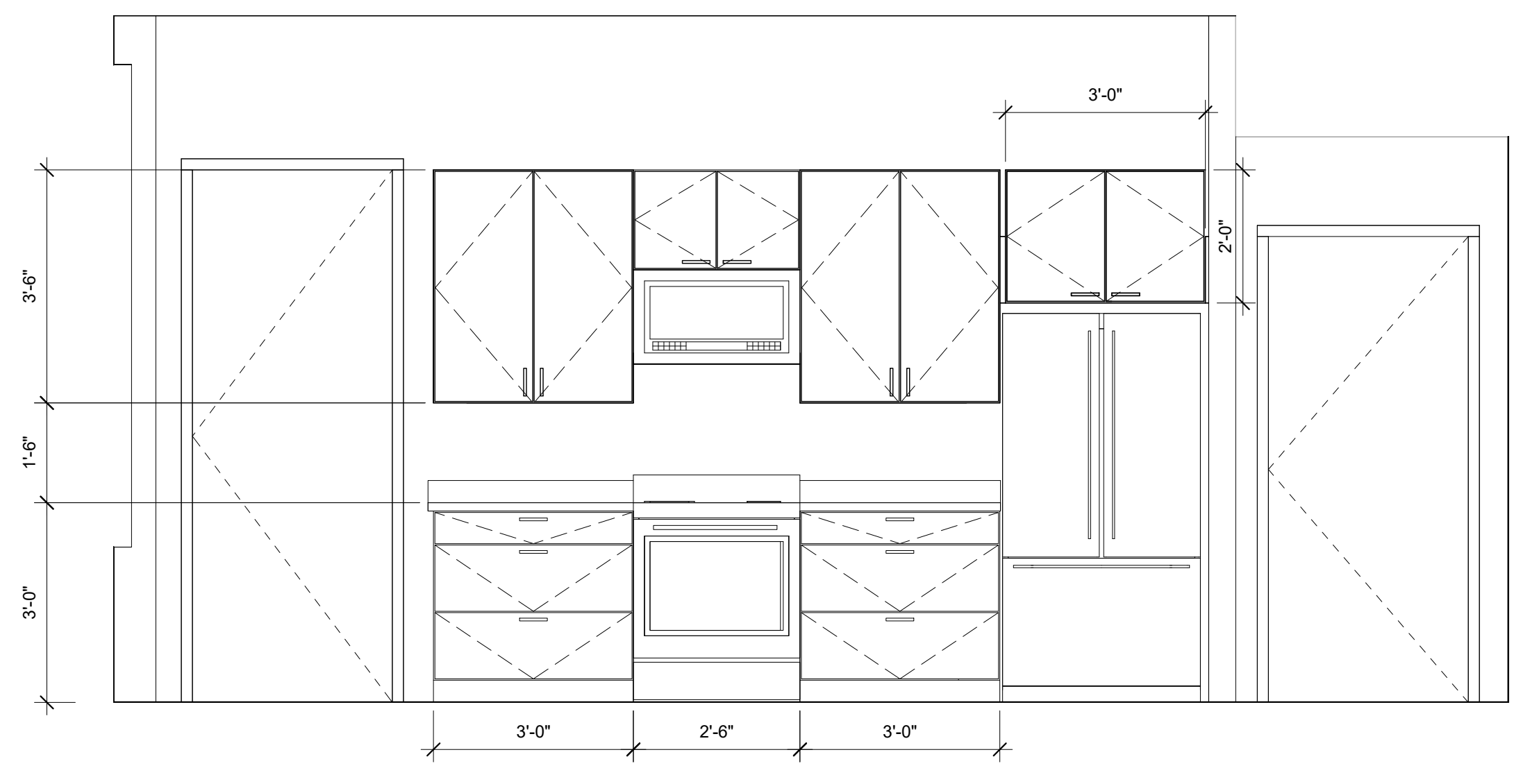
3 UNIT 401 KITCHEN ELEV. B 1/2" = 1'-0"
