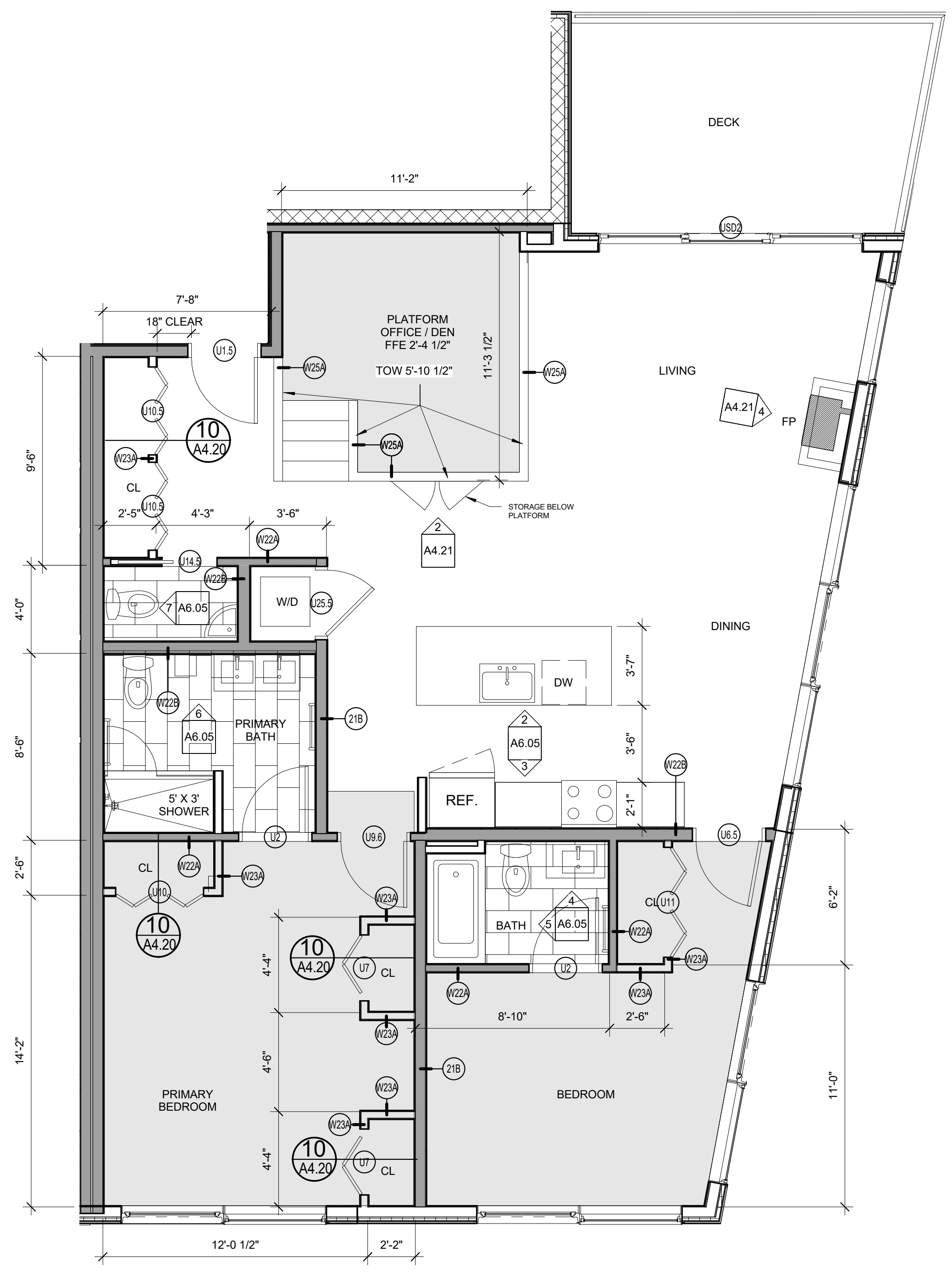
1 ENLARGED PLAN - UNIT 401 1/4" = 1'-0"
