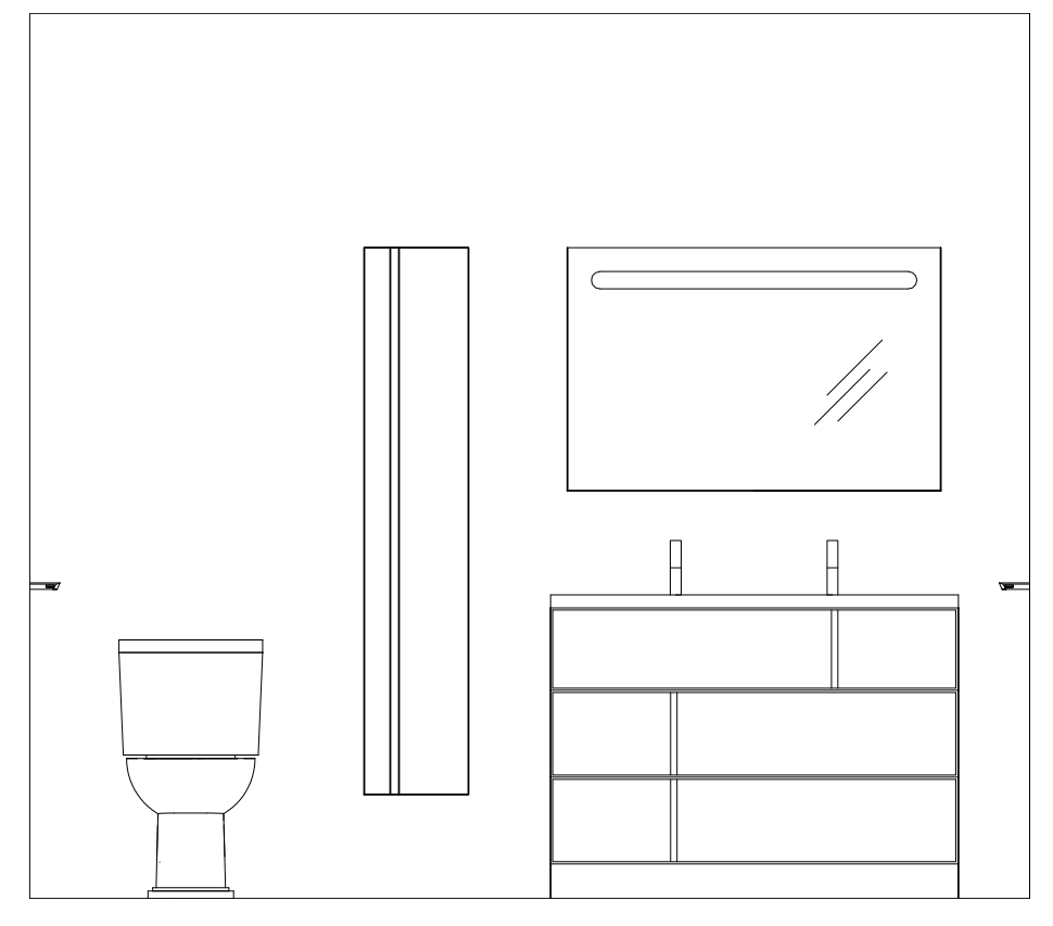
6 UNIT 401 BATH 2 ELEV. A 1/2" = 1'-0"
