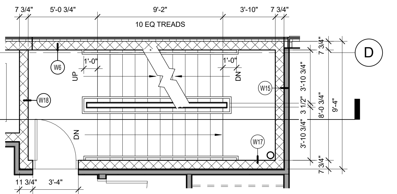
3 STAIR A - 2ND FLOOR 1/4" = 1'-0"
