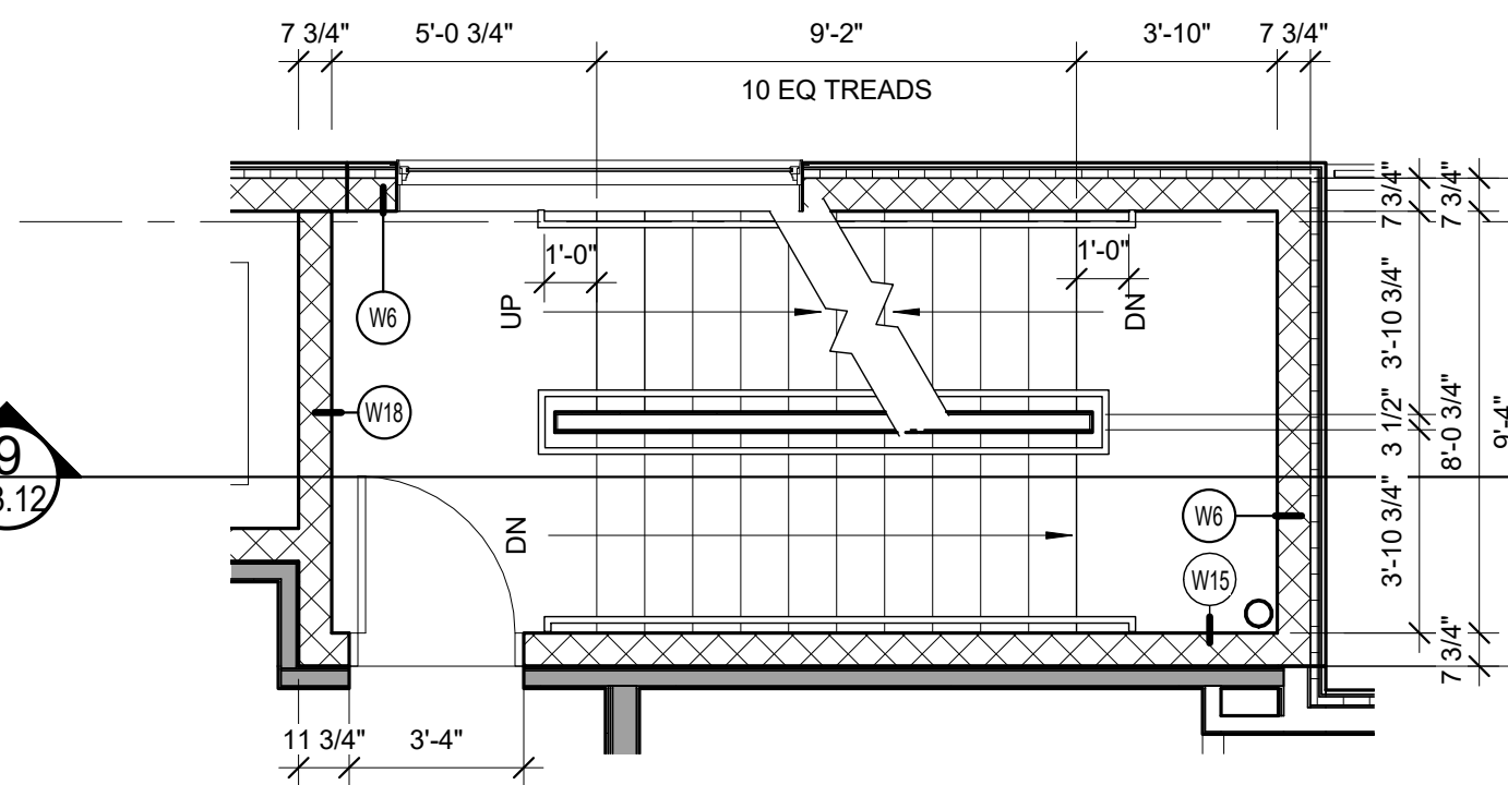
6 STAIR A - 5TH FLOOR 1/4" = 1'-0"
