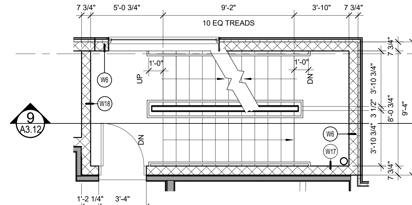
6 STAIR A - 5TH FLOOR 1/4" = 1'-0"
