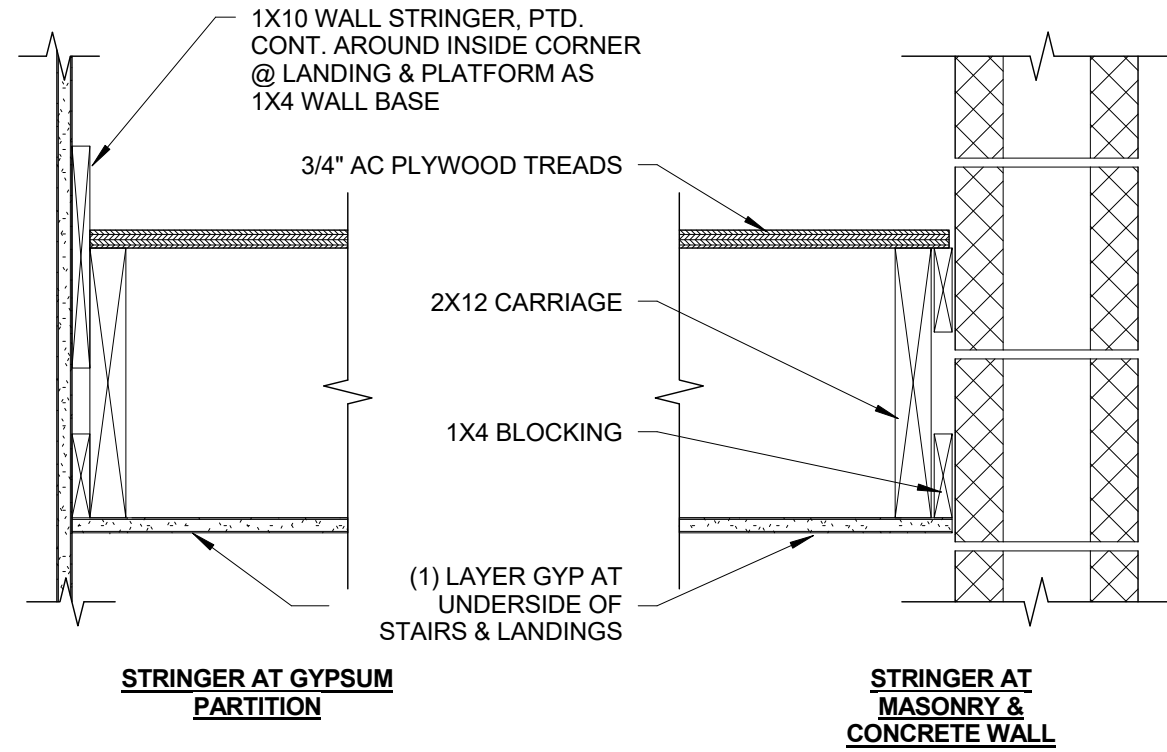
11 STAIR DETAIL - STRINGER DETAIL 1 1/2" = 1'-0"
