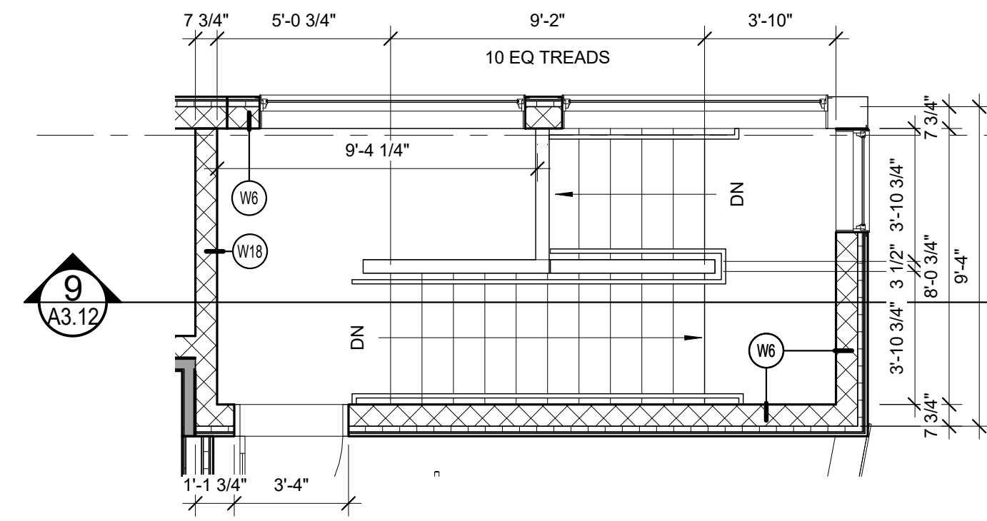
8 STAIR A - ROOF DECK 1/4" = 1'-0"
