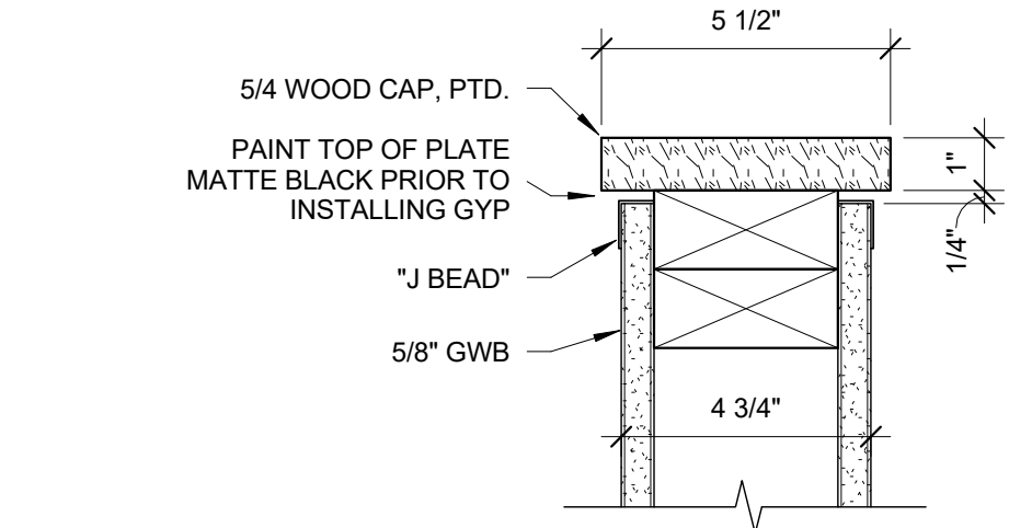
13 STAIR WALL DETAIL 3" = 1'-0"
