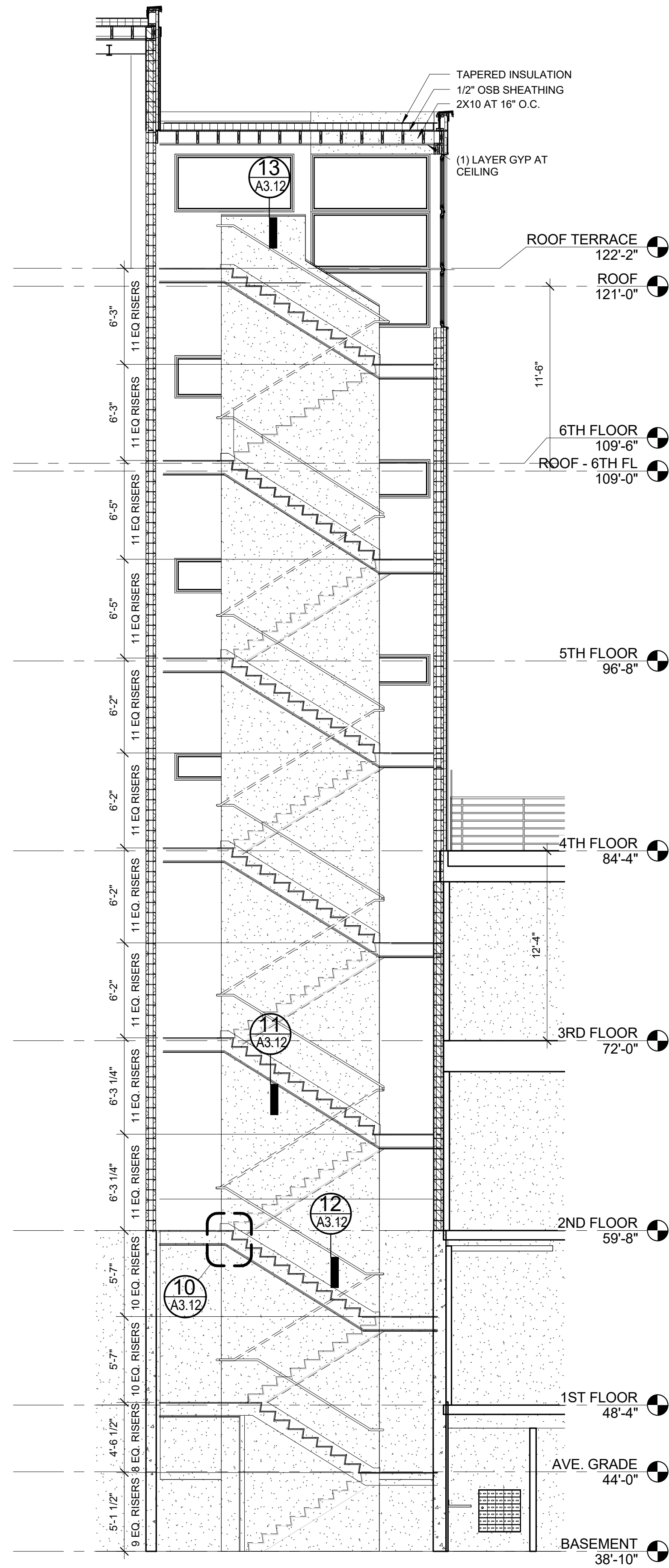
9 STAIR SECTION 3/16" = 1'-0"
