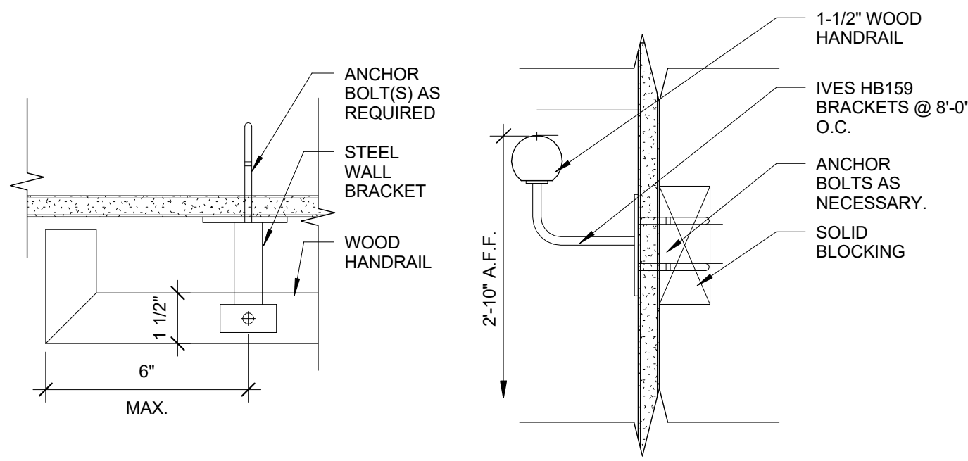
12 STAIR DETAIL - WOOD HANDRAIL 3" = 1'-0"
