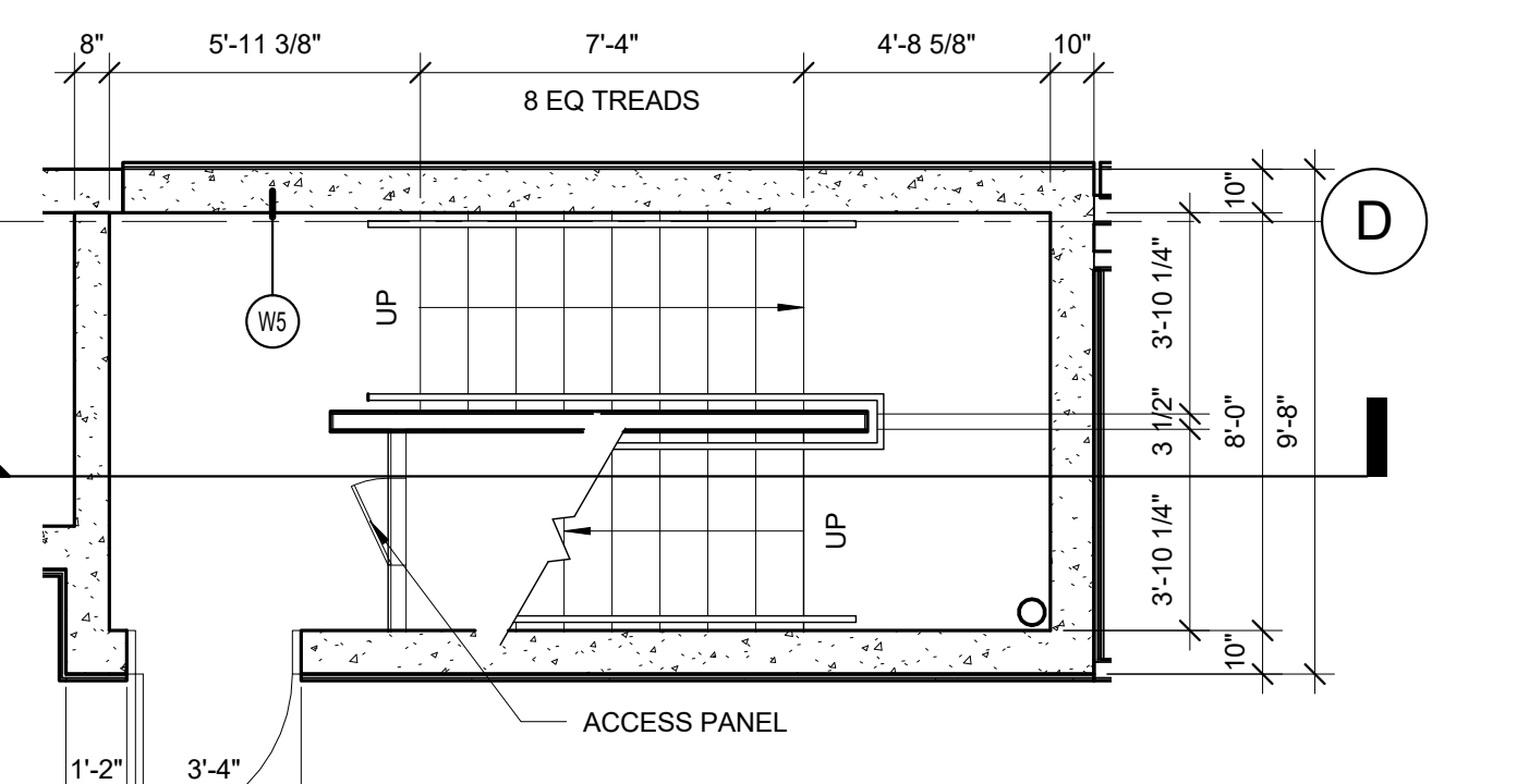
2 STAIR A - 1ST FLOOR 1/4" = 1'-0"
