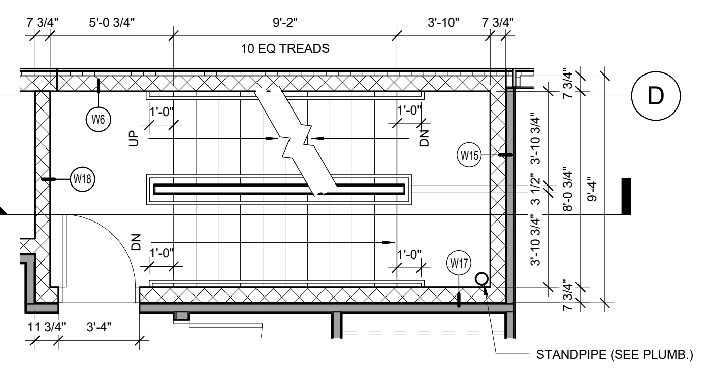
4 STAIR A - 3RD FLOOR 1/4" = 1'-0"
