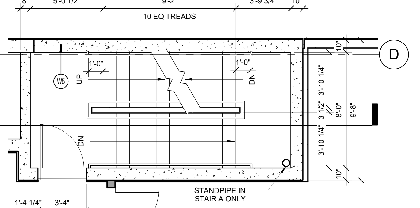
2 STAIR A - 1ST FLOOR 1/4" = 1'-0"
