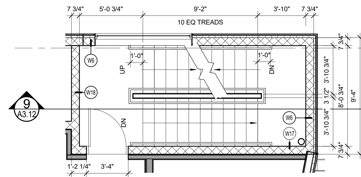
7 STAIR A - 6TH FLOOR 1/4" = 1'-0"
