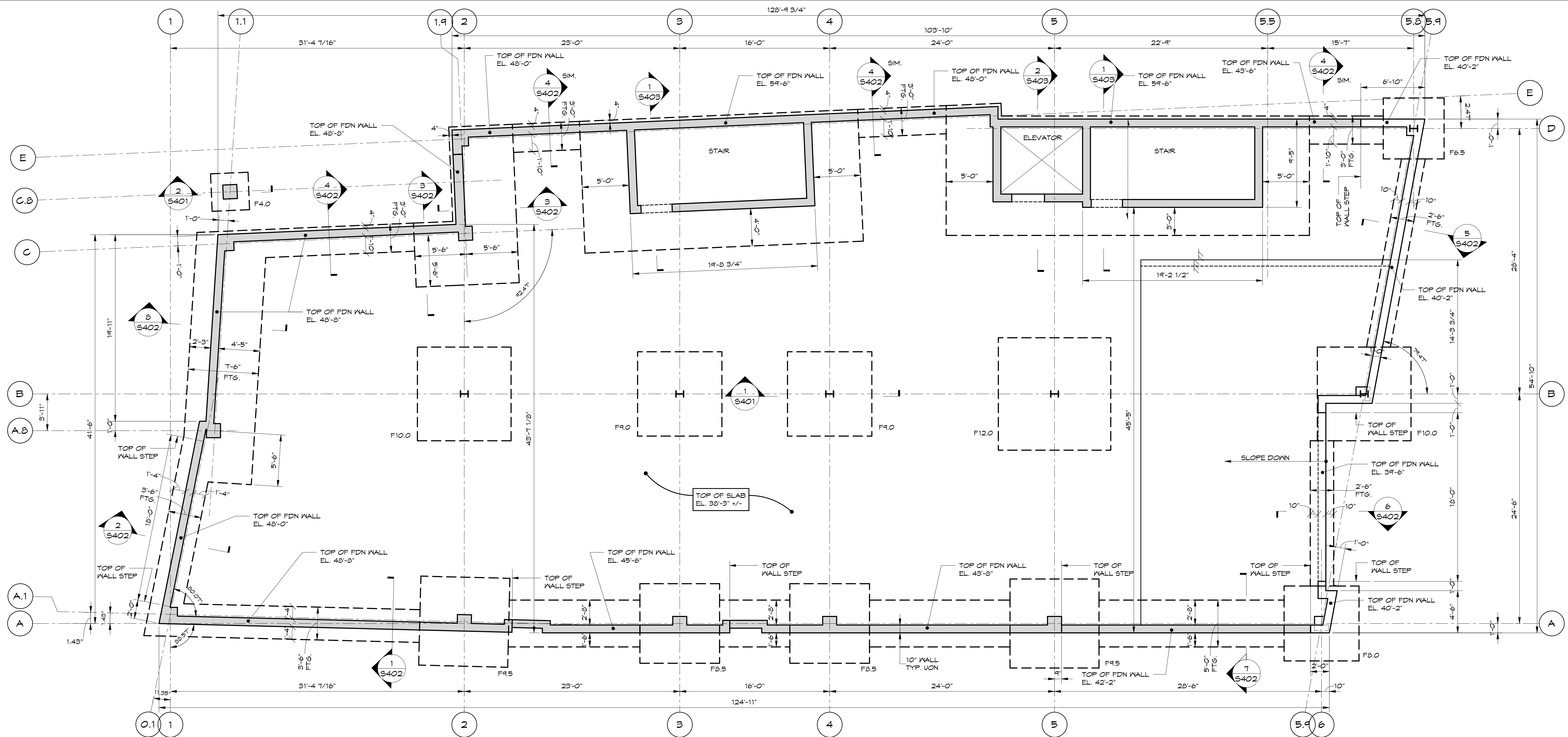
1 FOUNDATION PLAN (BASEMENT LEVEL) 3/16" = 1'-0"
