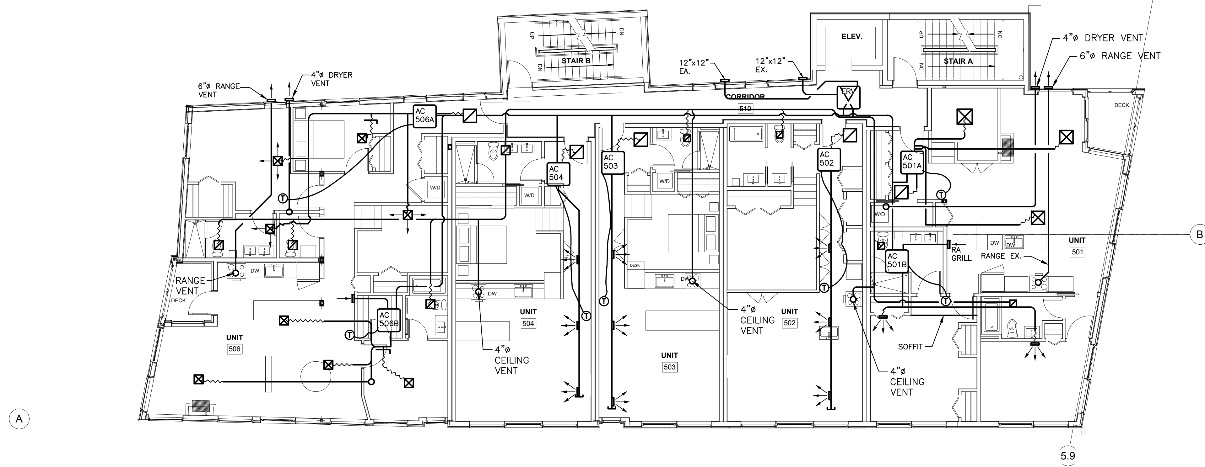
5TH FLOOR - DUCTWORK SCALE: 1/8"=1'-0"
