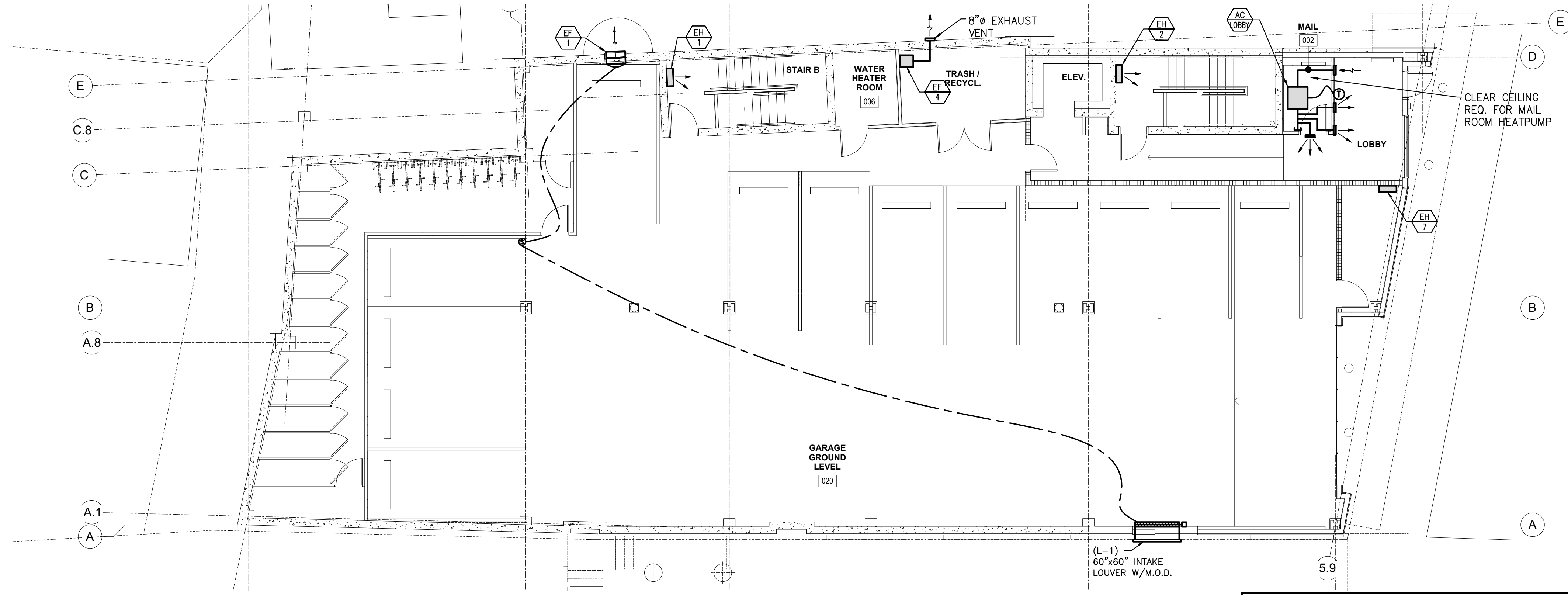
BASEMENT FLOOR – DUCTWORK SCALE: 1/8"=1'-0"
