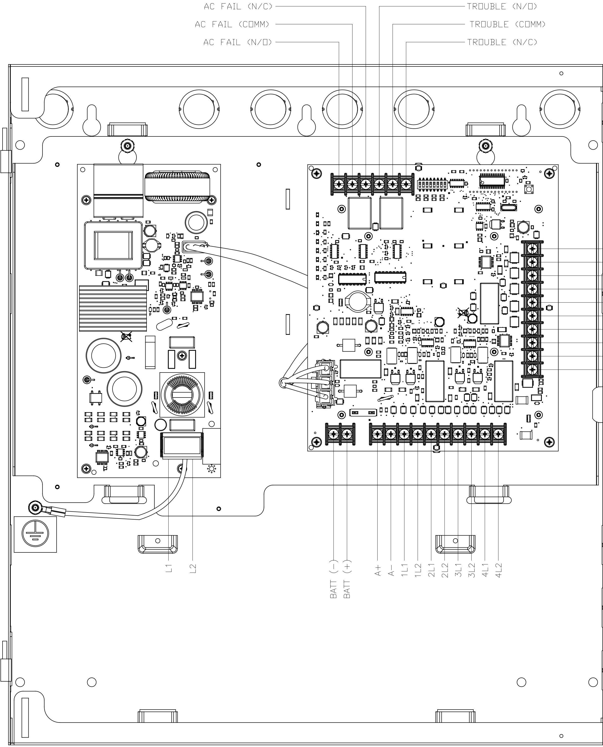
HPFF8 Remote Booster Panel Panel Wiring Diagram
