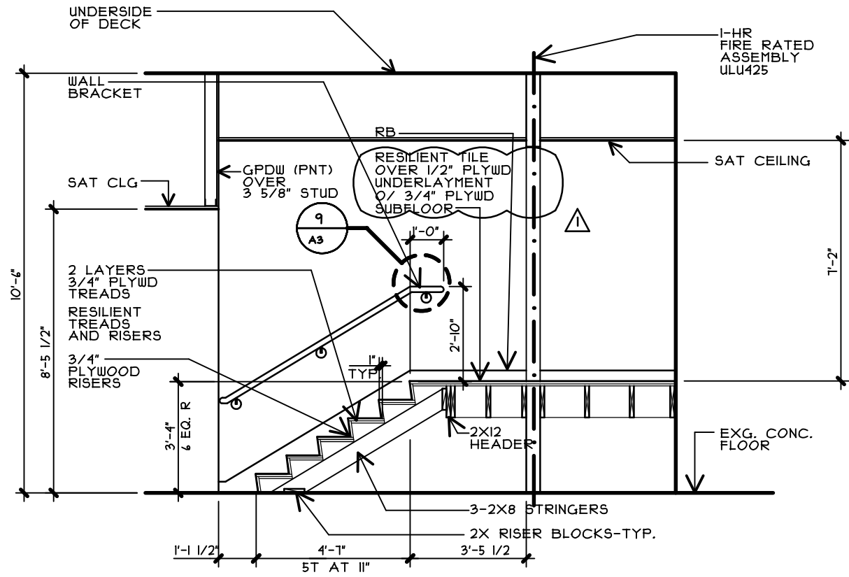
(A) SECTION
