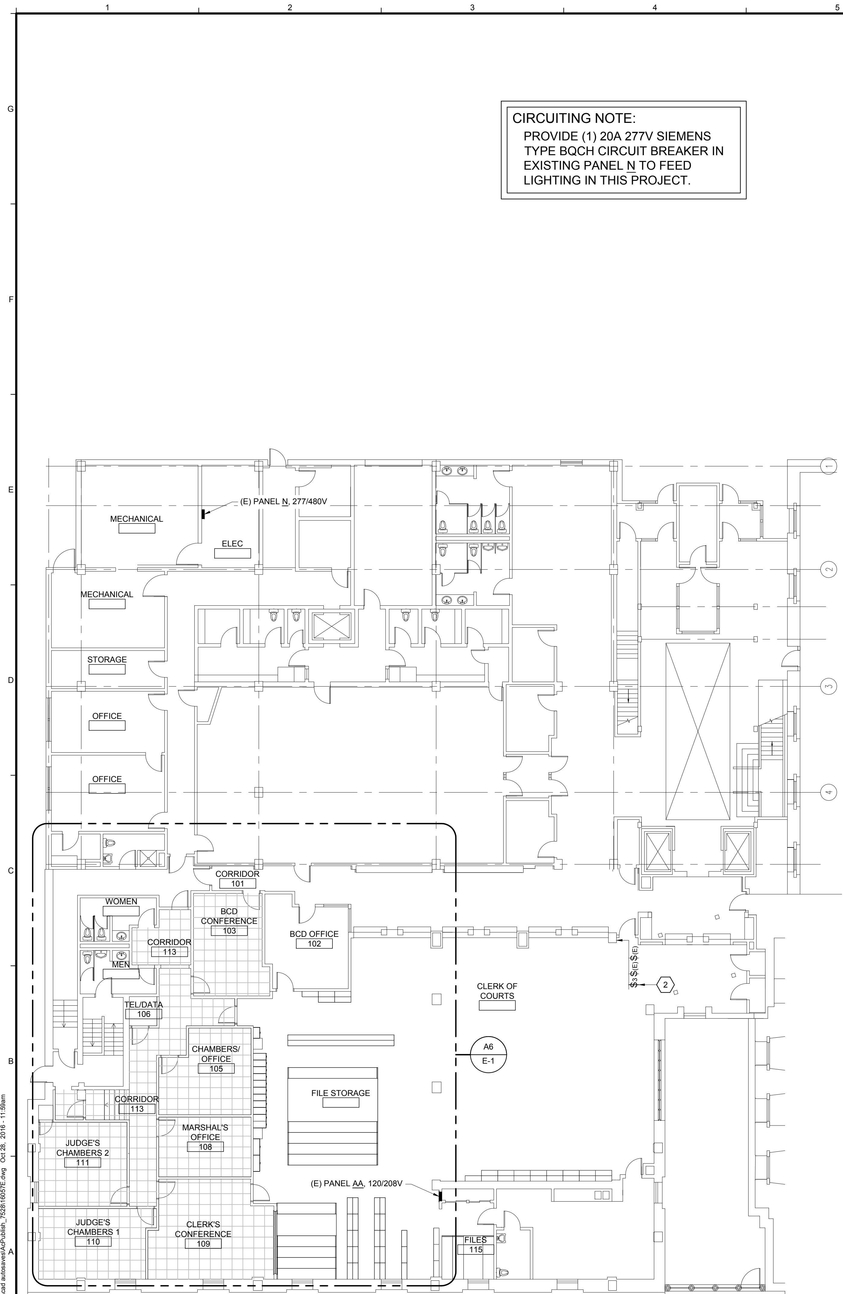
A1 FLOOR PLAN 3/32"=1'-0"
