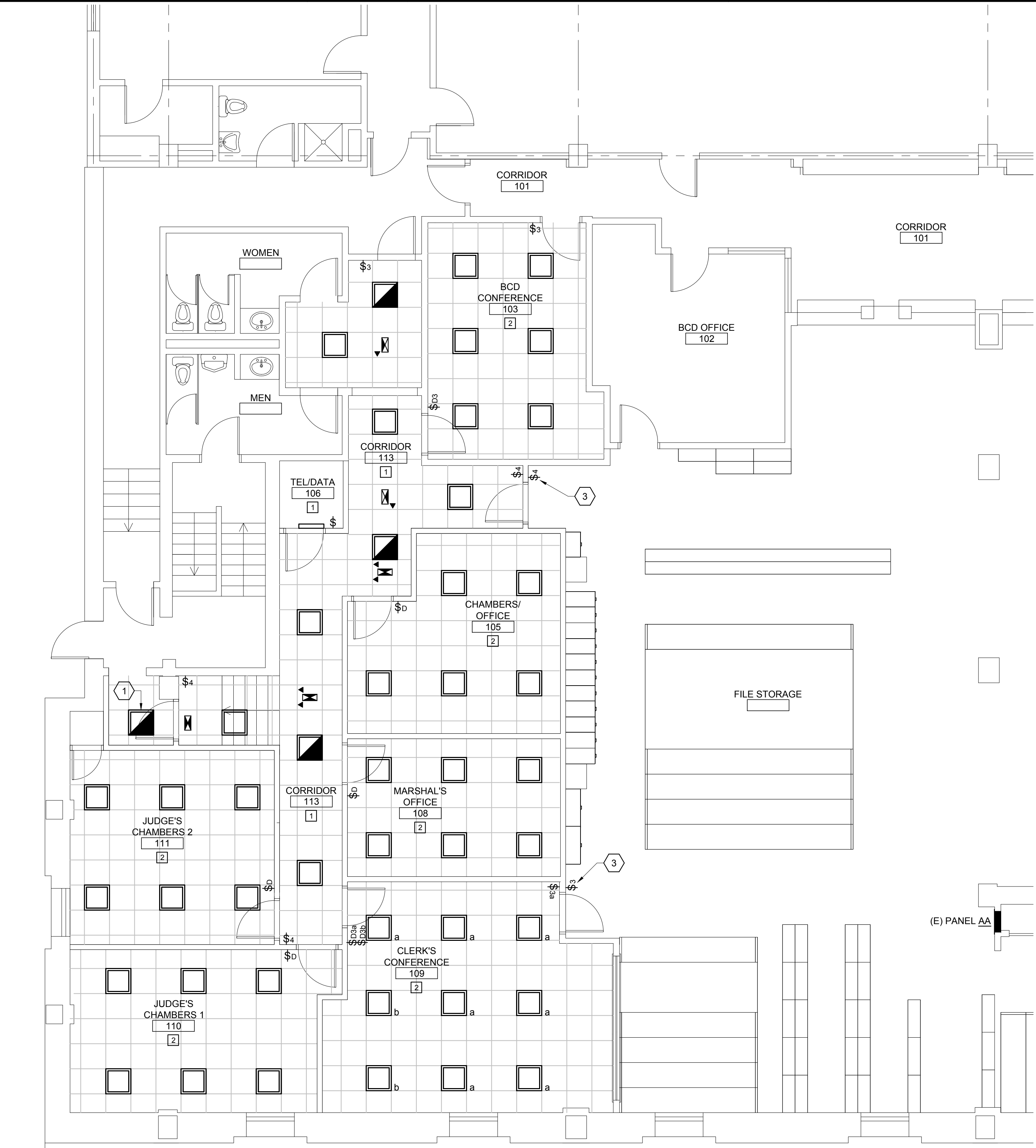
A6 ENLARGED FLOOR PLAN- LIGHTING 1/4"=1'-0"
