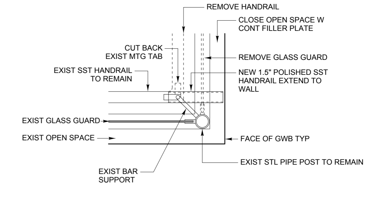
4 HANDRAIL PLAN DETAIL 1 1/2" = 1' - 0"
