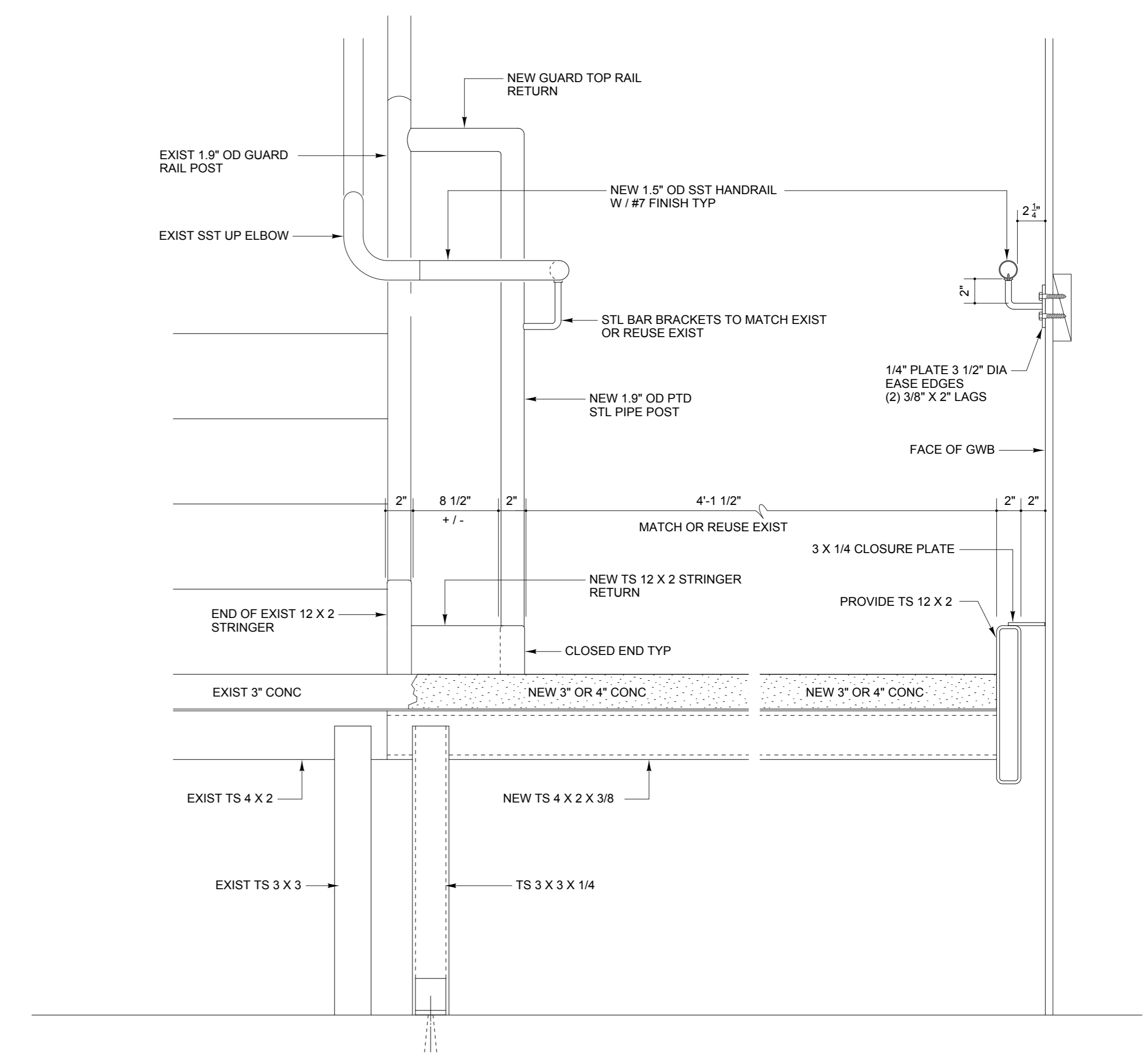
2 STAIR SECTION DETAIL 1 1/2" = 1' - 0"
