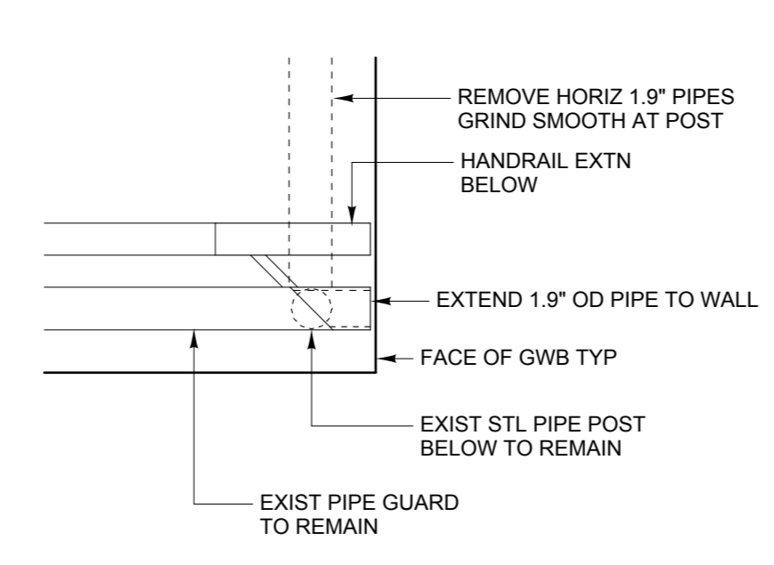
3 GUARDRAIL PLAN DETAIL 1 1/2" = 1' - 0"
